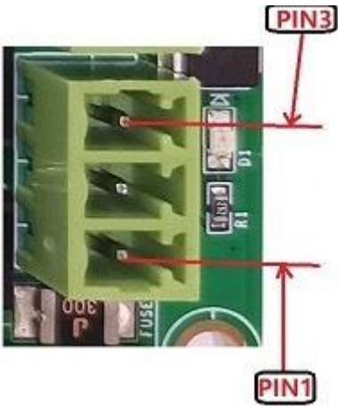
Figure 893: Power Input
