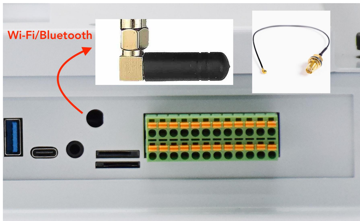
WiFi+BT Antenna
