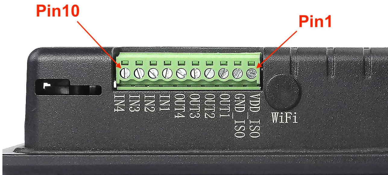
GPIO Terminal (enclosed PC version)
