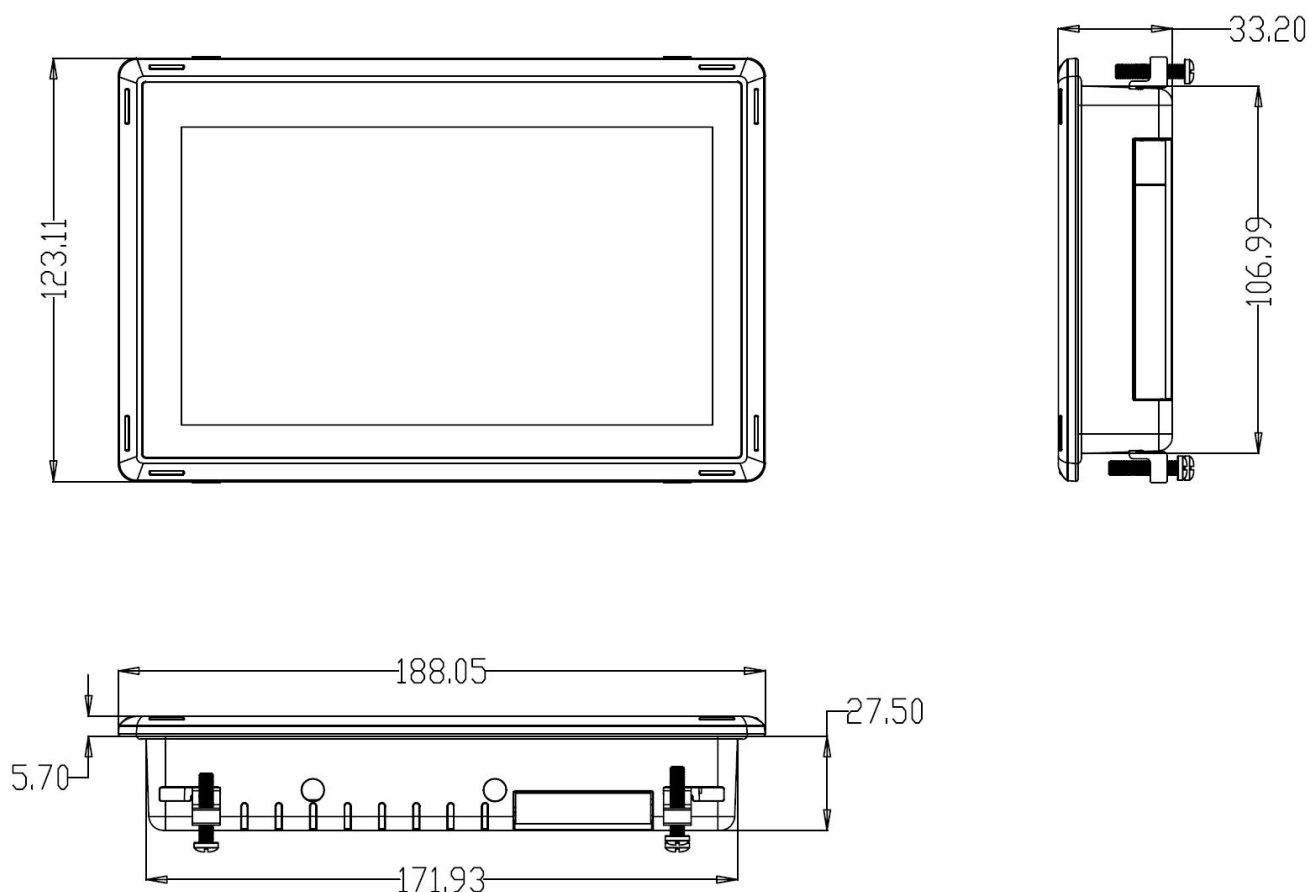
Figure 612: PPC-A55-070 Technical Drawing
