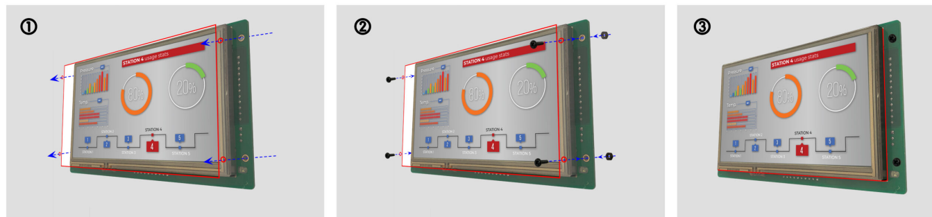
Figure 896: Embedded mounting
