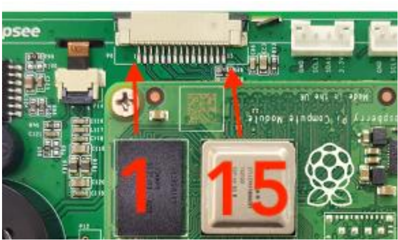
Camera Connector
