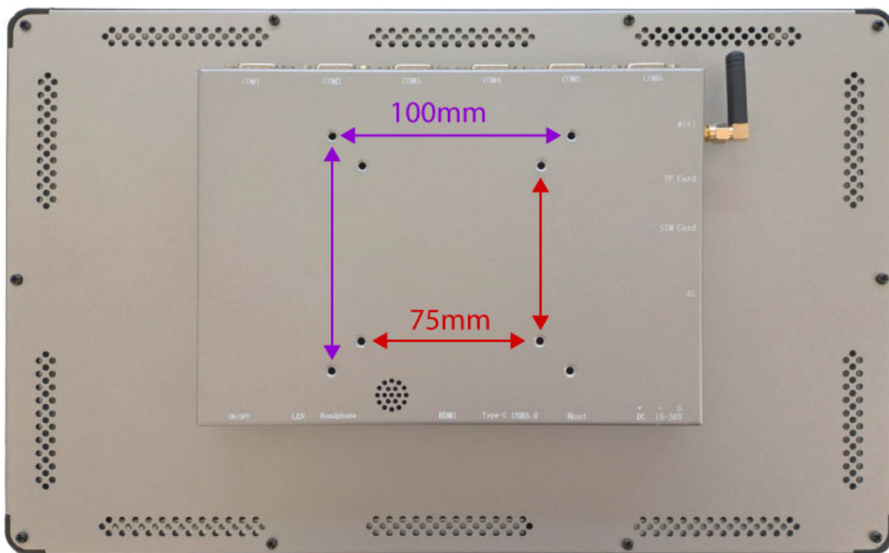
Figure 585: Mounting Method
