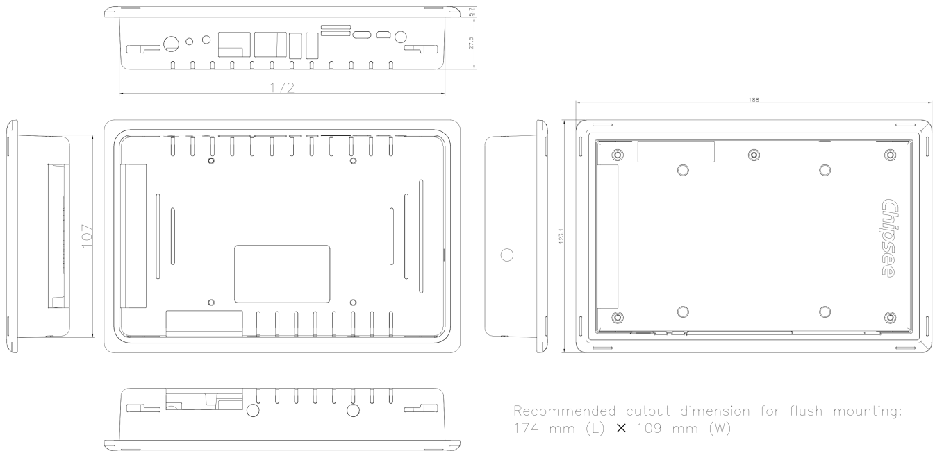
Figure 612: PPC-A55-070 Technical Drawing
