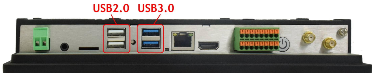
USB HOST Ports
