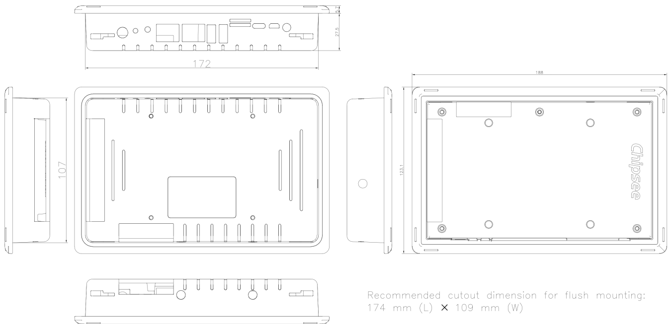
Technical Drawing (PPC-RK3576-070)
