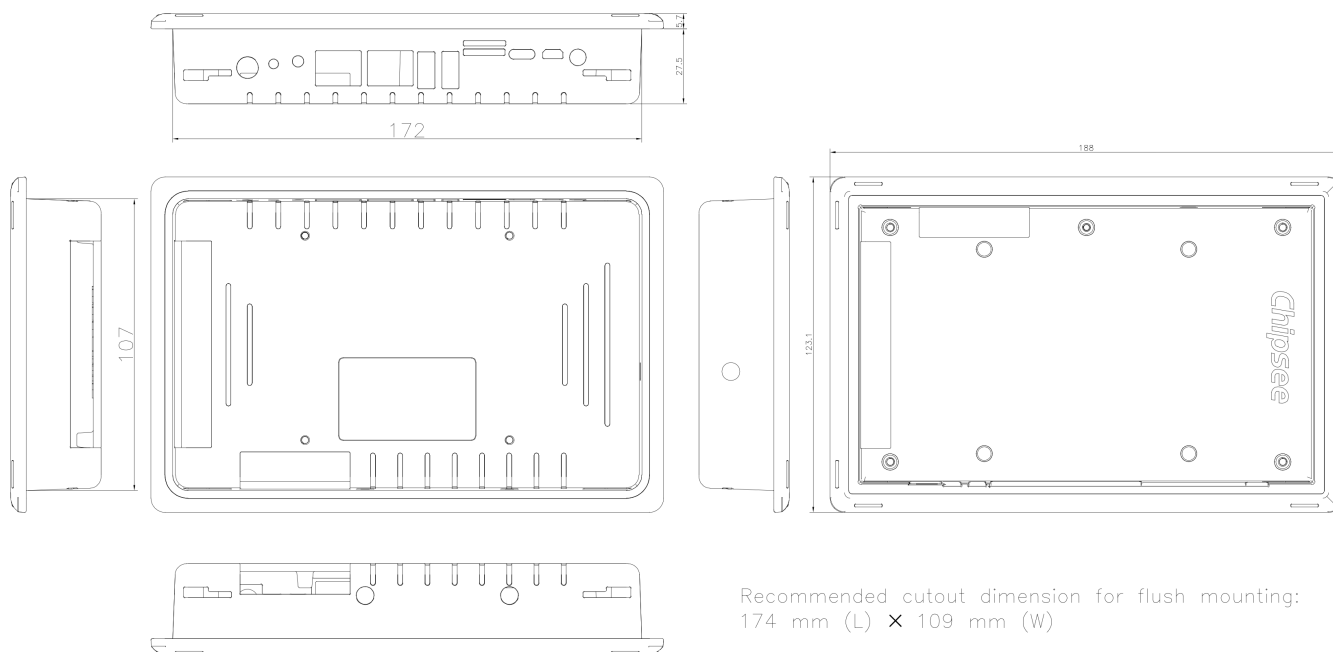
PPC-A76-070 Technical Drawing
