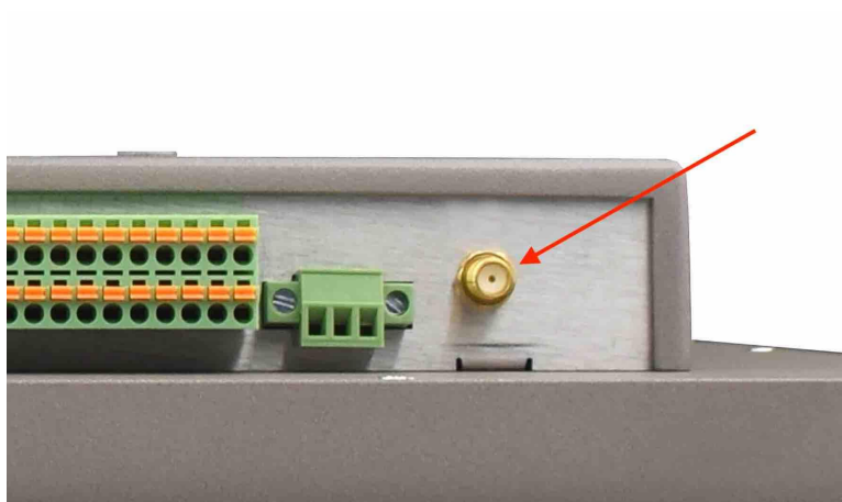
WiFi+BT Antenna
