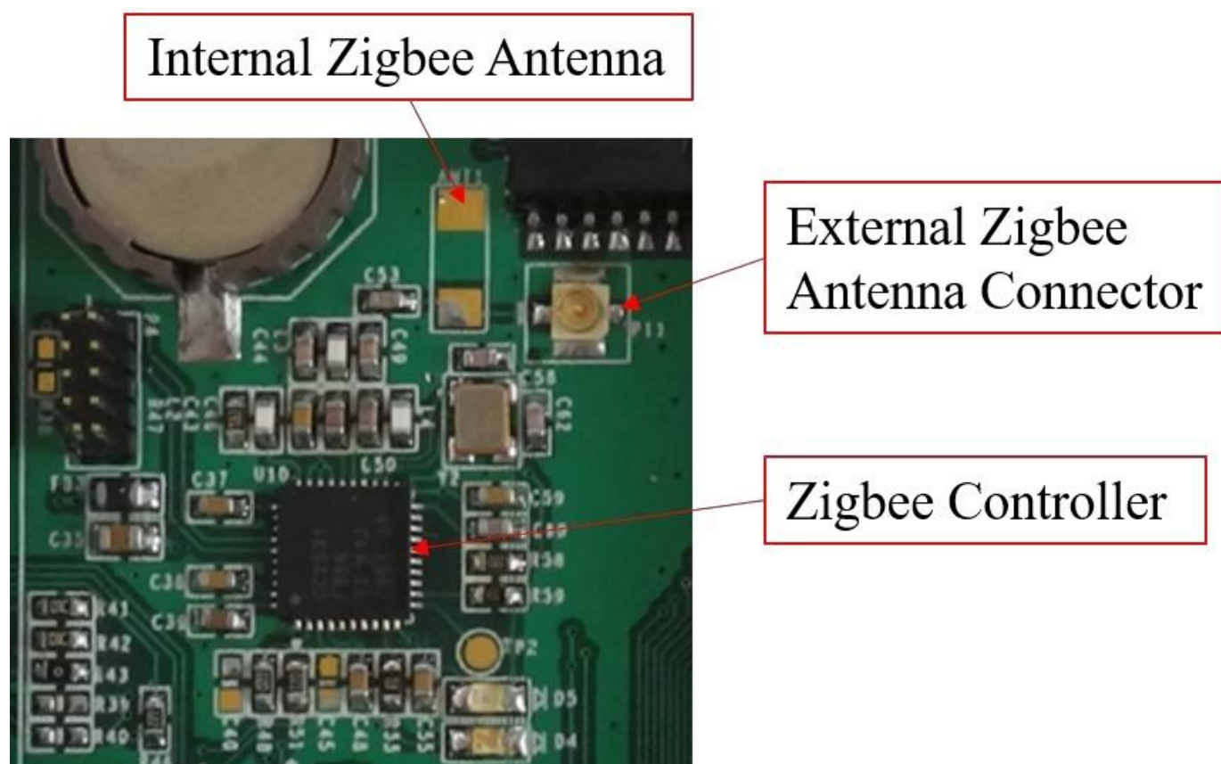
Figure 923: Zigbee controller
