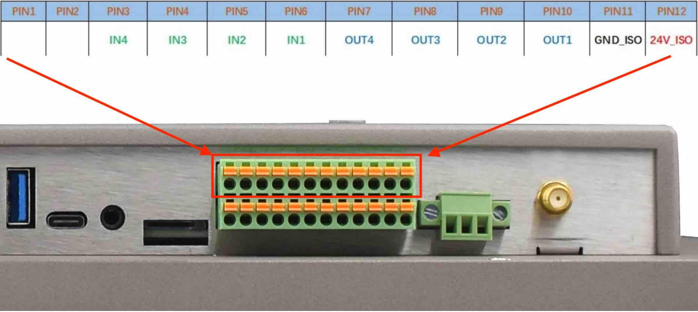
GPIO Connector
