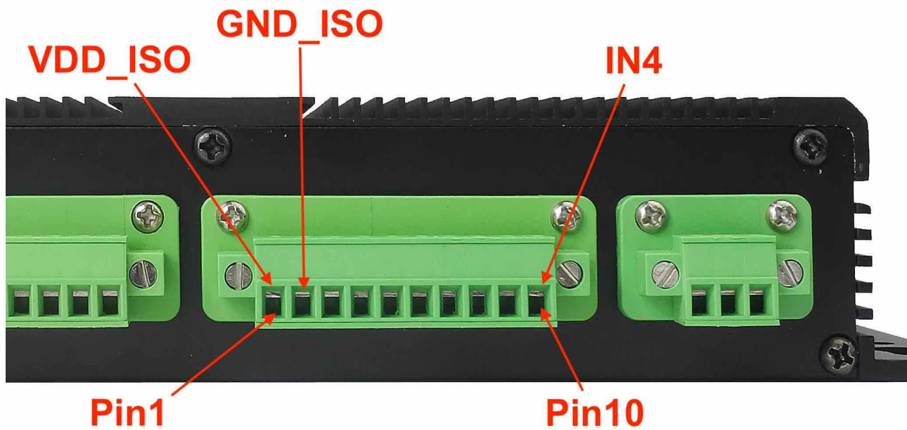
GPIO Terminal
