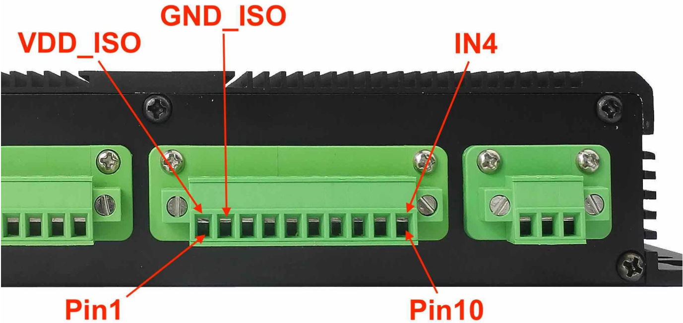
GPIO Connector
