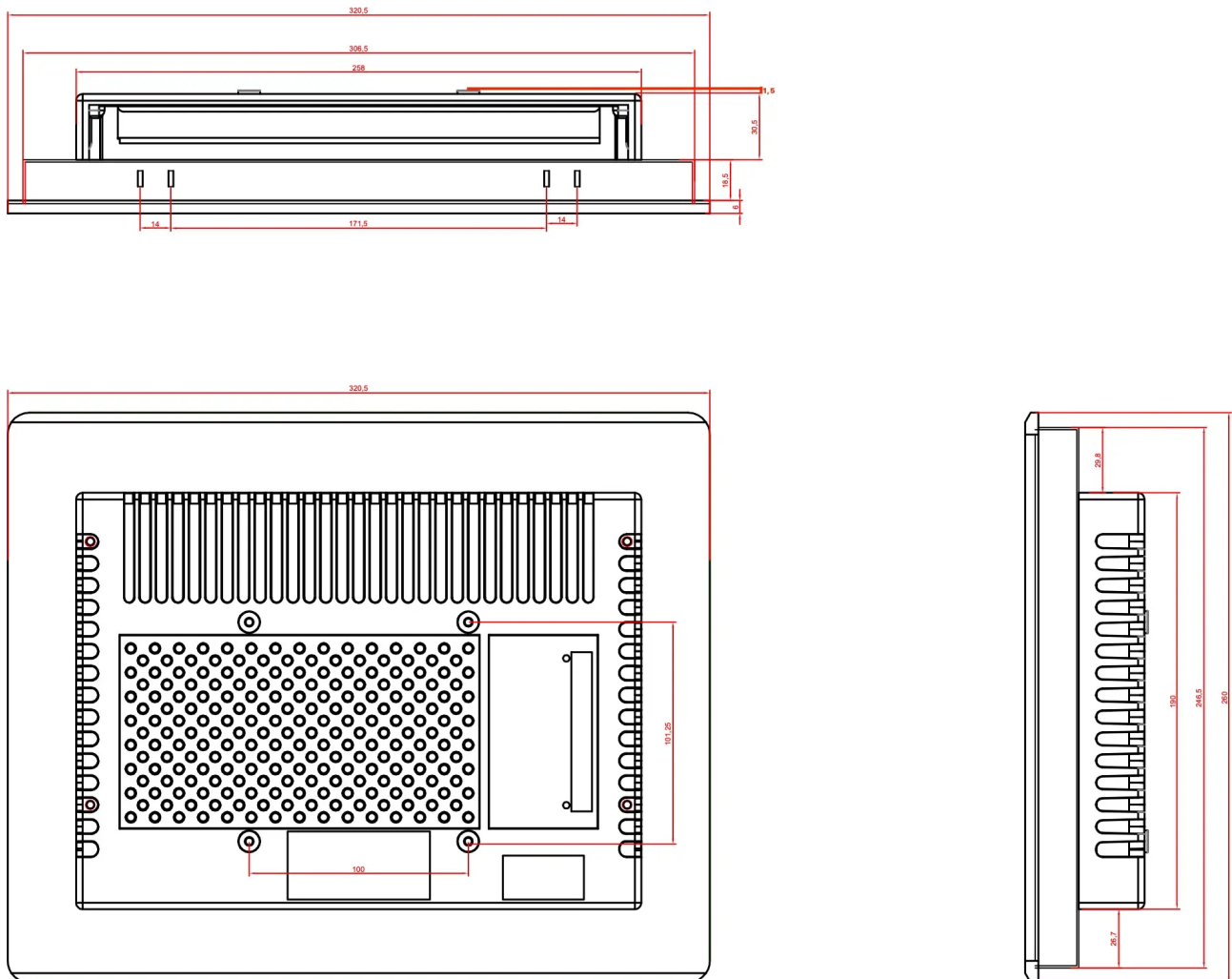
Figure 917: CS10768RA4121P Technical Drawing
