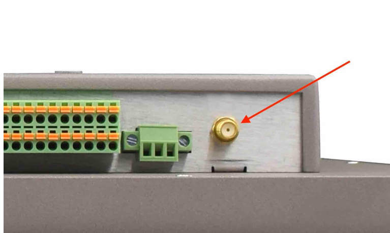
WiFi+BT Antenna
