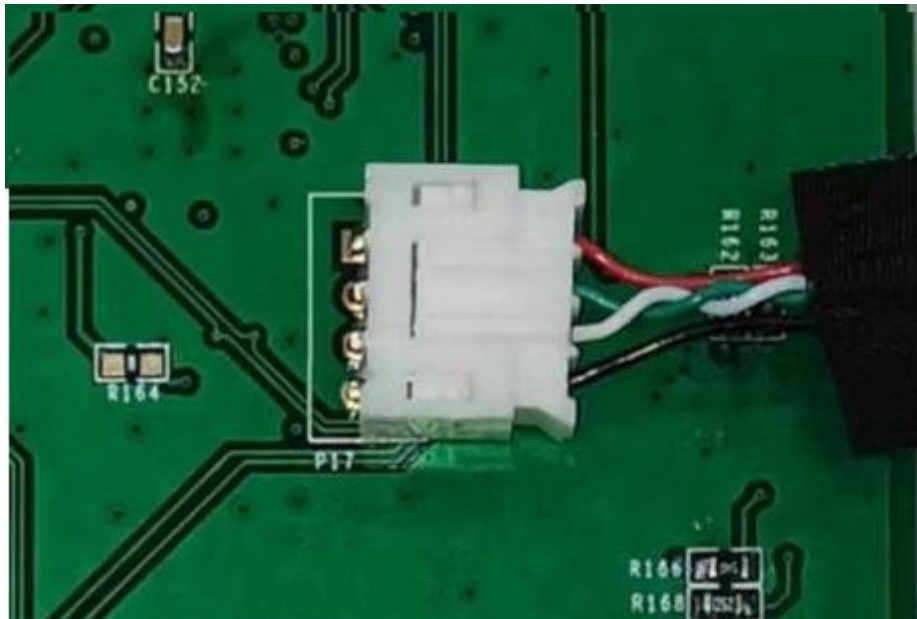
Figure 508: Capacitive Touch Screen Connector
