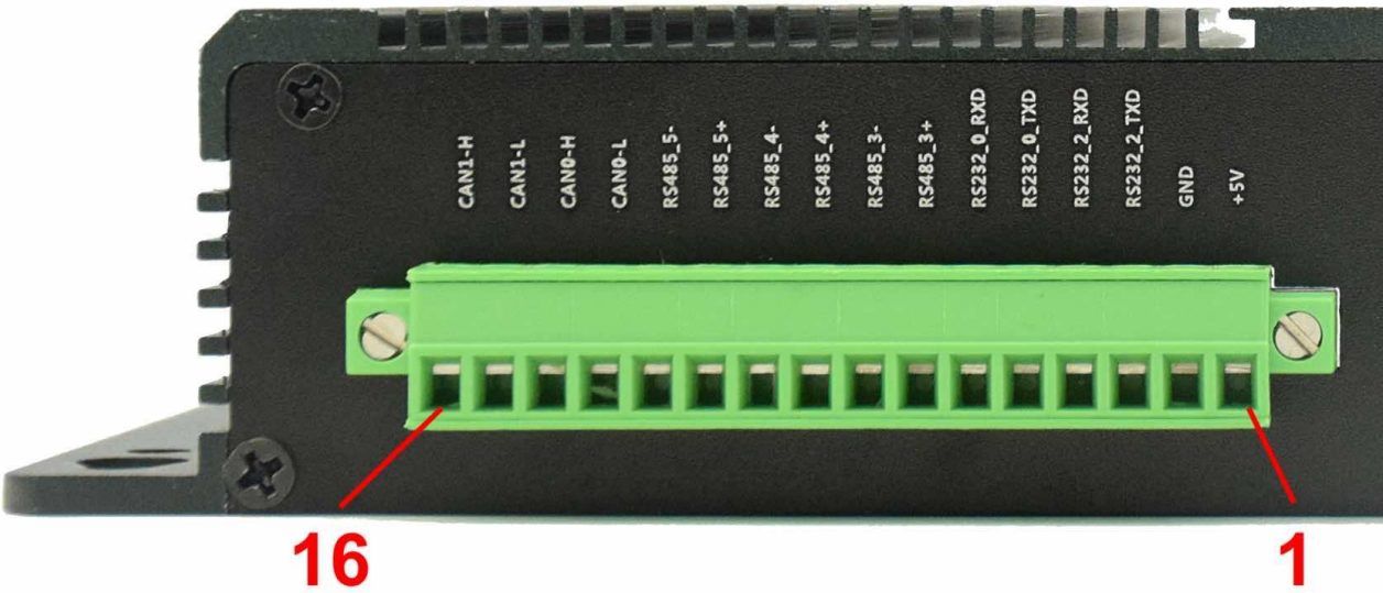
RS232 RS485 CAN Pins
