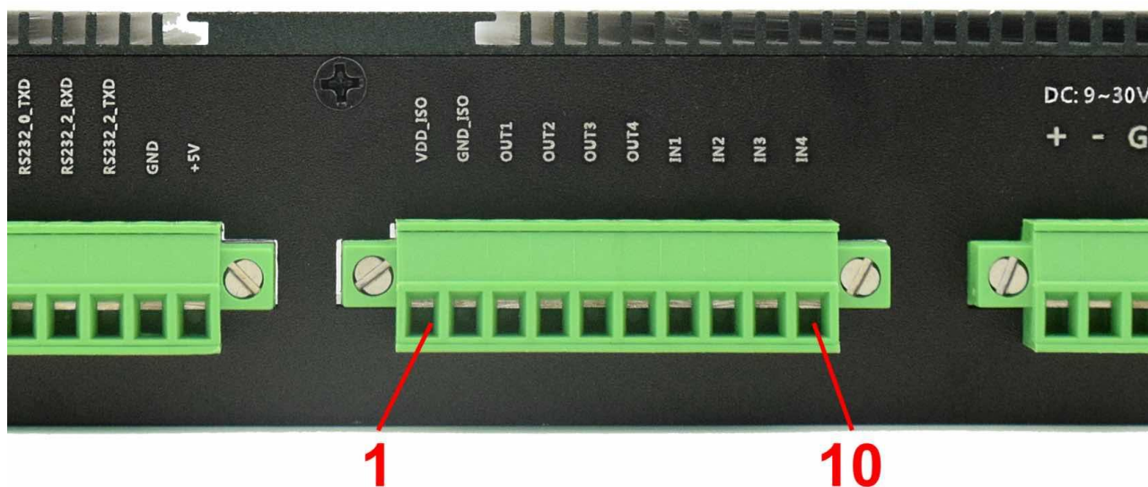
GPIO Terminal (enclosed PC version)
