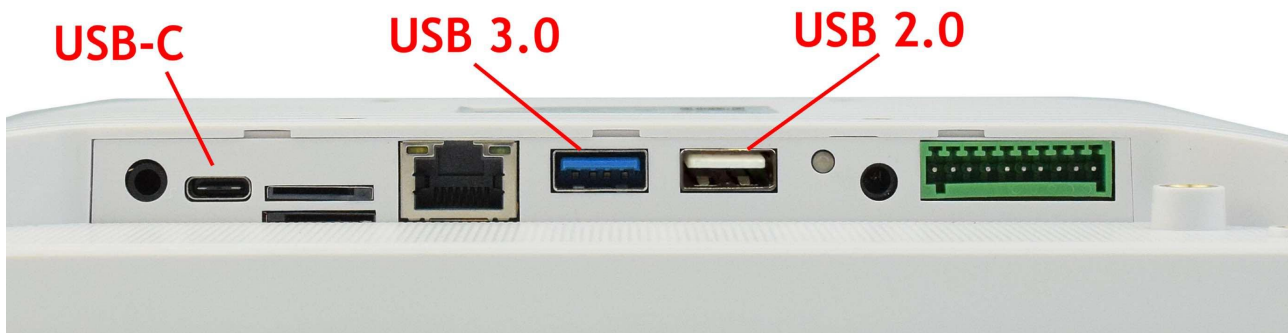
USB3.0 HOST and Type-C Connectors
