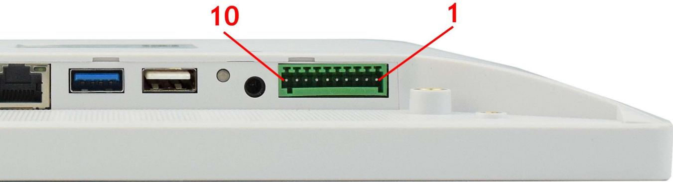
RS232/RS485/Relay Connector
