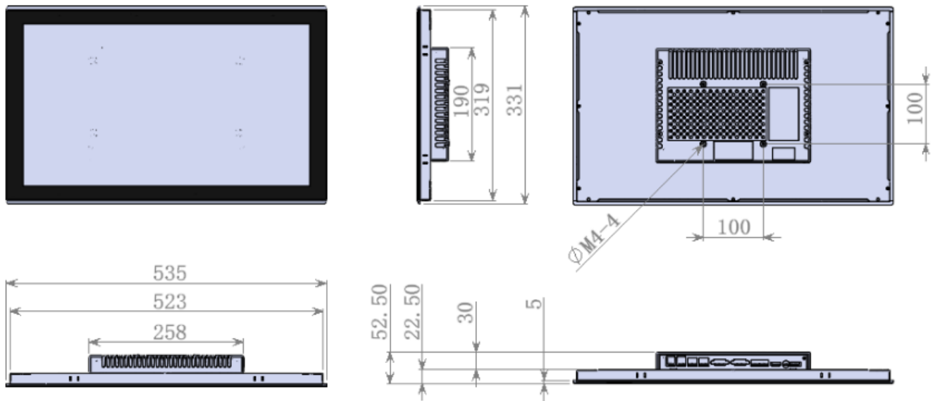
Dimensions (PPC-RK3576-215)
