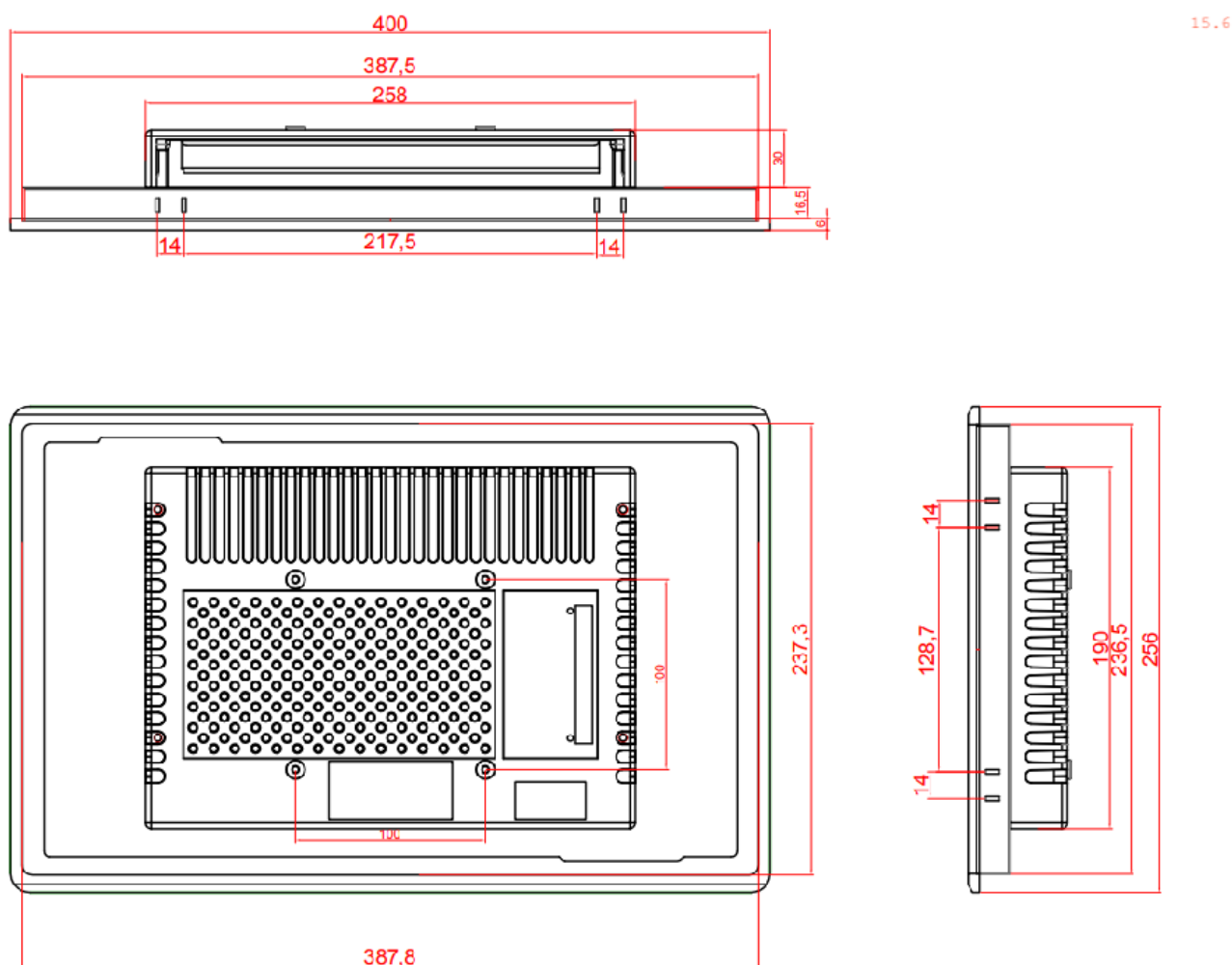
Figure 1024: Technical Drawing
