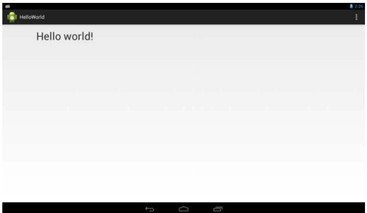
Figure 797: HelloWorld Program
