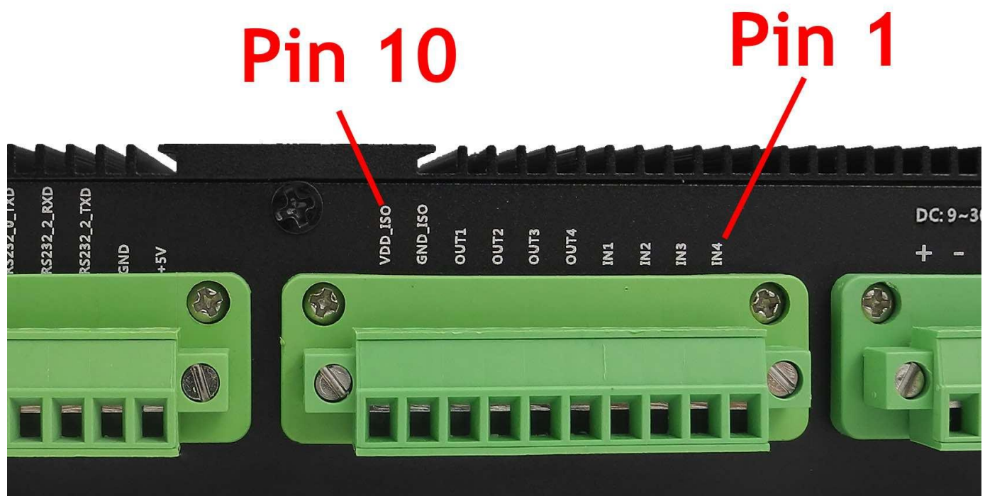
GPIO Terminal
