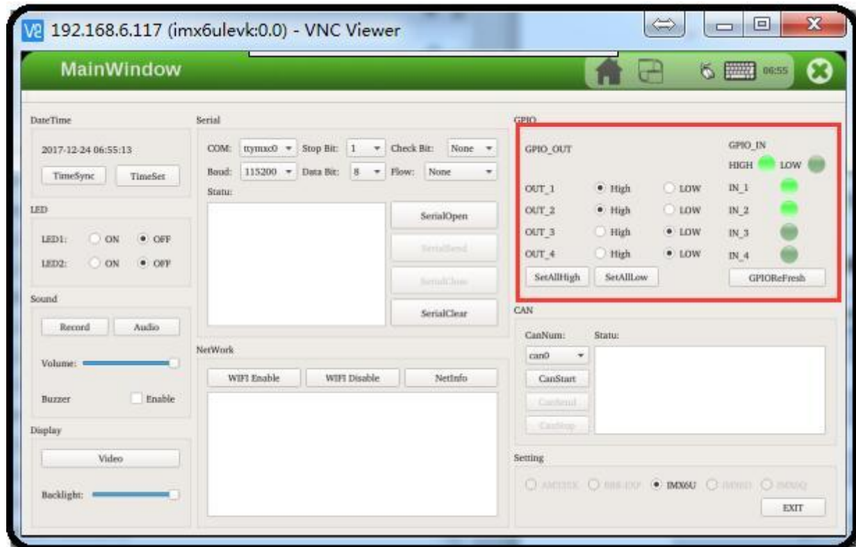
Figure 247: GPIO Test
