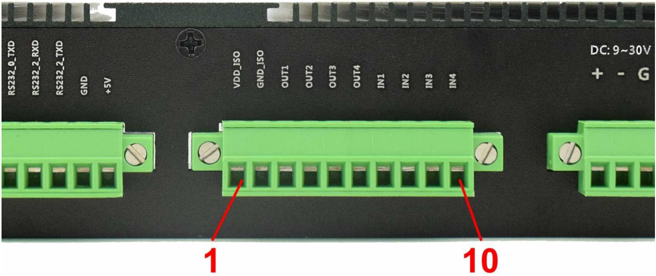
GPIO Terminal
