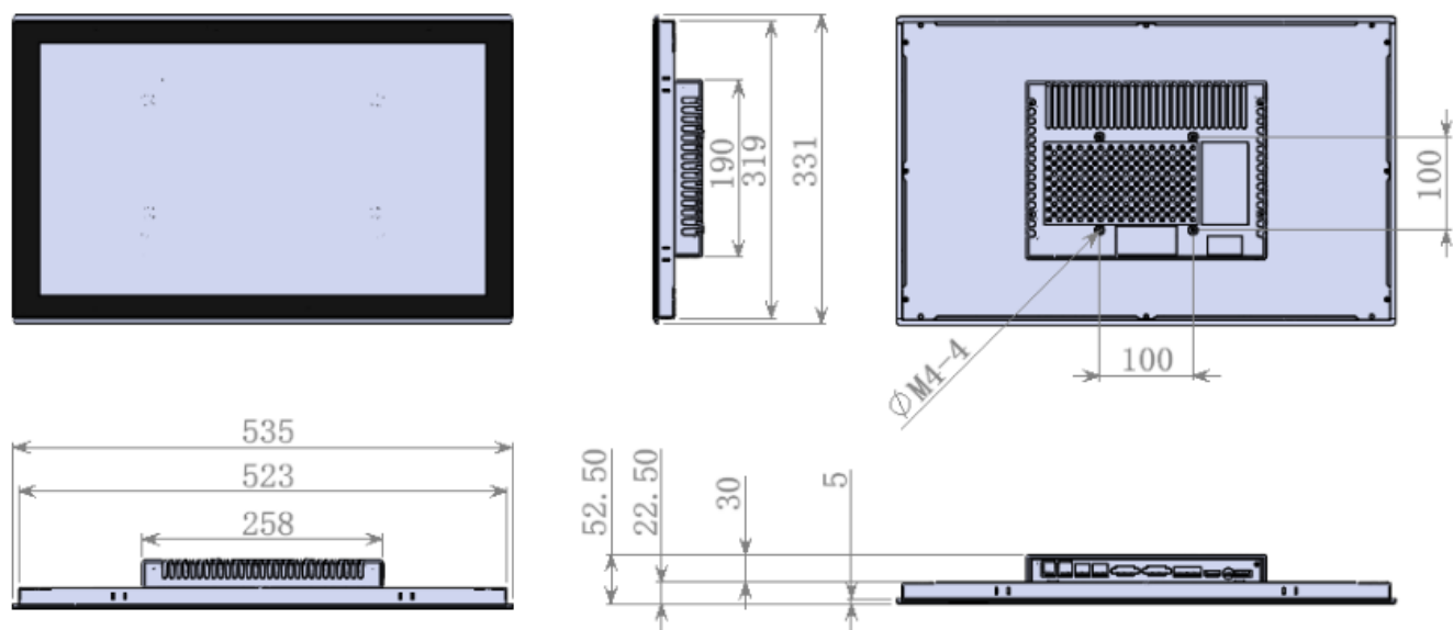
Technical Drawing
