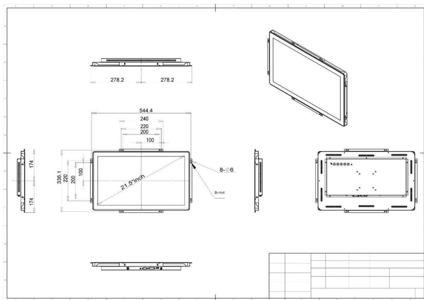
Figure 1028: Technical Drawing
