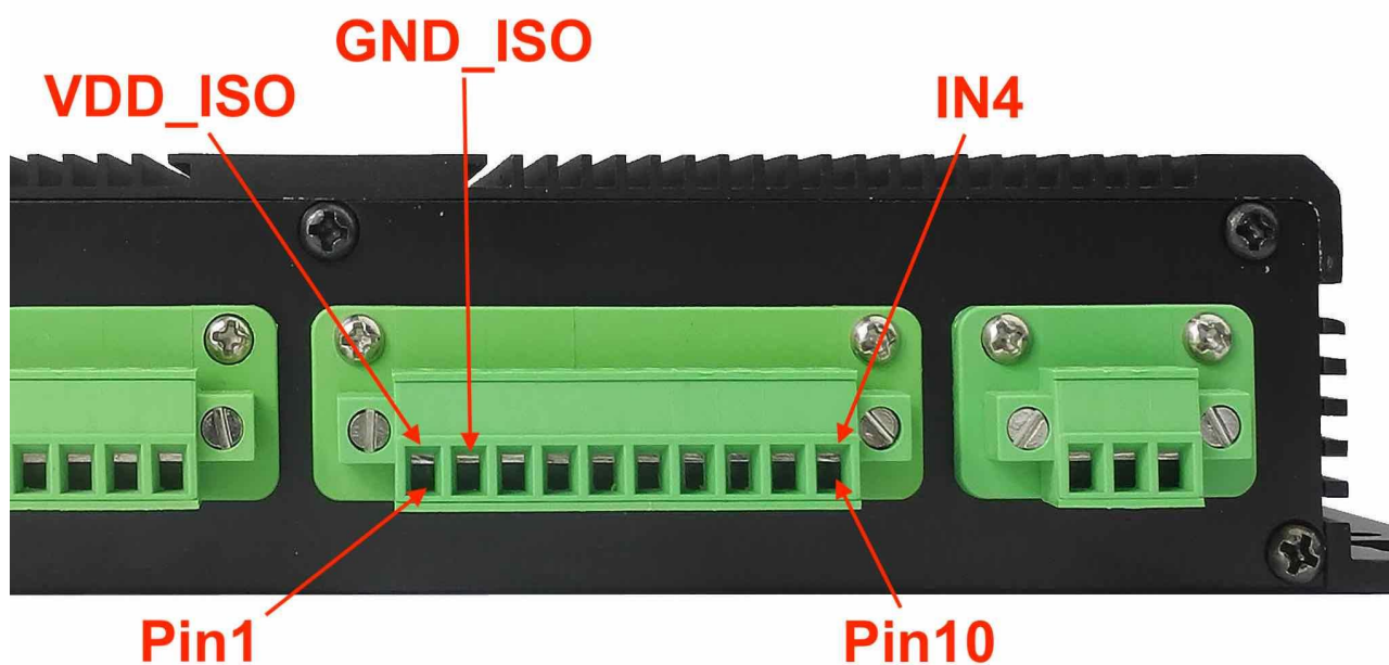
GPIO Terminal
