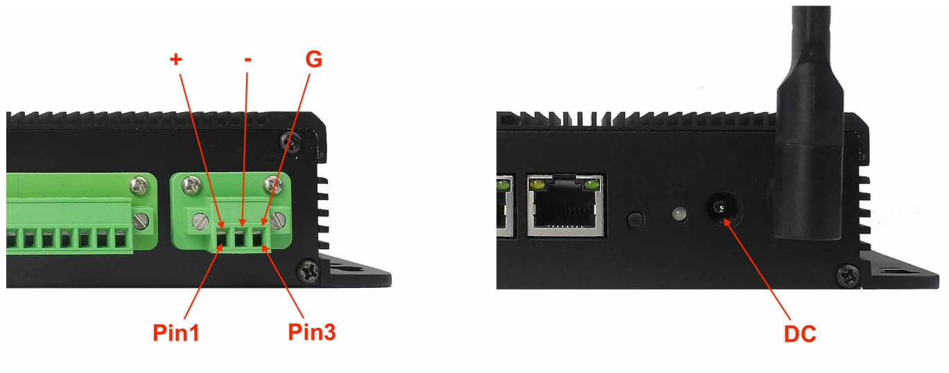
Power Input
