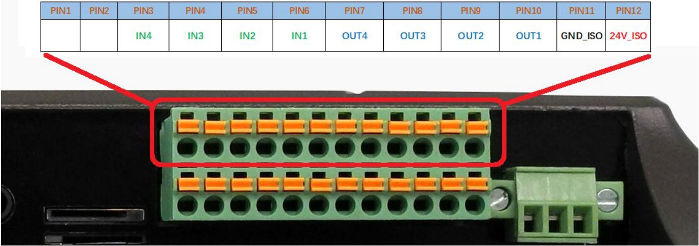
GPIO Connector
