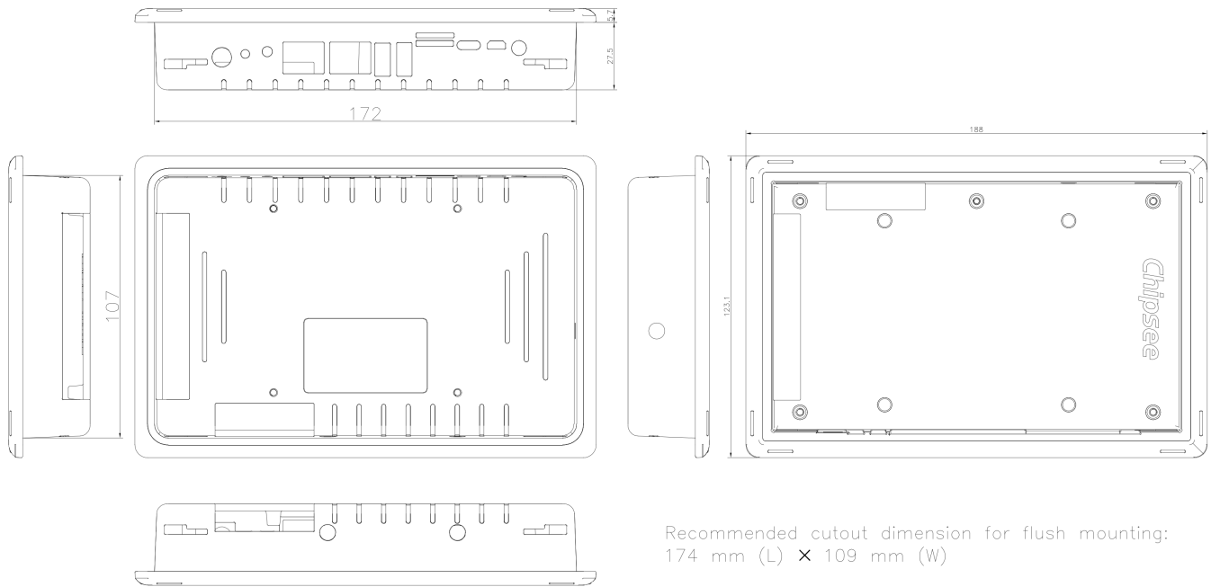
Figure 910: CS10600RA4070P-D Technical Drawing
