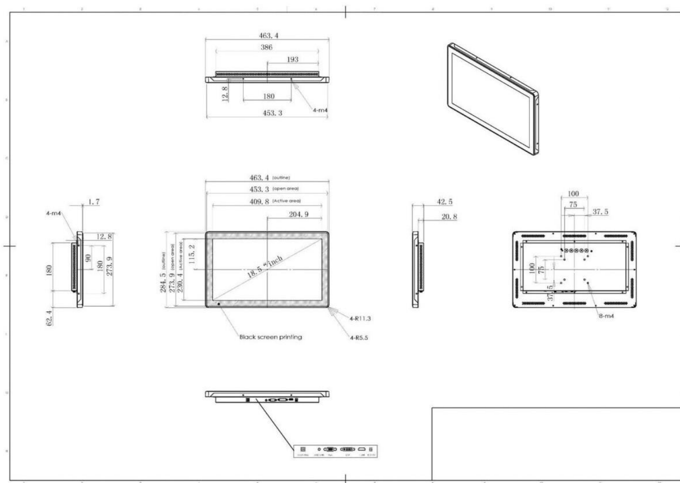
Figure 1026: Technical Drawing
