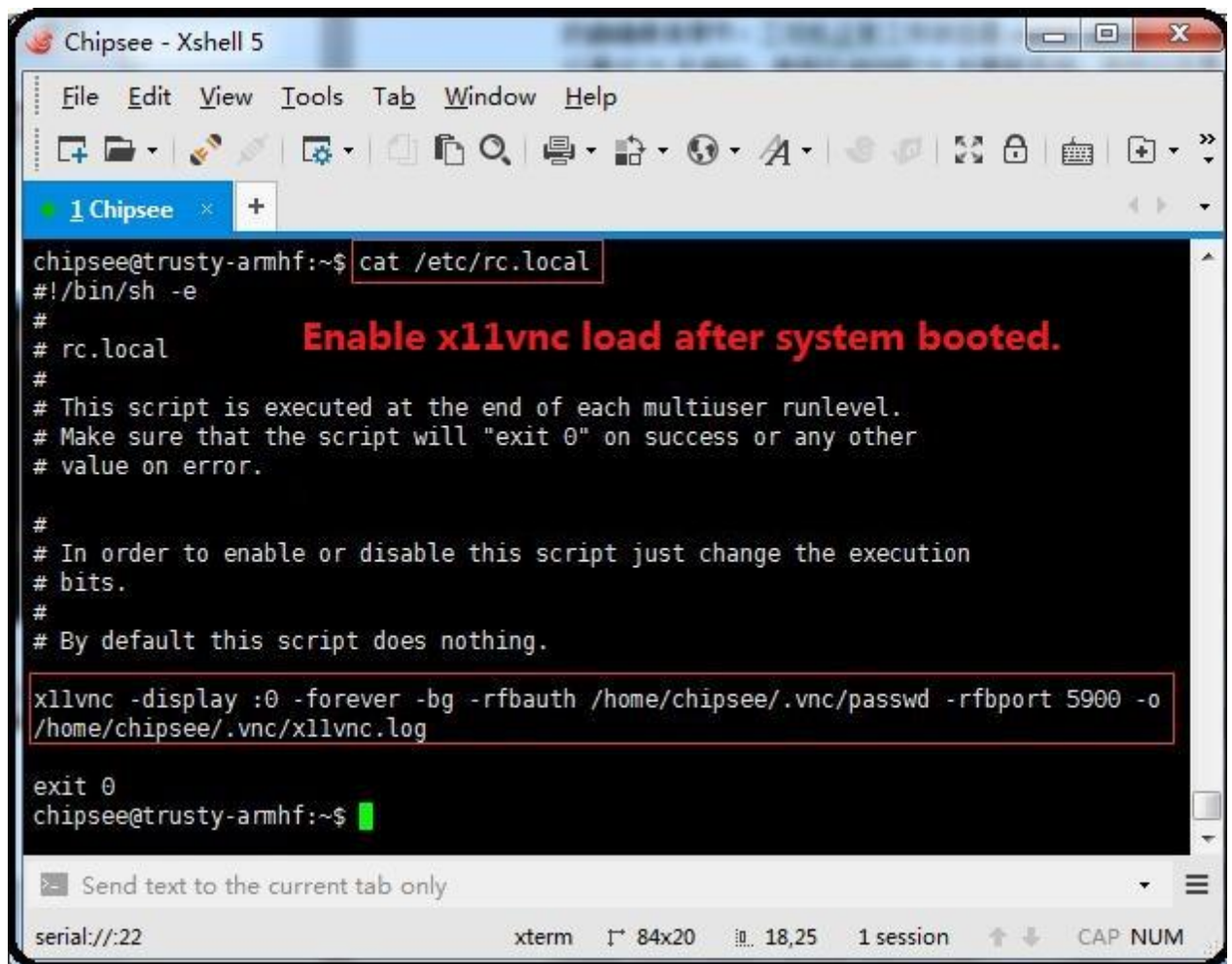
Figure 297: x11vnc auto load
