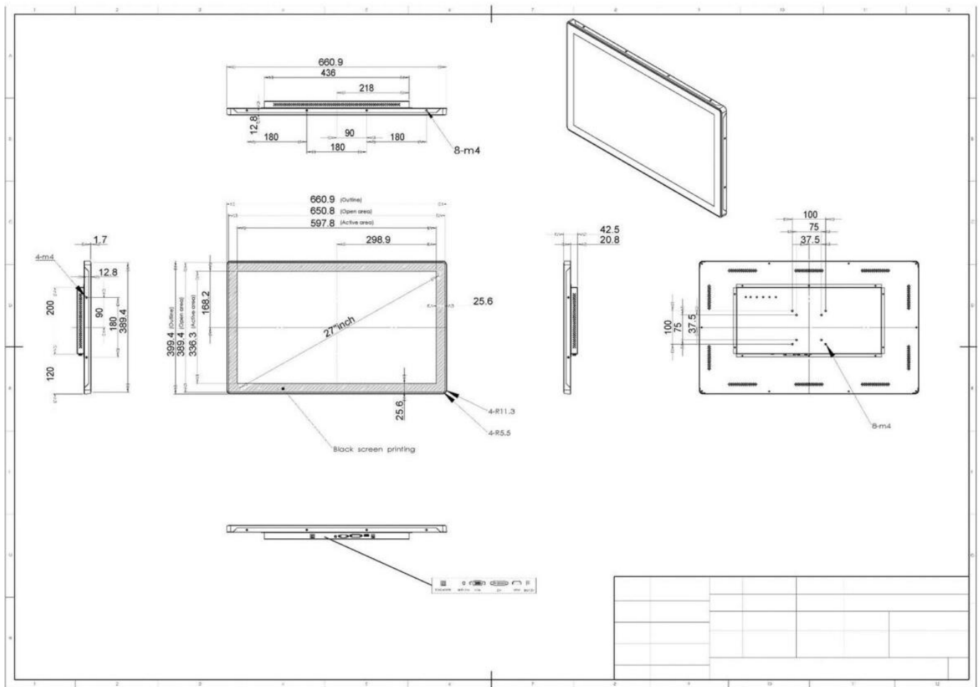
Figure 1030: Technical Drawing
