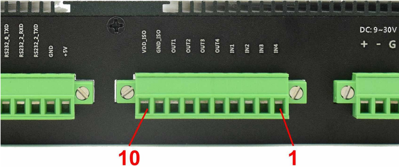
GPIO Terminal
