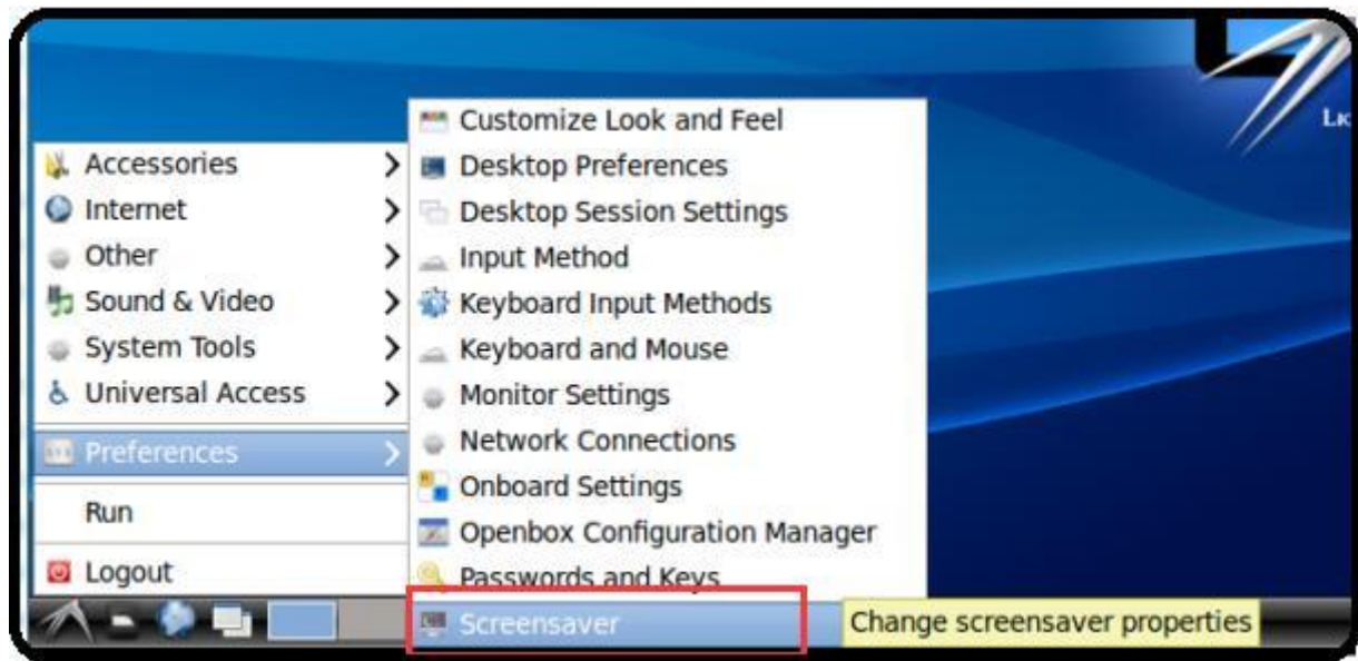
Figure 329: Screensaver
