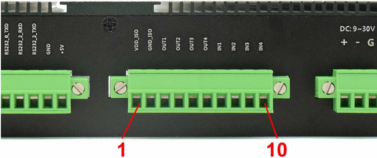
GPIO Terminal
