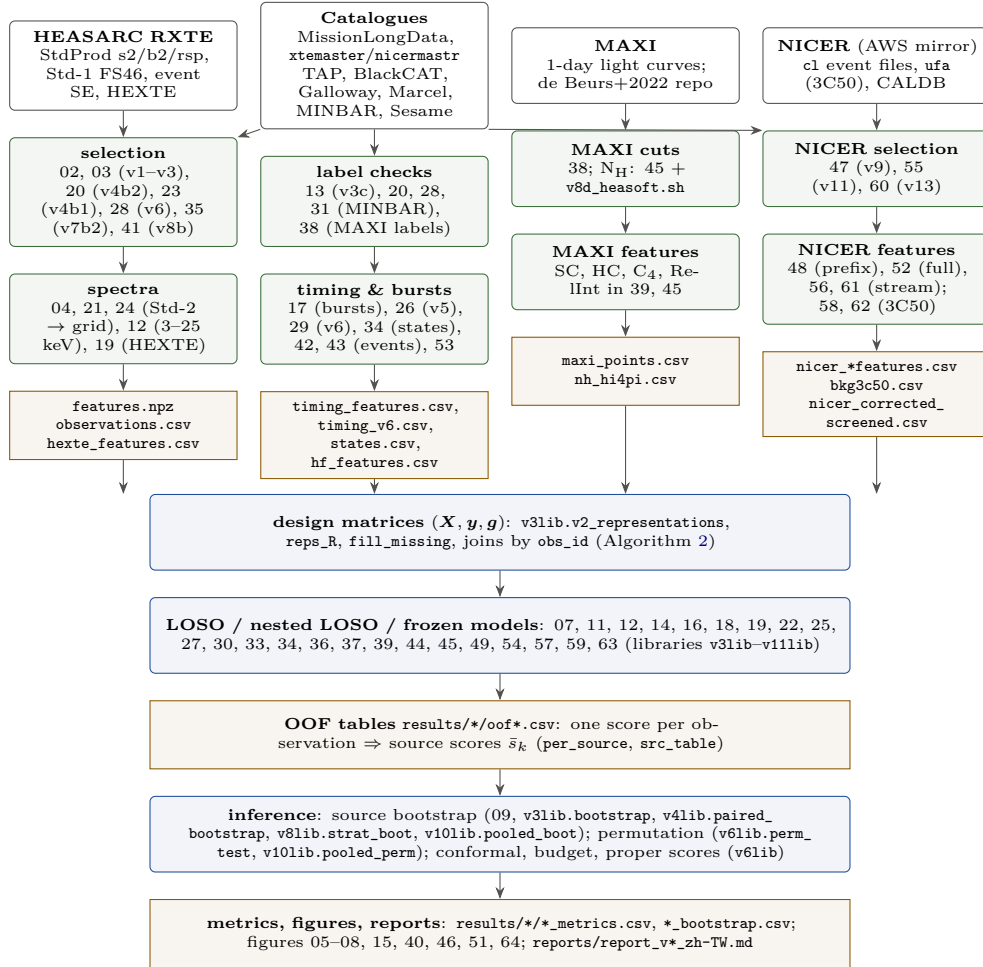
Figure 2.3: End-to-end data flow of the project. Grey boxes: external archives; green: selection and processing scripts (numbers = scripts/NN_*.py ); amber: committed intermediate files; blue: model fitting and inference. Raw files (left of the green boxes) are not in git; everything from the amber row down is committed, so every number in this report can be traced to a file in results/ or data/ . Drawn for this report.
