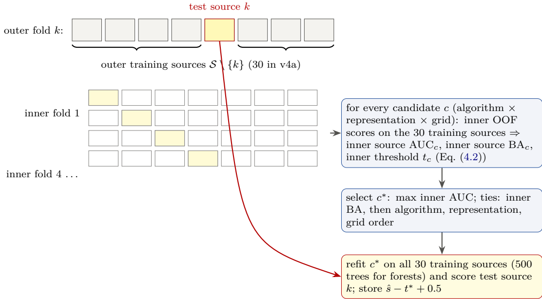
Figure 4.1: Nested LOSO as used in v4a (1d per algorithm and representation; 1e over all 140 configurations). For each outer fold, every candidate configuration is evaluated by an inner LOSO over the outer training sources only; the winner and its inner-optimal threshold are refitted on the outer training sources and applied once to the held-out source. The bias of “choosing the best of many” is therefore included in the outer estimate. Drawn for this report.
