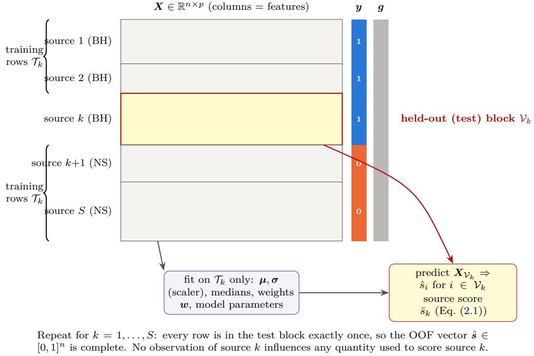
Figure 2.2: Schematic of the design matrix and one leave-one-source-out fold. Rows are observations grouped by source; the y column (blue = BH, orange = NS) and the source index g are attached to \mathbf{X} . The yellow block is the held-out source; every learned quantity – standardisation, imputation medians, sample weights, hyper-parameters, thresholds – is estimated from the grey training rows only. Drawn for this report.
