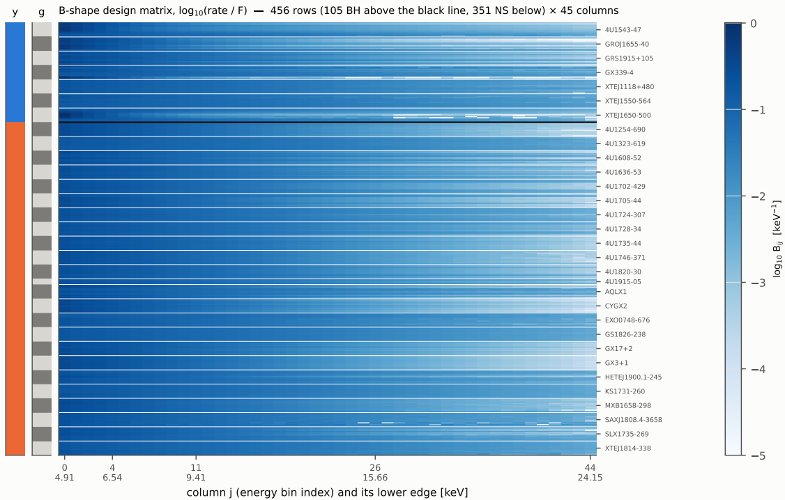
Figure 2.1: The real v2 design matrix for representation B: 456 rows (observations) \times 45 columns (energy bins), colour = \log_{10} B_{ij} (sequential scale, darker = larger). Rows are grouped by source (right labels; alternating grey in strip g ), BH sources first (strip y : blue = 1) and NS below the black line (orange = 0). The steep fall of the shape with energy dominates every row; differences between sources are subtle and mostly in the high-energy columns, consistent with the finding that two colours capture the usable information. Generated for this report from data/v2/processed/features.npz .
