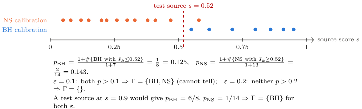
Figure 4.3: Illustration (made-up calibration scores) of the class-conditional conformal p -values of Eq. (4.9). A test source is compared with the calibration sources of each class separately; a label enters the prediction set if the test source is not too atypical for that class. Drawn for this report.
