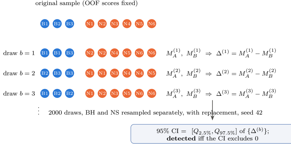
Figure 4.2: Class-stratified source bootstrap with paired differences. Each draw resamples the BH sources and the NS sources separately, with replacement and with all observations of a drawn source; both models are evaluated on the same drawn multiset, so the difference \Delta^{(b)} is paired. No model is refitted. Drawn for this report.
