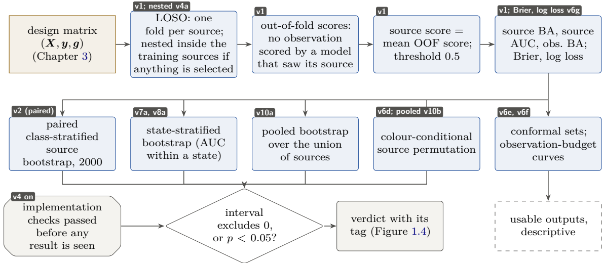
Figure 5.1: Evaluation chain, from the design matrix to a verdict, labelled with the version that introduced each element. Every inferential procedure in the middle row works on fixed out-of-fold scores or fixed features: nothing is refitted inside a resampling or a permutation. Bootstrap and permutation results are judged by the pre-registered rule when the comparison was declared primary or secondary (Figure 1.4); conformal sets and budget curves are always descriptive. Drawn for this report from Table 5.1 and the pre-registrations.
