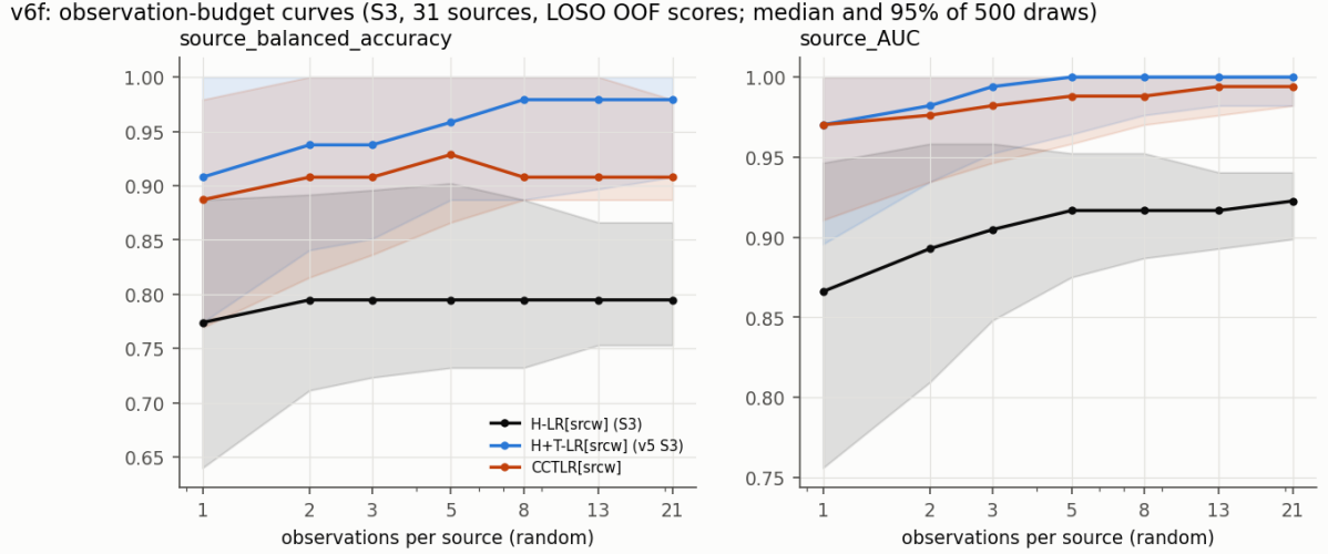
Figure 8.5: Observation-budget curves on S3: source balanced accuracy (left) and source AUC (right) when each source is represented by k randomly drawn observations (LOSO OOF scores of the source-equal-weight models; median and central 95% of 500 draws). Black H-LR, blue H+T-LR, red CCTLR. Repo: figures/v6/v6f_budget_curves.png , scripts/30_v6_analysis.py .
