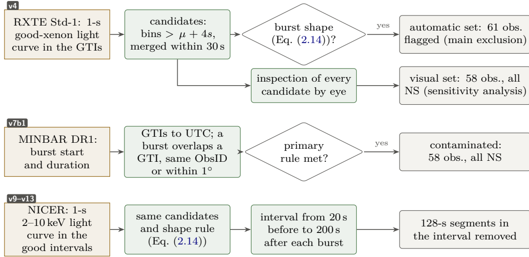
Figure 2.6: The three burst-screening procedures and the version that added each: the Standard-1 detector of v4 (automatic set used for the main exclusion, visual set as sensitivity analysis), the MINBAR catalogue match of v7b1 (primary rule shown; the literal pre-registered rule, any burst of any origin, is a sensitivity set), and the NICER rule of v9–v13, which removes segments rather than observations. Counts refer to the 456 v2 observations (Sections 7.3.1 and 9.6.1). Drawn for this report.
