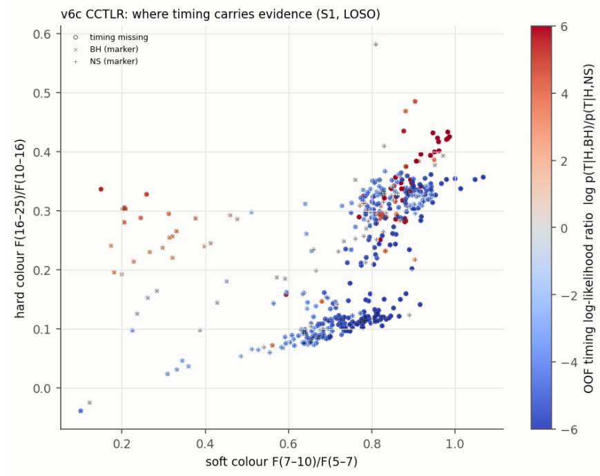
Figure 8.4: Where the timing features carry evidence: each S1 observation in the colour plane, coloured by its out-of-fold CCTLR timing log-likelihood ratio \Lambda = \log p(\mathbf{T} \mid \mathbf{h}, \text{BH}) / p(\mathbf{T} \mid \mathbf{h}, \text{NS}) (red BH-like, blue NS-like, clipped at \pm 6 ); \times = BH, + = NS markers, grey open circles = timing missing ( \Lambda = 0 ). The hard-state corner (hard colour \gtrsim 0.35 ) and the soft BH region at low soft colour are red; the NS banana branch at hard colour \approx 0.1 is blue. Repo: figures/v6/v6c_timing_evidence_map.png , scripts/30_v6_analysis.py .
