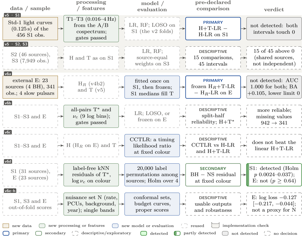
Figure 8.1: Phase 3 analysis map (reading as in Figure 6.1). v5 adds the timing block T to the Phase 1–2 samples; v6 adds the external set E with models frozen after training on S1, better timing estimators, a structured classifier, the colour-conditional permutation test and usable outputs. Both pre-registrations were written after all earlier results. Values from Tables 8.4, 8.7, 8.9, 8.10 and 8.13 and Section 8.6.6. Drawn for this report.
