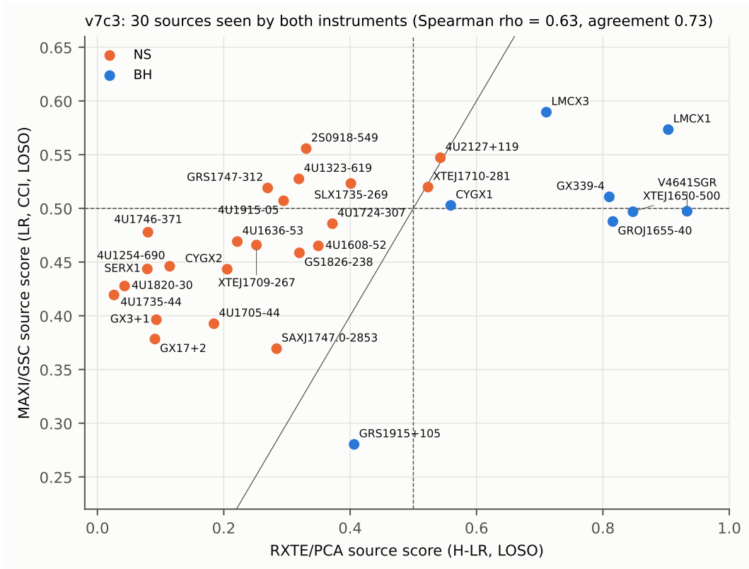
Figure 9.6: RXTE/PCA H-LR source score (horizontal) against MAXI/GSC LR (CCI) source score (vertical) for the 30 common sources (BH blue, NS orange; dashed lines at 0.5; solid line y = x ). The vertical axis is limited to 0.22–0.66, the range of the MAXI scores. Redrawn for this report from results/v7c/v7c3_rxte_vs_maxi.csv (same points as the repository figure figures/v7c/v7c3_rxte_vs_maxi.png of scripts/39_v7c2_analysis.py , whose labels overlap; Spearman \rho and agreement recomputed from the CSV and identical to the repository values).
