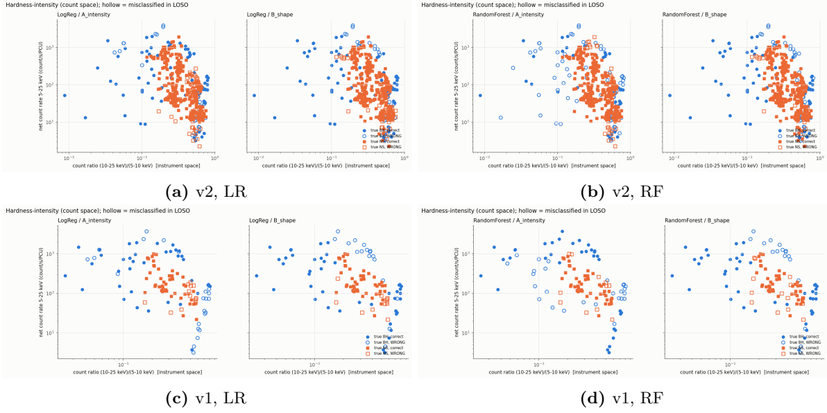
Figure 6.8: Hardness–intensity diagrams in count space: count ratio (10–25)/(5–10) keV (x, log) versus net 5–25 keV rate (y, log), each panel pair for A (left) and B (right); filled = correct, hollow = misclassified under LOSO; circles BH, squares NS. Misclassified NSs cluster at hard ratios ( \gtrsim 0.4 ) and low rates where hard BHs also lie; misclassified BHs are hard observations or the very bright soft GRS 1915+105 observations (top left). Repo: figures/step5_hid_errors_*.png , figures/v2/step5_hid_errors_*.png ; script scripts/08_error_analysis.py .
