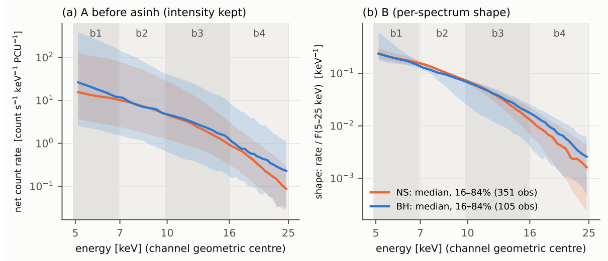
Figure 2.5: Median (line) and 16–84% range (shading) of the v2 count-space spectra, BH (blue, 105 observations) and NS (orange, 351 observations). (a) net rate per keV per PCU (the quantity transformed by asinh in representation A); (b) per-spectrum shape B. Grey and light bands mark the four colour bands b_1 – b_4 of Table 2.5. Non-positive bins are omitted from the percentiles. The class medians differ mainly in the overall slope above 10 keV and overlap strongly, which is why two colours capture most of the shape information (Chapter 6). Generated for this report from data/v2/processed/features.npz ( report_en/figures/generated/make_figures.py ).
