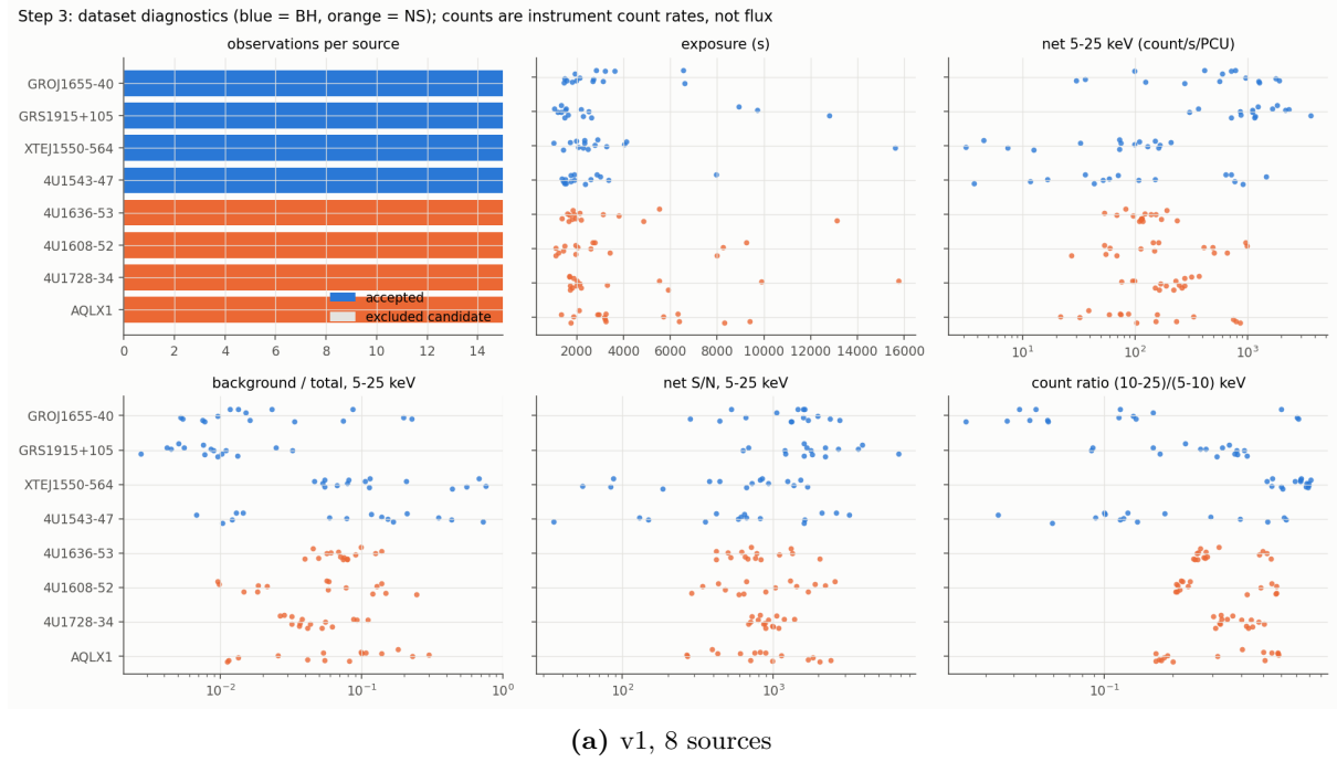
Figure 6.2: Per-source diagnostics of the accepted observations (blue = BH, orange = NS): observations per source (accepted vs excluded candidates), spectrum exposure, net 5–25 keV count rate per PCU, background fraction, net S/N and the count ratio (10–25)/(5–10) keV (log axes where indicated). BH and NS overlap in every quantity; the BHs are on average brighter in v1 (GRS 1915+105, GRO J1655–40), a possible intensity shortcut that representation A could exploit. Repo: figures/step3_dataset_diagnostics.png , figures/v2/step3_dataset_diagnostics.png ; script scripts/06_dataset_checks.py . Panel (b), v2, is in the continuation of this figure.
