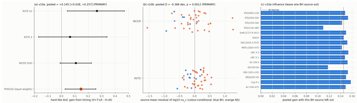
Figure 10.4: v10 pooled tests: (a) hard-like timing gain per component and pooled (red); (b) source-mean residuals of \log_{10} \nu_c at fixed colour per instrument (BH blue, NS orange); (c) pooled gain with each BH source left out (dashed: all sources). Repo: figures/v10/v10_pooled.png , scripts/54_v10_pooled.py .
