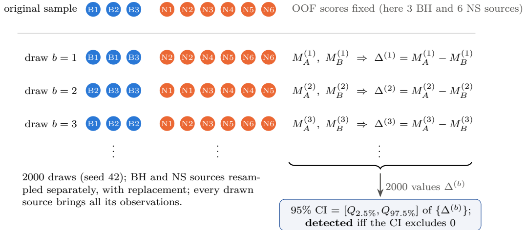
Figure 5.3: Class-stratified source bootstrap with paired differences. Each draw resamples the BH sources and the NS sources separately, with replacement and with all observations of a drawn source; both models are evaluated on the same drawn multiset, so the difference \Delta^{(b)} is paired. No model is refitted. Drawn for this report.
