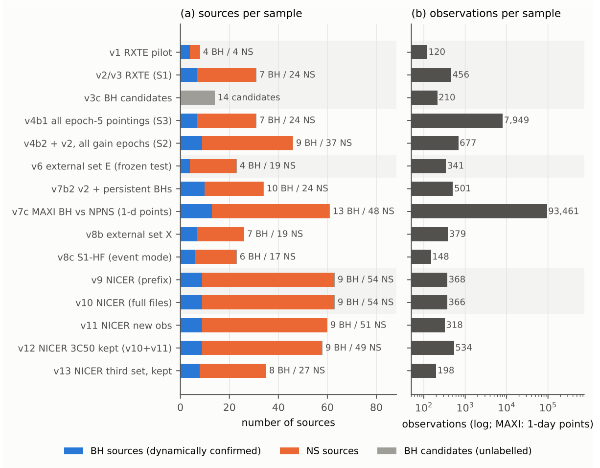
Figure 1.3: Sources (a) and observations (b) of every sample that enters a model. Bars in (a) are stacked: dynamically confirmed BH (blue), NS (orange), unlabelled BH candidates (grey, v3c only). Observations in (b) are on a log scale; for MAXI they are 1-day points. Shaded bands group the six phases. The number of BH sources never exceeds 13 in any single sample (16 over all instruments). Generated for this report from the features.npz files, data/v6/sources.csv , data/v7c/maxi_points.csv , data/v8b/processed/external_states_timing.csv , data/v8c/processed/hf_features.csv , the NICER feature tables and results/v13/v13_frozen_predictions.csv (values in G1_sample_sizes.csv ).
