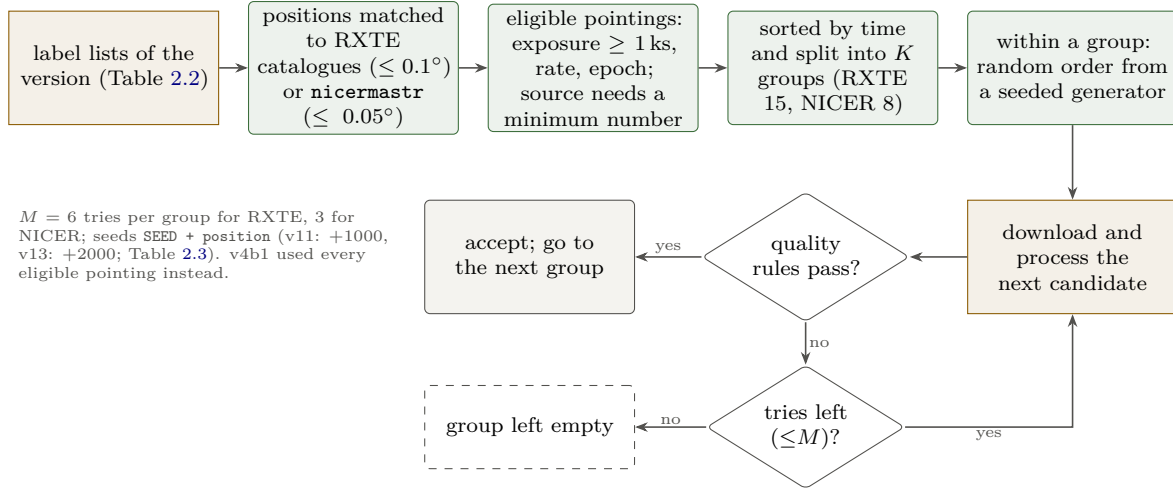
Figure 2.1: Selection of sources and observations (Algorithm 1). The choice of an observation does not depend on its spectral shape or its variability: apart from the quality rules of Section 2.4.5 (exposure, S/N, deadtime, position; NICER: segments and count rate, Section 2.10) it depends only on the label list, the catalogue position, the eligibility rules, the time ordering and a seeded random order. Drawn for this report.
