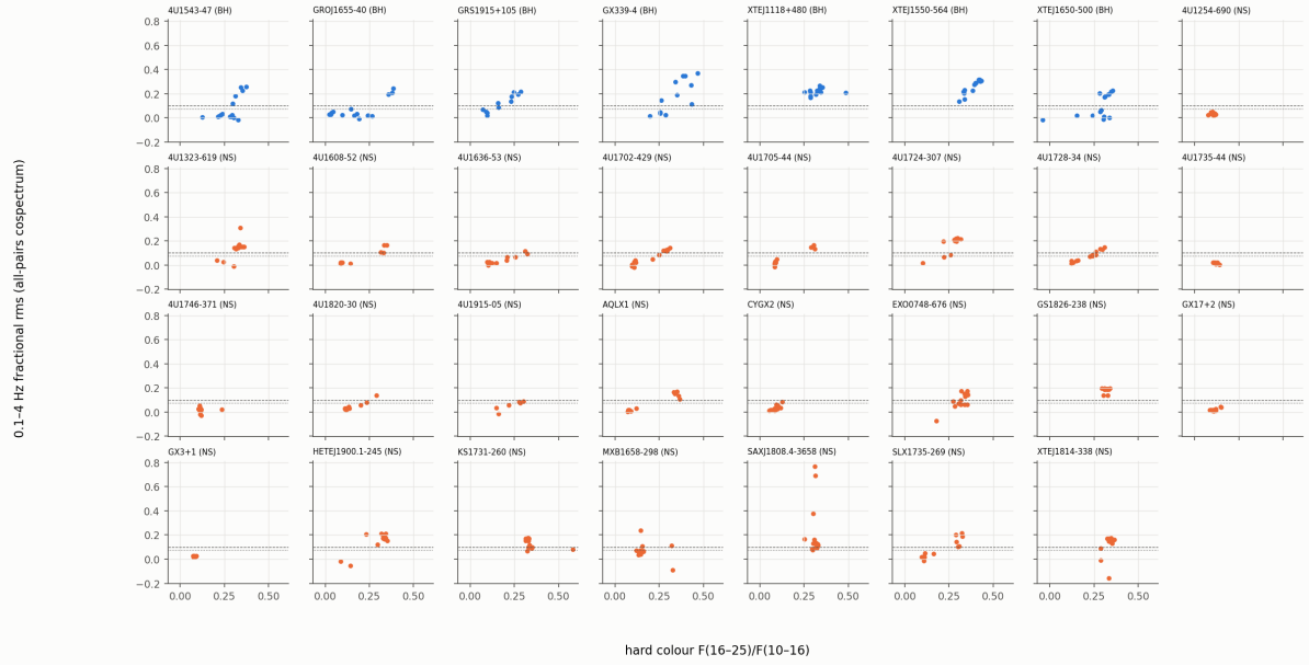
Figure 9.2: The state index (0.1–4 Hz fractional rms, all-pairs cospectrum) against the hard colour for every S1 source (BH blue, NS orange; dashed 0.10 = hard-like threshold, dotted 0.075 = soft-like threshold, RM06 Table 2). XTE J1118+480 and XTE J1550–564 are hard-like throughout; the Z sources Cyg X-2 and GX 17+2 are soft-like; in most sources rms rises with the hard colour. Repo: figures/v7a/v7a_rms_vs_colour_by_source.png , scripts/34_v7a_states.py .
