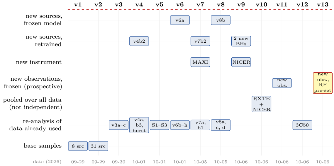
Figure 1.2: What each version adds in terms of independence from data already seen. Rows are ordered from most independent (top) to least; each box is a sub-analysis of the version in its column. External sources (v6a, v8b) were scored by frozen RXTE models, but few BHs were available (4–7). The NICER versions brought a new instrument and two BHs never used before; v10 pooled everything; v11 and v13 used never-read observations of the same sources with frozen pipelines, v13 with the Random Forest chosen before download (highlighted). Every version’s pre-registration was written after all earlier results, so each column knew the results of every column to its left. Not reached by any version: new sources tested prospectively with a frozen model on new data. Drawn for this report from the pre-registrations and reports/decision_log.md .
