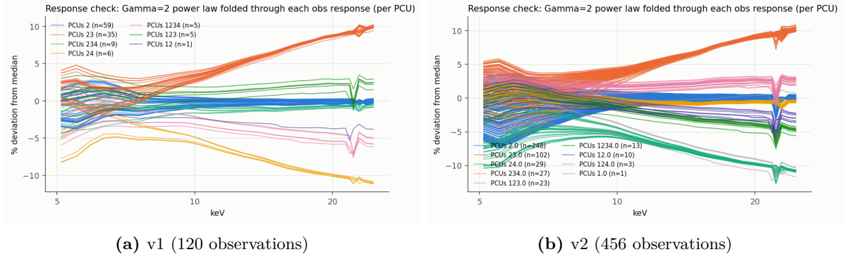
Figure 2.4: Response check: a fixed \Gamma = 2 power law folded through each observation’s response, per PCU, shown as percentage deviation from the median over observations, against energy; colour = PCU combination. The spread (a few per cent, up to \sim 10\% at 25 keV) is set by which PCUs were on, not by the source class. Repo: figures/step3_response_variation.png , figures/v2/step3_response_variation.png ; script scripts/06_dataset_checks.py .
