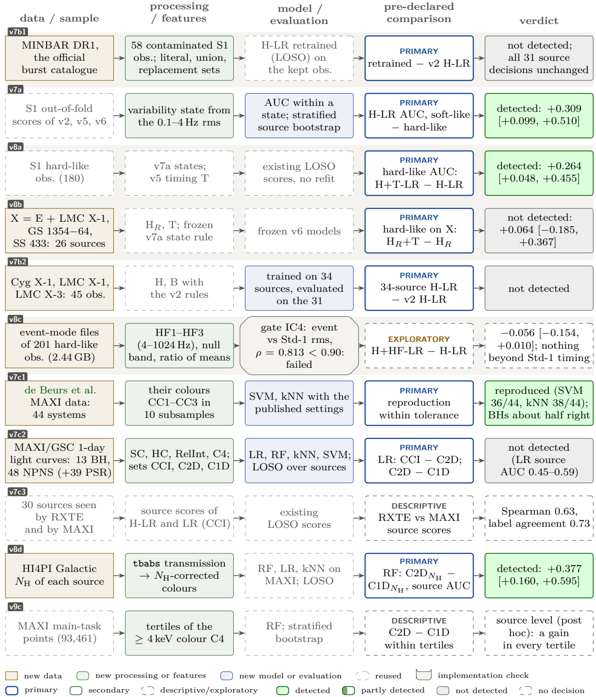
Figure 9.1: Phase 4 analysis map (reading as in Figure 6.1). Shaded and white bands separate the themes: data quality (v7b1), states (v7a), timing within the hard state (v8a, v8b), more BHs (v7b2), higher frequencies (v8c) and an independent instrument (v7c1–v7c3, v8d, v9c). Most RXTE analyses re-use the existing out-of-fold scores and add only a state label or a mask; v8c was downgraded to exploratory when its implementation check failed. Values from Tables 9.7 to 9.9, 9.11, 9.13, 9.14, 9.16, 9.17 and 9.19 to 9.21. Drawn for this report.
