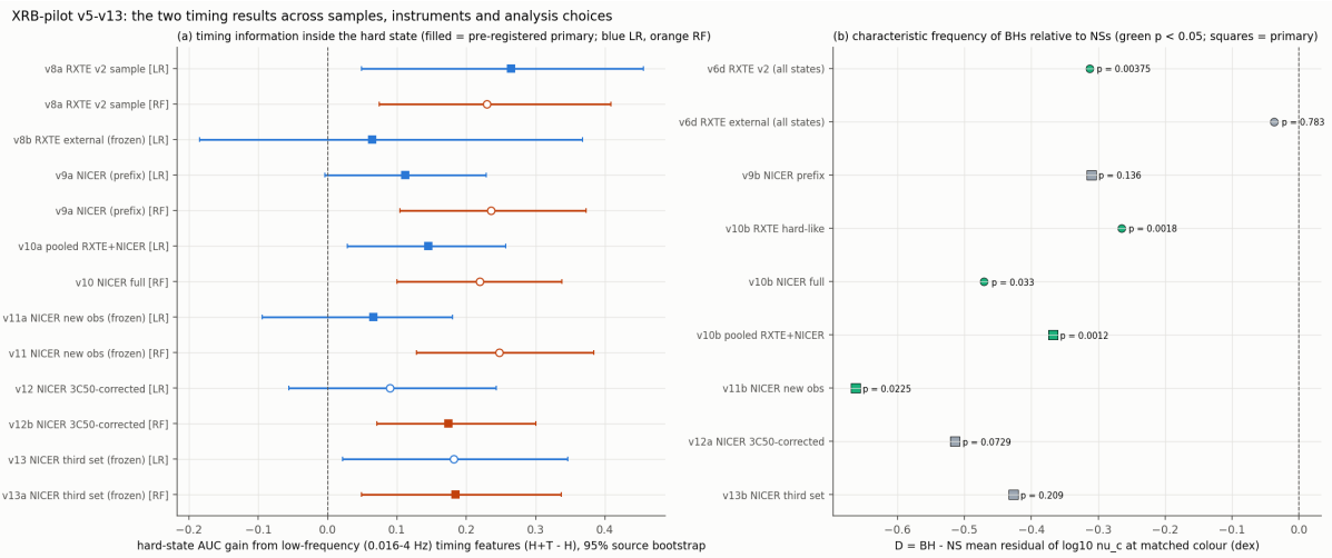
Figure 12.1: The two timing results of v5–v13. (a) Hard-state AUC gain from the 0.016–4 Hz timing features with 95% source-bootstrap intervals (blue LR, orange RF; filled squares = pre-declared primaries). (b) Colour-conditional \log_{10} \nu_c difference BH – NS (green: p < 0.05 ; squares: primaries). Every RF interval lies above 0; the LR intervals of the external and new-observation sets include 0; every D except the four-BH external RXTE set is between −0.27 and −0.66 dex. Repo: figures/final_summary_across_versions.png , scripts/64_final_summary_figure.py ; values in the two results/final_*.csv files.
