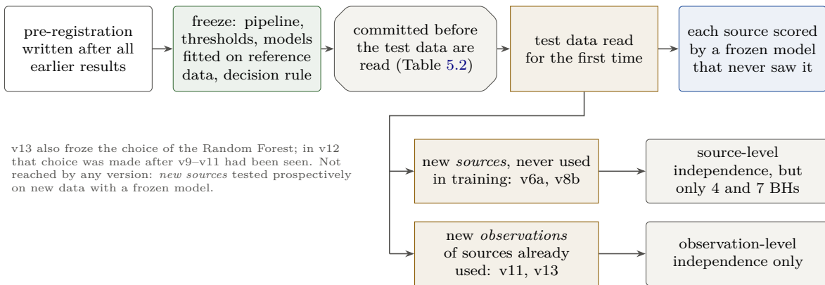
Figure 5.6: Frozen and prospective protocol. Everything that could adapt to the test data was fixed and committed before the data were read. The two kinds of test data give different levels of independence: new sources (v6a, v8b) and new observations of sources already used (v11, v13). Drawn for this report from Table 5.2 and the pre-registrations.
