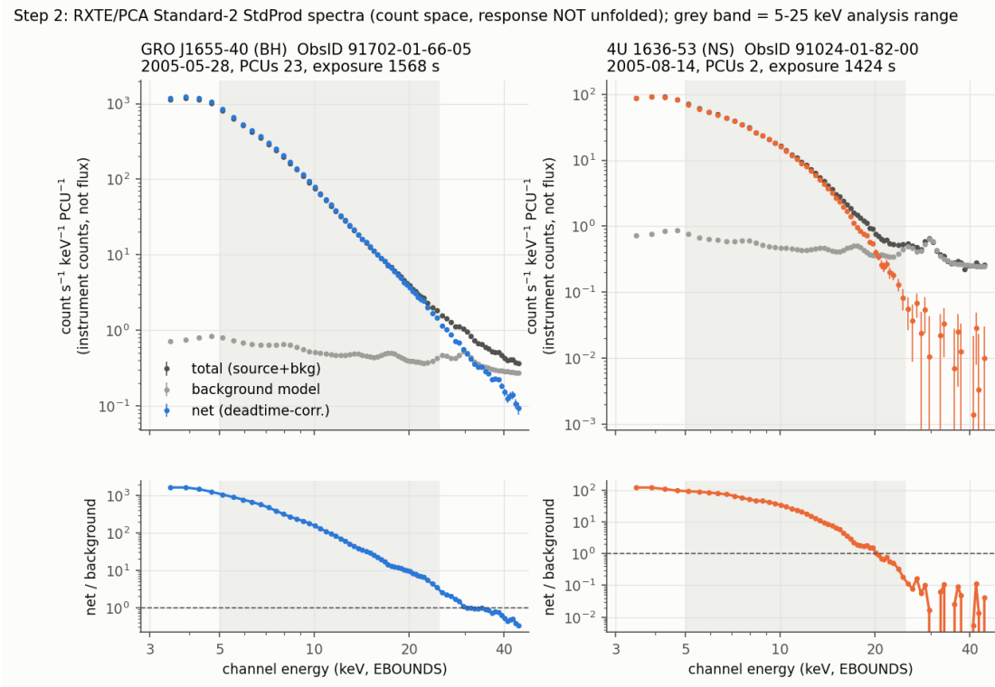
Figure 2.3: Data-flow validation on one BH (GRO J1655–40, ObsID 91702-01-66-05) and one NS (4U 1636–53, ObsID 91024-01-82-00). Top: total (dark grey), background model (light grey) and deadtime-corrected net (colour) count rates per keV per PCU against channel energy (EBOUNDS), log-log; the grey band is the 5–25 keV analysis range. Bottom: net/background ratio. The point is that the net spectrum is background-dominated only above \sim 30 keV for these bright sources, and that everything is in instrument count space (no response unfolding). Repo: figures/step2_two_sources.png , script scripts/05_two_source_check.py .
