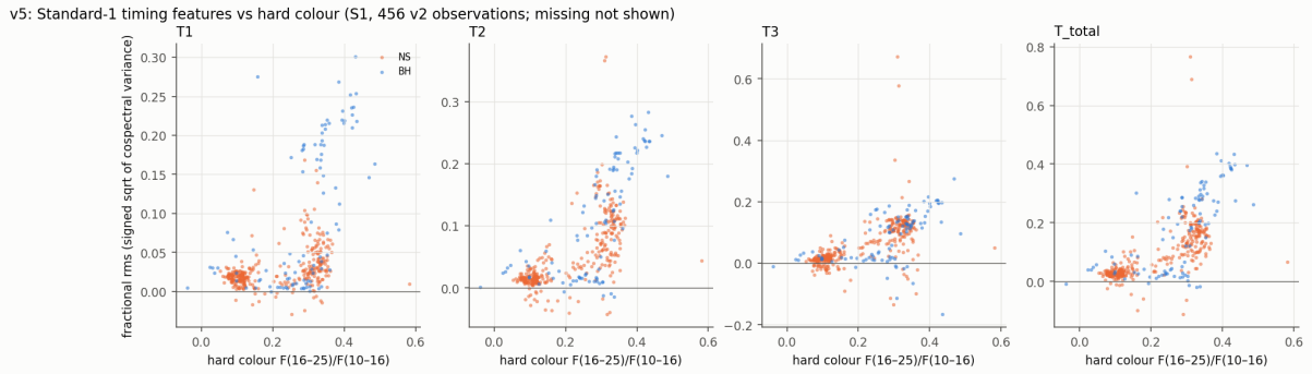
Figure 8.2: v5 timing features against the hard colour F(16-25)/F(10-16) for the 422 S1 observations with timing (BH blue, NS orange; fractional rms = signed square root of the cospectral variance). Panels: T1 (0.016–0.094 Hz), T2 (0.10–1.0 Hz), T3 (1.0–4.0 Hz), T_{\text{total}} . At hard colour \gtrsim 0.3 the BH T1 values (0.1–0.3) lie well above most NS values ( \lesssim 0.1 ); in T3 the classes overlap. Repo: figures/v5/v5_timing_vs_colour.png , scripts/27_v5_analysis.py .
