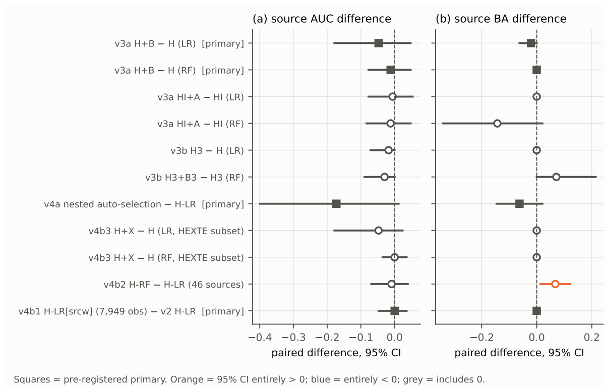
Figure 7.8: Main paired differences of Phases 1–2 against their two-colour baselines with 95% source-bootstrap intervals: (a) source AUC, (b) source balanced accuracy. Rows marked [primary] were the pre-declared primary comparisons of v3a, v4a and v4b1 (the v4b1 main comparison was pre-declared as its main comparison; the pre-registration calls only v4a 1e “primary”). Generated for this report from results/v3/v3a_bootstrap.csv , results/v3/v3b_bootstrap.csv , results/v4/v4a_bootstrap.csv , results/v4b3/v4b3_bootstrap.csv , results/v4b2/v4b2_bootstrap.csv and results/v4b1/v4b1_bootstrap.csv by report_en/figures/generated/make_figures.py ; plotted values in G5_phase12_forest.csv .
