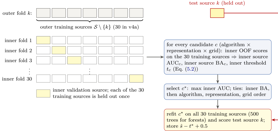
Figure 5.2: Nested LOSO as used in v4a (1d per algorithm and representation; 1e over all 140 configurations). For each outer fold, every candidate configuration is evaluated by an inner LOSO over the outer training sources only; the winner and its inner-optimal threshold are refitted on the outer training sources and applied once to the held-out source. The bias of “choosing the best of many” is therefore included in the outer estimate. Drawn for this report.
