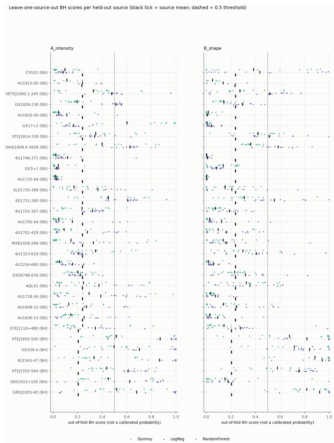
Figure 6.7: v2: out-of-fold BH score of every observation of each held-out source (left: A, right: B; grey Dummy, purple LR, green RF), black tick = source mean, dashed = 0.5. The BH sources (bottom seven) are spread over the whole score range; XTE J1118+480 and GRS 1915+105 are below 0.5 for B. Repo: figures/v2/step4_loso_scores.png ; script scripts/07_train_eval.py (XRB_VERSION=v2).
