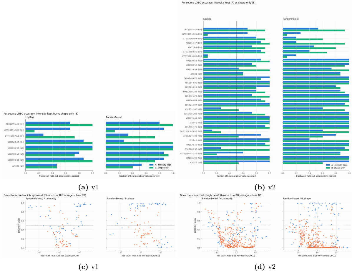
Figure 6.9: Top: fraction of each source’s held-out observations classified correctly with A (blue) and B (green), for LR and RF; dashed = 0.5. Bottom: RF OOF score versus net count rate for A and B (blue BH, orange NS). With A the RF score depends on brightness in a non-monotone way: the faintest ( \lesssim 10 ) and the brightest ( \gtrsim 500 \text{ cs}^{-1} \text{ PCU}^{-1} ) observations of both classes tend to get high BH scores and many BH observations at intermediate rates get low ones – the forest partly learned brightness ranges of the training sources (possible explanation, not verified); with B the BH and NS scores separate at every rate. Repo: figures/step5_per_source_A_vs_B.png , figures/step5_score_vs_rate.png and their figures/v2/ versions; script scripts/08_error_analysis.py .
