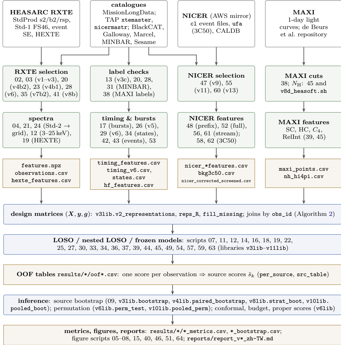
Figure 3.3: End-to-end data flow of the project. Top row (white): external archives and catalogues; green: selection and processing scripts (numbers = scripts/NN_*.py ); amber: committed intermediate files; blue: model fitting and inference. Raw files downloaded from the top-row archives are not in git; everything from the amber row down is committed, so every number in this report can be traced to a file in results/ or data/ . The catalogues feed the RXTE and NICER selections and the label checks (which also define the MAXI labels in script 38). Drawn for this report.
