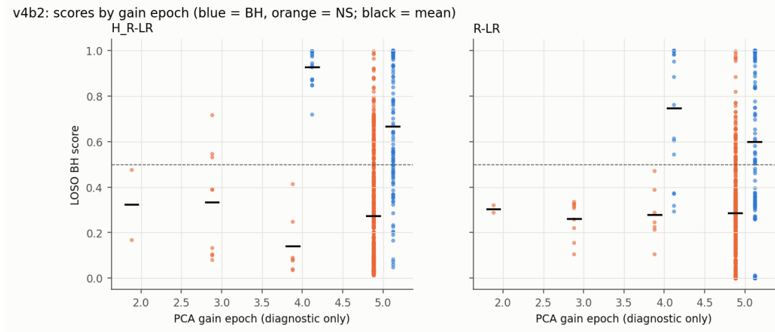
Figure 7.6: LOSO BH scores of the 677 v4b2 observations by PCA gain epoch (diagnostic only; BH blue right of each epoch, NS orange left, black bar = mean). Left: H_R -LR; right: R -LR. The epoch-4 BH points are almost all XTE J1859+226; epochs 2–3 contain only a few NS observations of the new sources. Repo: figures/v4b2/v4b2_scores_by_epoch.png , scripts/22_v4b2_analysis.py .
