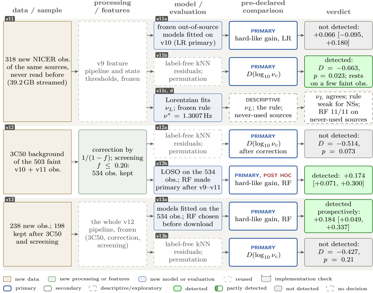
Figure 11.1: Phase 6 analysis map (reading as in Figure 6.1). Every test uses new observations of the same sources (observation-level independence, not new sources). v11 freezes the v9 pipeline and the v10 models; v12 adds the 3C50 background correction and screening; v13 freezes the whole v12 pipeline. RF was made the primary model post hoc in v12 and was pre-specified in v13. Values from Tables 11.3 to 11.5. Drawn for this report.
