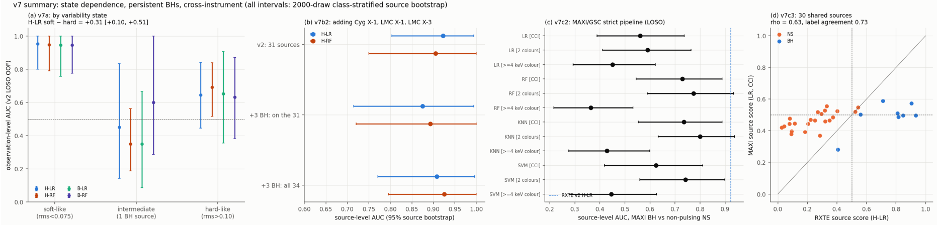
Figure 9.9: v7 summary: (a) AUC by variability state for four models; (b) source AUC of H-LR and H-RF with 31 sources, with 34 sources evaluated on the 31, and on all 34; (c) MAXI source AUC of all models and feature sets (dashed: RXTE v2 H-LR); (d) RXTE vs MAXI source scores of the 30 common sources. Repo: figures/v7/v7_summary.png , scripts/40_v7_summary_figure.py .
