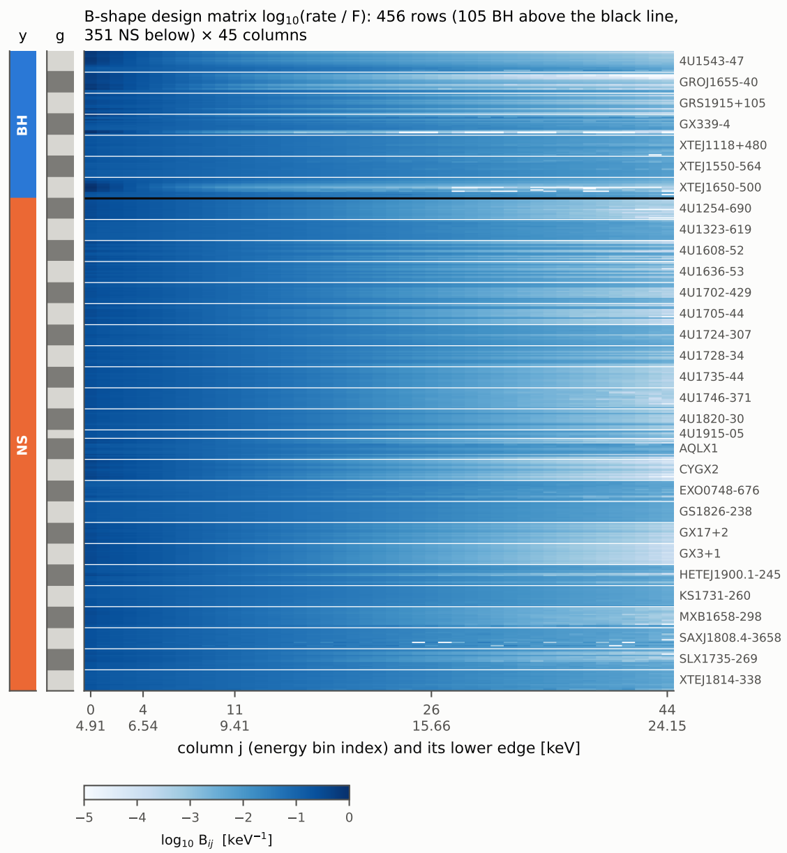
Figure 3.1: The real v2 design matrix for representation B: 456 rows (observations) \times 45 columns (energy bins), colour = \log_{10} B_{ij} (sequential scale, darker = larger). Rows are grouped by source (right labels; alternating grey in strip g ), BH sources first (strip y : blue = 1) and NS below the black line (orange = 0). The steep fall of the shape with energy dominates every row; differences between sources are subtle and mostly in the high-energy columns, consistent with the finding that two colours capture the usable information. Generated for this report from data/v2/processed/features.npz .
