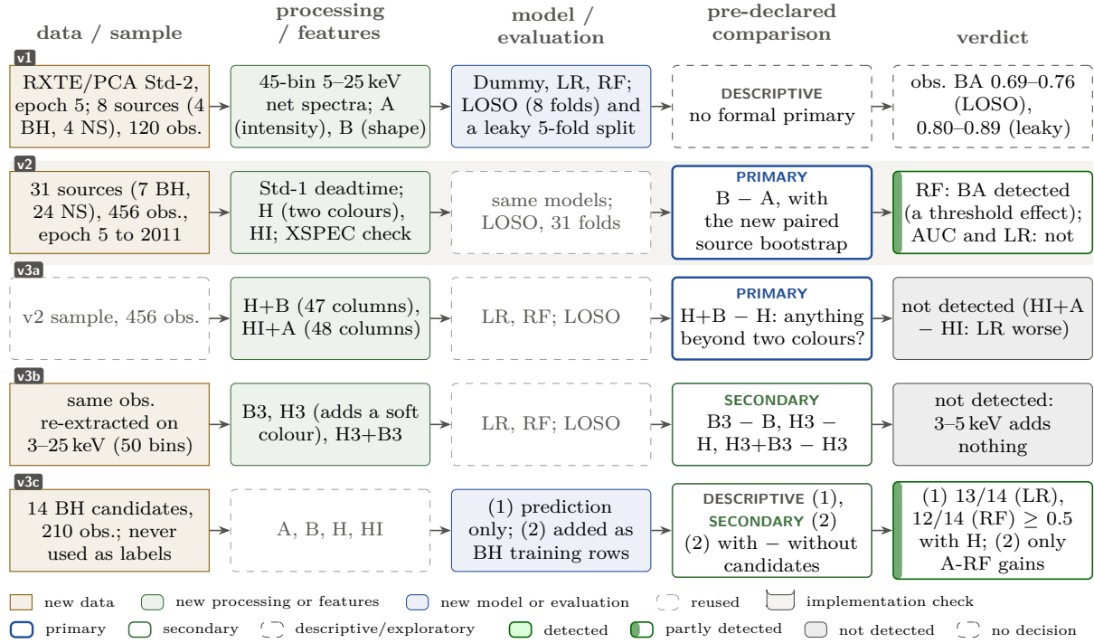
Figure 6.1: Phase 1 analysis map. Each row is one version or sub-analysis, read from left to right: the data, the processing or features, the models and evaluation, the pre-declared comparison and its verdict (95% class-stratified source-bootstrap interval). Solid boxes are new in that version; dashed boxes reuse an element of an earlier version. Values from Tables 6.8, 6.10 and 6.11 and Section 6.6. Drawn for this report.
