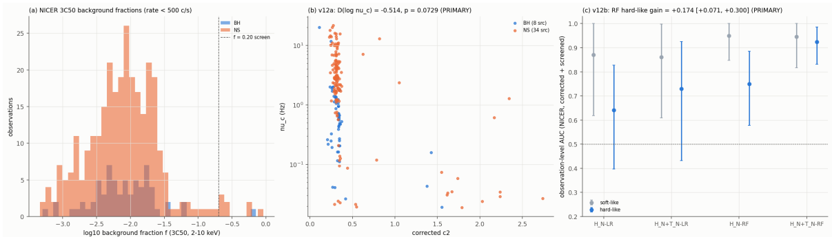
Figure 11.3: v12: (a) 3C50 background fractions of the faint ( < 500 \text{ cs}^{-1} ) observations with the f = 0.20 screen; (b) \nu_c against the corrected c_2 (8 BH, 34 NS sources); (c) AUC by state after correction and screening. Repo: figures/v12/v12_background.png, scripts/59_v12_analysis.py.
