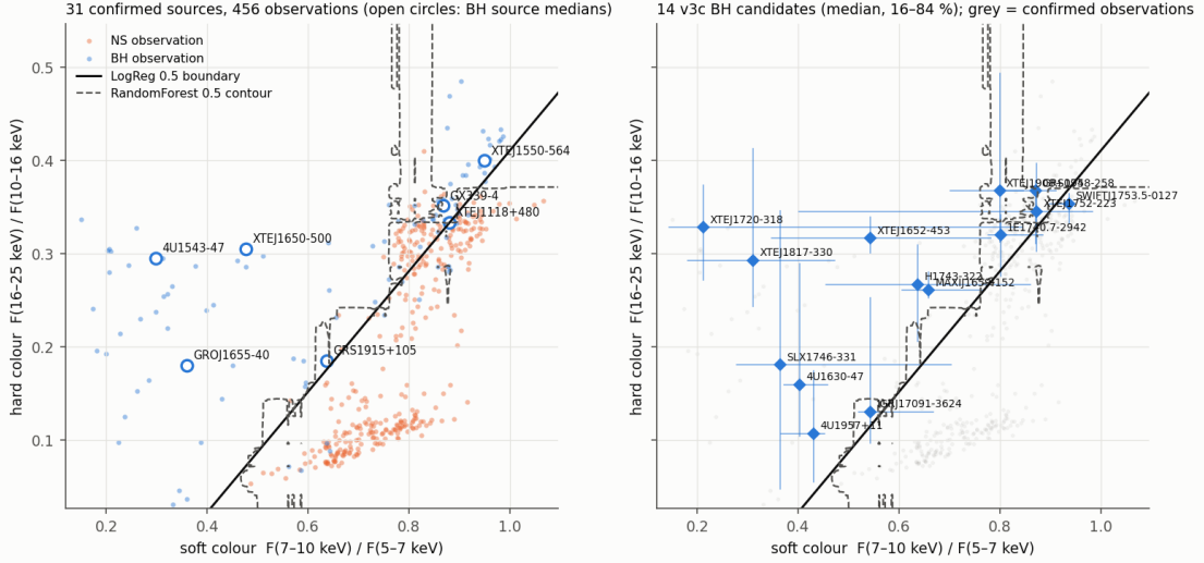
Figure 6.11: The two count-space colours of H: soft F(7-10)/F(5-7) (x) and hard F(16-25)/F(10-16) (y). Left: 456 observations of the 31 confirmed sources (orange NS, blue BH; open circles = BH source medians), the LR 0.5 boundary (solid) and the RF 0.5 contour (dashed), both fitted on all sources for illustration only. Right: the 14 v3c candidates (median and 16–84% range) on the confirmed observations (grey). Look at the upper-right end of the NS track: hard BHs and hard NSs overlap there, which is where every spectral model errs and where Phases 3–6 look for timing information. Repo: figures/final/colour_colour_decision_boundary.png ; script scripts/15_colour_colour.py .
