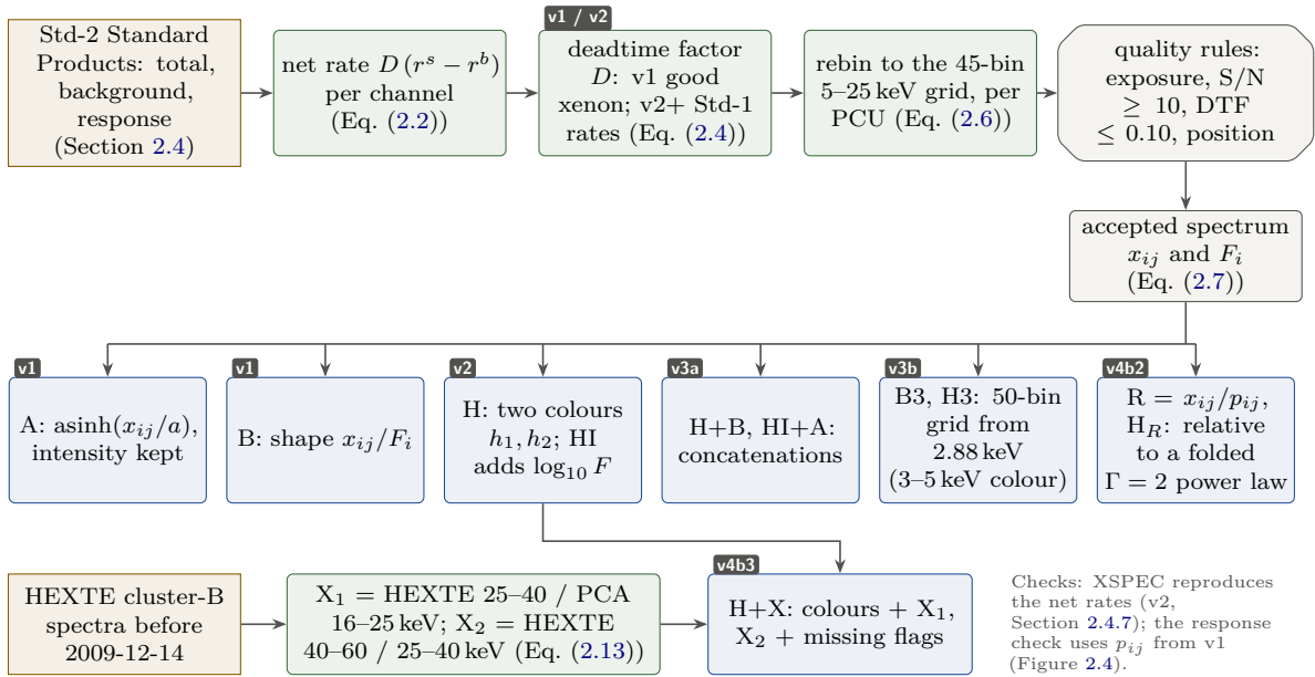
Figure 2.2: RXTE/PCA spectral pipeline. Top row: processing of every observation (the quality rules decide whether the next candidate of the same time group is tried, Algorithm 1). Middle: the representations built from the accepted spectrum, labelled with the version that introduced them; every model of Phases 1–4 uses one of them. Bottom: the HEXTE colours added in v4b3. Drawn for this report from Sections 2.4 to 2.6.
