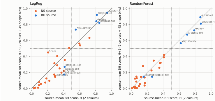
(a) v3a: H vs H+B source scores
