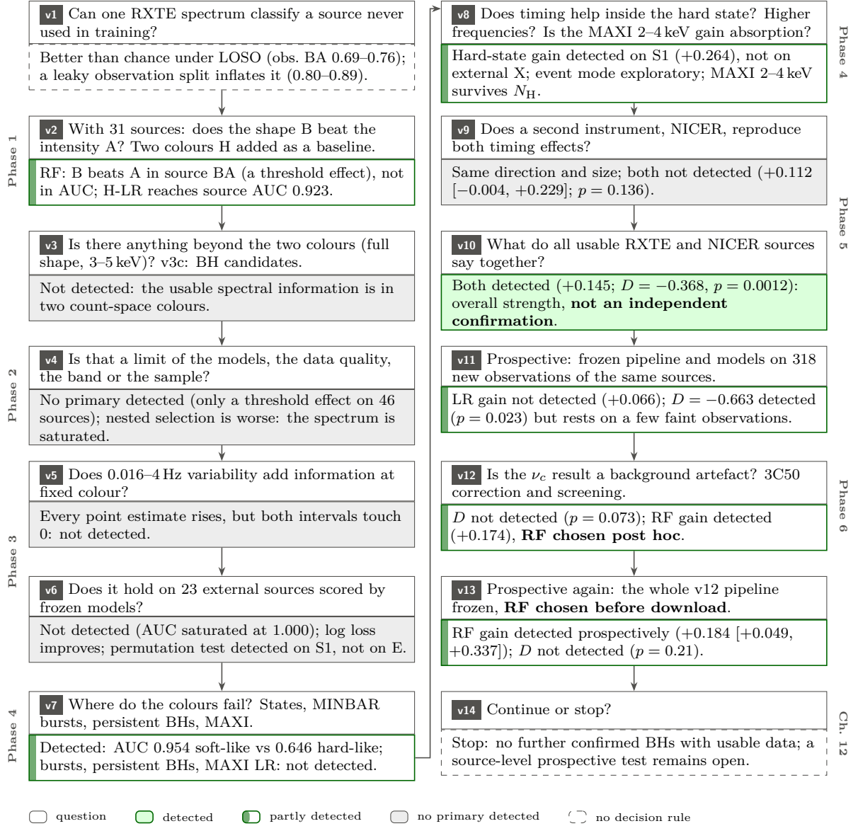
Figure 1.5: The chain of questions. Each version (white: its question) was designed after the results of all earlier versions (coloured: what it found, by the verdict of its pre-declared comparisons). Read down the left column (v1–v7), then the right column (v8–v14). The series moved from spectra (Phases 1–2) to timing (Phases 3–4), then to a second instrument and pooled evidence (Phase 5) and to prospective tests on new observations of the same sources (Phase 6). Detailed maps: Figures 6.1, 7.1, 8.1, 9.1, 10.1 and 11.1. Drawn for this report from the phase chapters.
