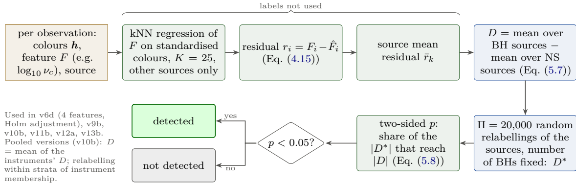
Figure 5.4: Colour-conditional source permutation test. The colour dependence of the feature is removed without labels (neighbours only from other sources), so the class enters only through D and its permutation null; the source, not the observation, is relabelled. Drawn for this report from Eqs. (4.15), (5.7) and (5.8) and v6lib.perm_test , v10lib.pooled_perm .
