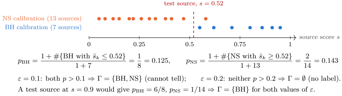
Figure 5.5: Illustration (made-up calibration scores) of the class-conditional conformal p -values of Eq. (5.9). A test source is compared with the calibration sources of each class separately; a label enters the prediction set if the test source is not too atypical for that class. Drawn for this report.
