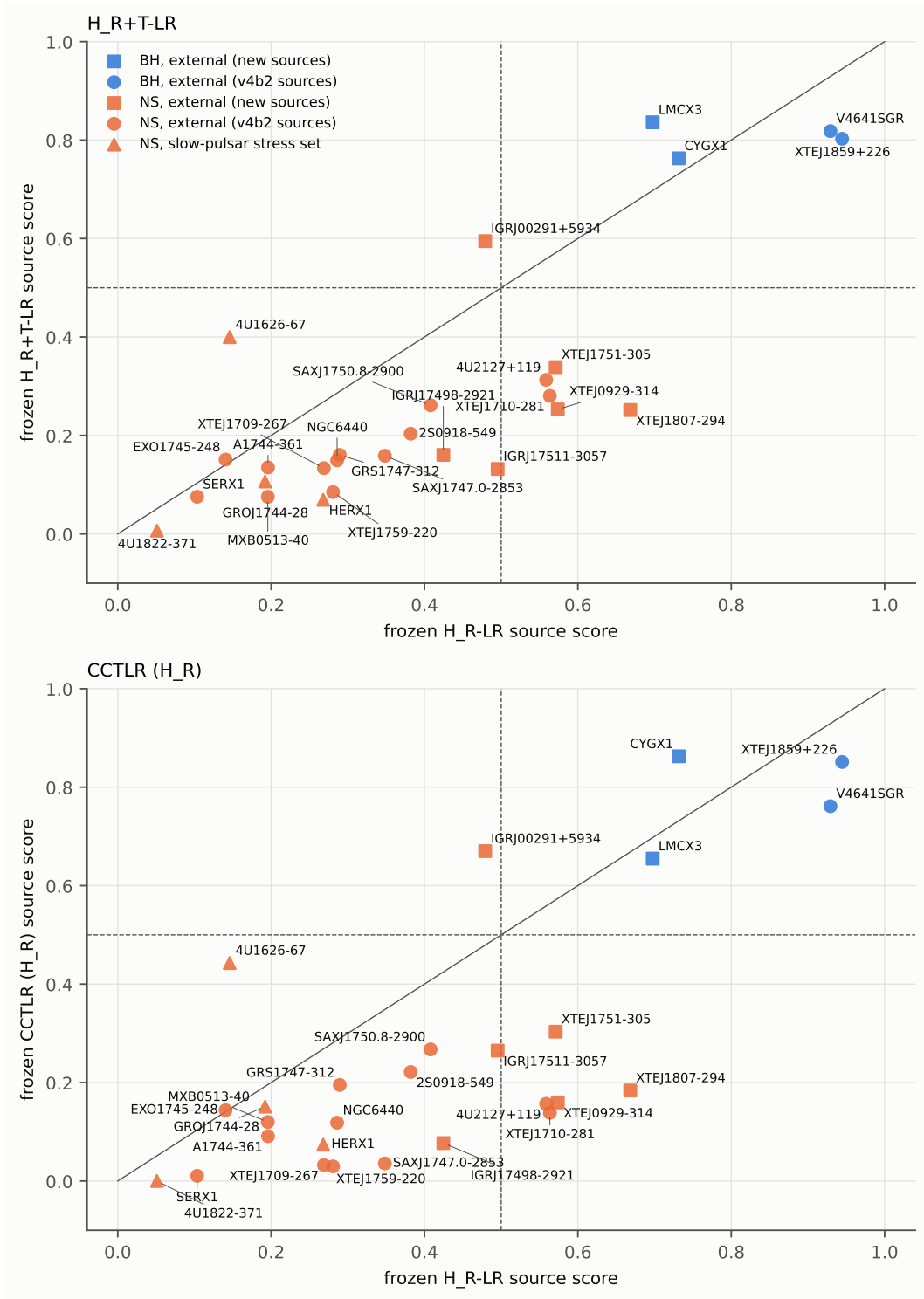
Figure 8.3: Source scores of the frozen models on sources never used in training: horizontal, colour-only H_R -LR; vertical, H_R +T-LR (top) and CCTLR (bottom). Squares = E_{\text{new}} , circles = v4b2 sources, triangles = slow-pulsar stress set; BH blue, NS orange; dashed lines at 0.5. Points in the lower-right quadrant are NSs misclassified by colour and corrected by timing; IGR J00291+5934 moves the other way, and 4U 1626–67 is pushed up by its coherent 0.13 Hz pulsation. Redrawn for this report from results/v6/v6a_external_per_source.csv (same points and encoding as the repository figure figures/v6/v6a_external_sources.png of scripts/30_v6_analysis.py , whose source labels overlap); labels are offset, with leader lines, so that none overlap.
