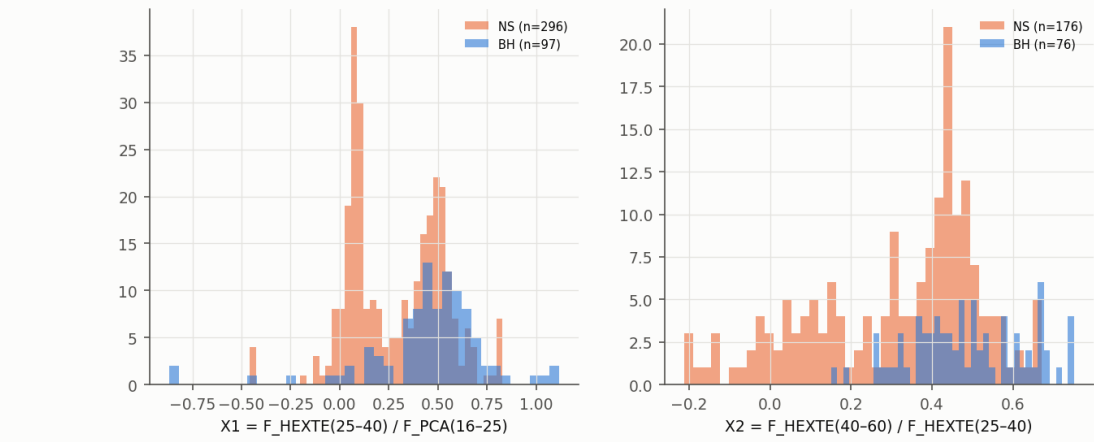
Figure 7.3: HEXTE cluster-B colours (Eq. (7.1)) of the v2 observations with valid values, BH blue, NS orange. Left: X_1 (393 observations: 97 BH, 296 NS); right: X_2 (252 observations: 76 BH, 176 NS). The NS X_1 distribution is bimodal (soft states near 0, hard states near 0.5); the BHs lie mostly in the hard NS mode, and the X_2 distributions overlap. Repo: figures/v4b3/v4b3_hexte_colours.png , scripts/19_v4b3_hexte.py ; values in data/v4b3/processed/hexte_features.csv .
