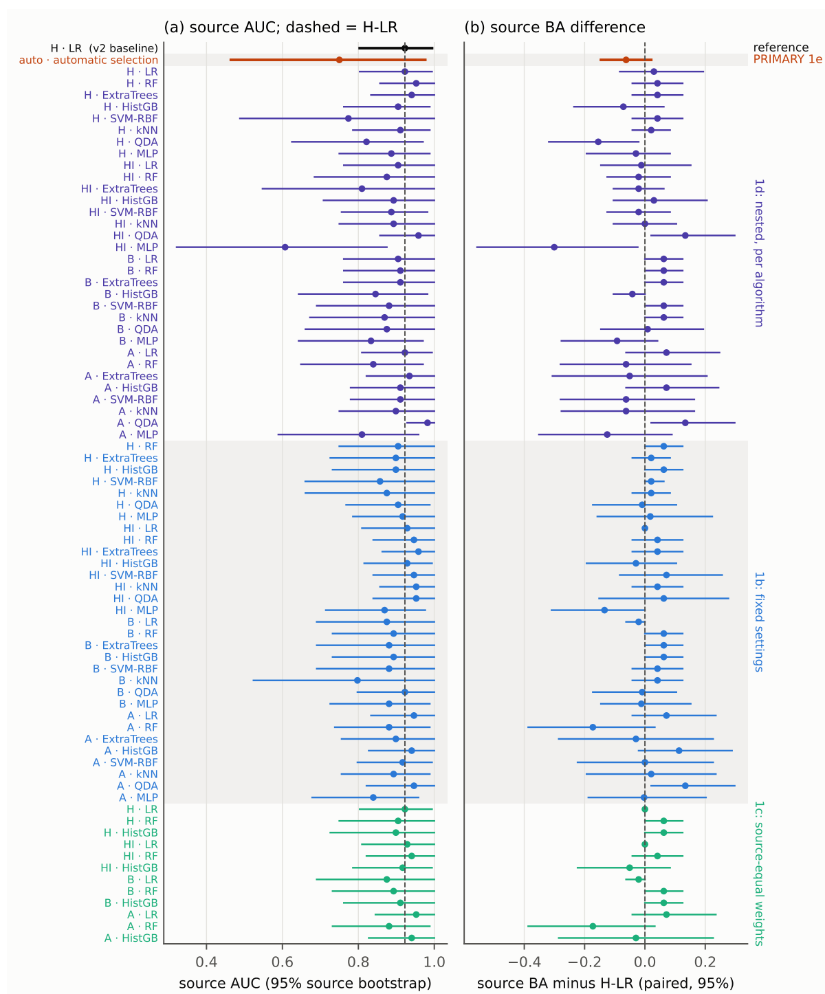
Figure 7.4: All v4a combinations. Left: source-level AUC with 95% source-bootstrap interval (dashed line = H-LR, 0.923); right: paired difference in source balanced accuracy against H-LR. Orange = the primary nested automatic selection (1e), purple = nested per algorithm (1d), blue = fixed settings (1b), green = source-equal weights (1c), black = the H-LR baseline. The primary is the lowest-AUC entry except HI-MLP (nested); the three source-BA intervals above 0 are A-QDA (fixed), HI-QDA and A-QDA (nested). Redrawn for this report from results/v4/v4a_bootstrap.csv with the same rows, order, colours and intervals as the repository figure figures/v4/v4a_forest_source_auc.png of scripts/16_v4a_algorithms.py , whose 77 row labels are unreadable at page size; rows are labelled representation · algorithm and grouped by sub-analysis (right margin).
