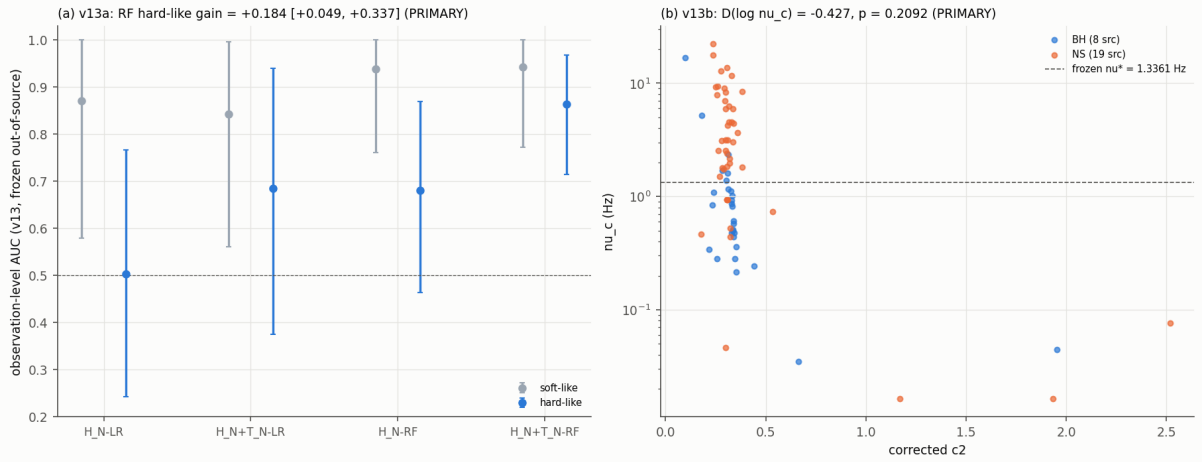
Figure 11.4: v13 on a third set of new observations with the frozen v12 pipeline: (a) AUC by state of the frozen out-of-source models; (b) \nu_c against the corrected c_2 with \nu^* = 1.3361 Hz – at c_2 \approx 0.3 the BHs lie mostly below the NSs. Repo: figures/v13/v13_prospective.png , scripts/63_v13_analysis.py .
