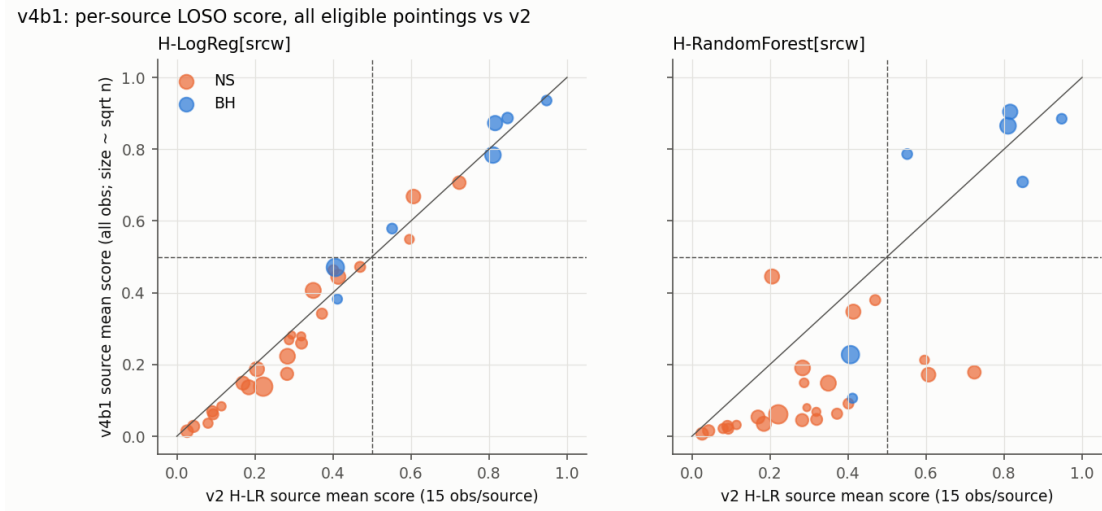
Figure 7.7: Per-source LOSO mean scores with all eligible observations (v4b1, vertical) against the v2 H-LR with 15 observations per source (horizontal); marker size \propto \sqrt{n} , BH blue, NS orange, dashed lines at 0.5. Left: H-LR with source-equal weights – every source stays on the diagonal and in the same quadrant. Right: H-RF with source-equal weights – the forest pushes most NSs to lower scores and moves the NSs that H-LR misclassifies below 0.5, but GRS 1915+105 (large blue circle near 0.23) and XTE J1118+480 stay below 0.5. Repo: figures/v4b1/v4b1_source_scores.png , scripts/25_v4b1_analysis.py .
