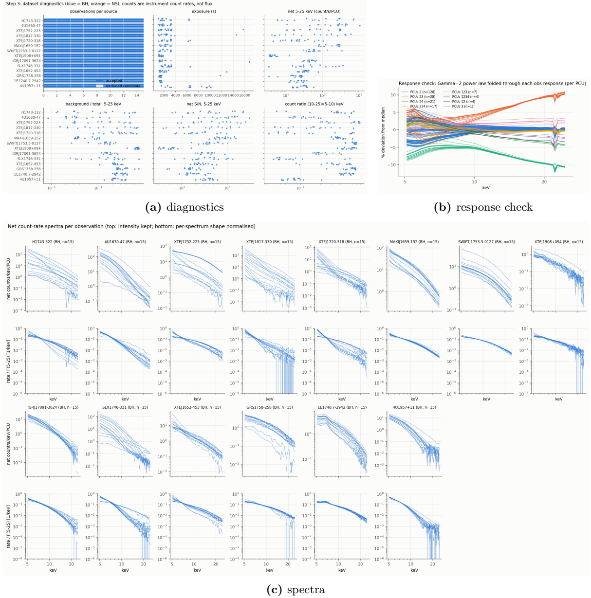
Figure 6.4: The 14 v3c BH candidates (all plotted in the BH colour although they are unlabelled): per-source diagnostics as in Figure 6.2, the response check of Figure 2.4, and spectra as in Figure 6.3. XTE J1908+094 is the faintest (median 4.1 \text{ cs}^{-1} \text{ PCU}^{-1} ); 4U 1630–47 the brightest (269). Repo: figures/v3c/step3_*.png ; script scripts/06_dataset_checks.py with XRB_VERSION=v3c .
