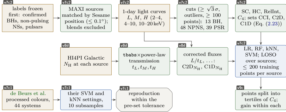
Figure 2.9: MAXI/GSC pipeline. v7c2 froze the labels before any light curve was downloaded and used the cuts of de Beurs et al. (2022) ; v8d added the Galactic absorption correction, which feeds the same models; v9c split the points into tertiles of the \geq 4 keV colour C_4 . The reproduction of de Beurs et al. (2022) (v7c1) uses their processed colours, not this pipeline. Drawn for this report from Sections 2.11 and 9.6.6.
