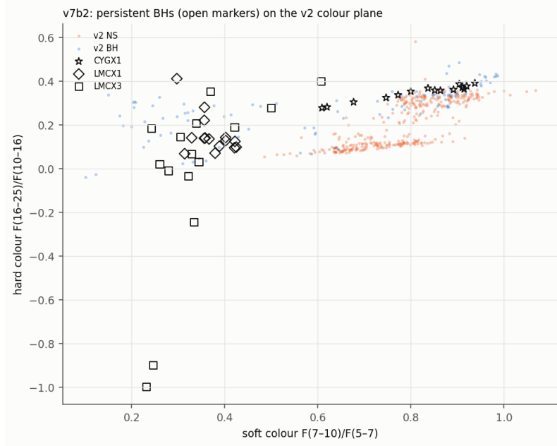
Figure 9.5: The 45 observations of the persistent BHs (open symbols: star Cyg X-1, diamond LMC X-1, square LMC X-3) on the v2 colour plane (dots: v2 BH blue, NS orange). The two LMC X-3 points near hard colour -1 are the high-leverage faint observations. Repo: figures/v7b2/v7b2_colour_positions.png , scripts/36_v7b2_analysis.py .
