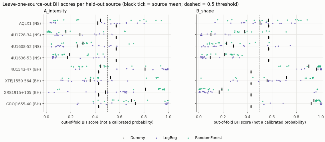
Figure 6.5: v1: out-of-fold BH scores of every observation of each held-out source (left A, right B; grey Dummy, purple LR, green RF), black tick = source mean, dashed line = 0.5. GRS 1915+105 is classified by its intensity (A) but not by its shape (B); XTE J1550–564 the other way round. Repo: figures/step4_lososcores.png ; script scripts/07_train_eval.py .
