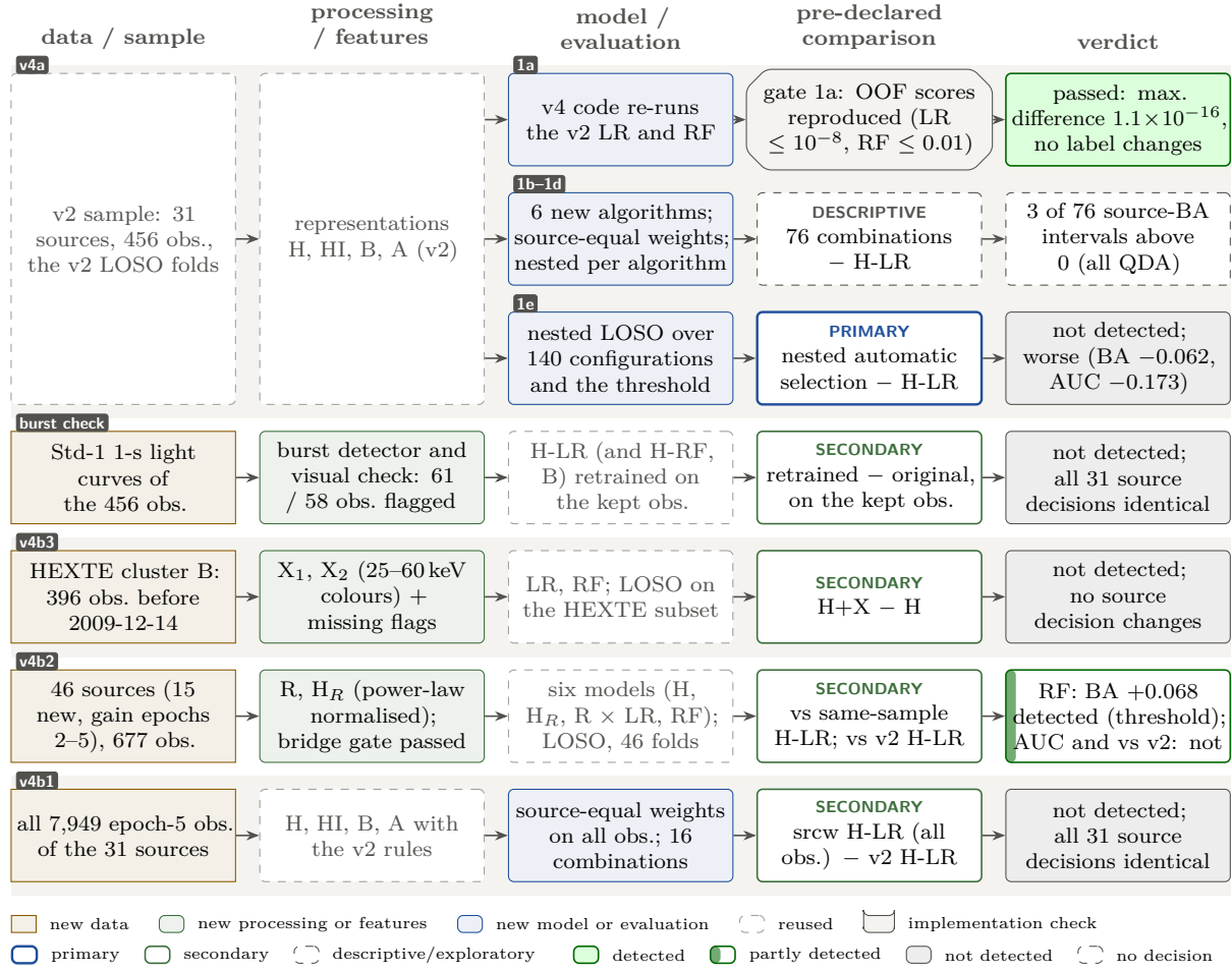
Figure 7.1: Phase 2 analysis map (reading as in Figure 6.1: solid boxes are new in that sub-analysis, dashed boxes reuse earlier elements). The three v4a procedures share the v2 sample and representations; the 1a reproduction gate had to pass before any v4 result was looked at. Every comparison is paired with H-LR on the same bootstrap resamples. Values from Tables 7.6, 7.9, 7.10, 7.12 and 7.14 and Figure 7.4. Drawn for this report.
