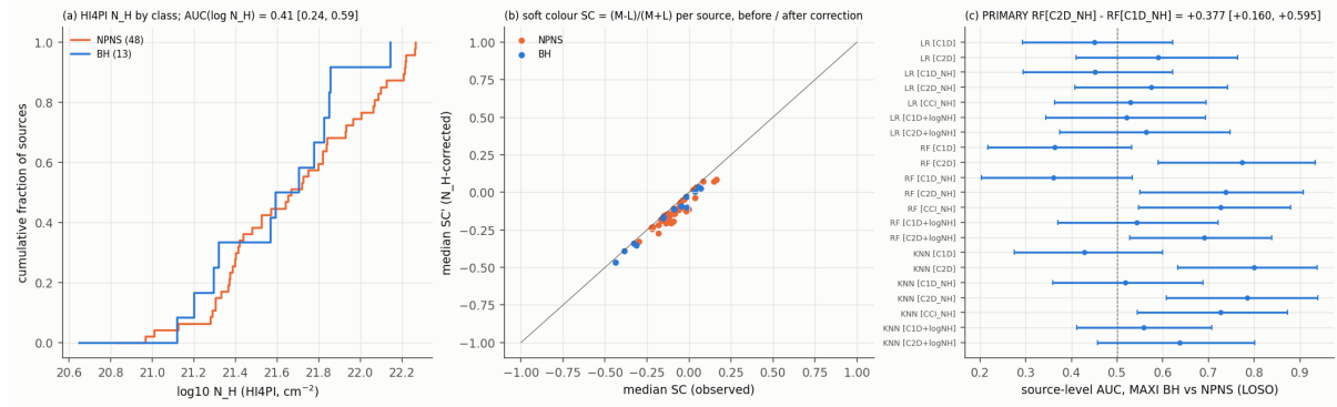
Figure 9.7: v8d: (a) cumulative HI4PI \log N_H of the 13 BHs and 48 NPNS (AUC of \log N_H alone 0.41); (b) per-source median soft colour SC before and after the correction; (c) source AUC of all model/feature combinations (95% source-bootstrap intervals). Repo: figures/v8d/v8d_nh_control.png , scripts/45_v8d_nh.py .
