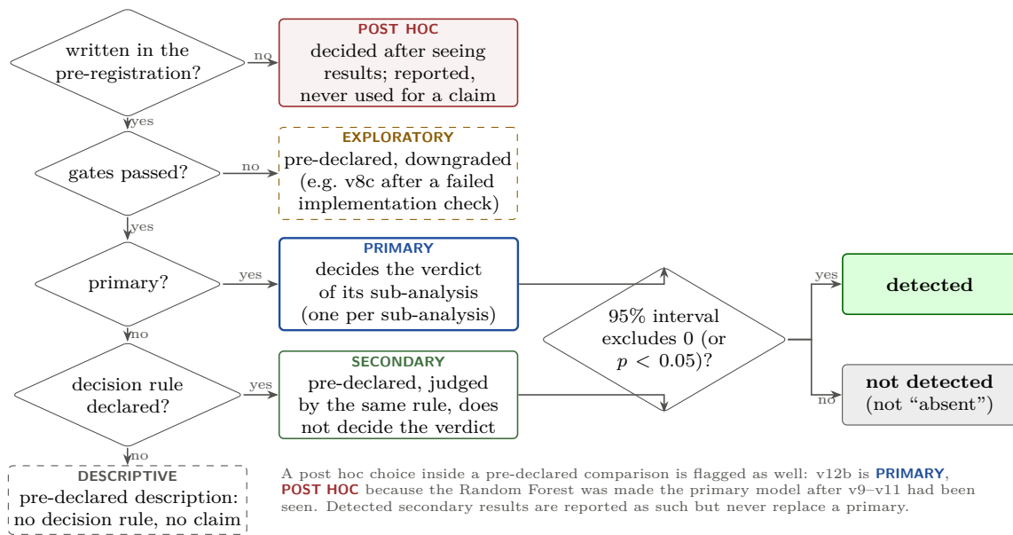
Figure 1.4: How a comparison receives its status tag and its verdict. Only primary and secondary comparisons are judged by the pre-registered rule; descriptive, exploratory and post hoc results are reported but never used to claim a difference. “Not detected” means that the interval includes 0 under the pre-registered criterion, not that the effect is absent. The interval is the paired 95% class-stratified source-bootstrap interval (Section 5.5). Drawn for this report from the pre-registrations and Section 5.11.
