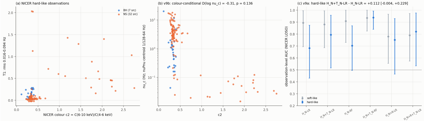
Figure 10.2: NICER hard-like observations (BH blue, 7 sources; NS orange, 32 sources): (a) T1 rms against the colour c_2 = C(6-10)/C(4-6) ; (b) \nu_c against c_2 – at c_2 \approx 0.2-0.4 the BHs lie at lower \nu_c , and the very hard NS observations ( c_2 > 0.7 ) have very low \nu_c ; (c) observation-level AUC by state for the v9a models. Repo: figures/v9/v9_nicer.png , scripts/49_v9_analysis.py .
