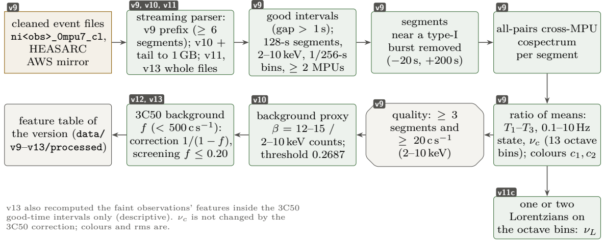
Figure 2.8: NICER/XTI feature pipeline (read the top row left to right, then the bottom row right to left). The v9 steps were frozen before the new observations of v11 were read, and the whole chain including the 3C50 step before those of v13; v10 added the full-length read and the background proxy, v11c the Lorentzian fits, v12 the 3C50 correction and screening. The colours are computed from the same segment windows as the timing features. Drawn for this report from Section 2.10 and scripts/v9lib.py-v11lib.py .
