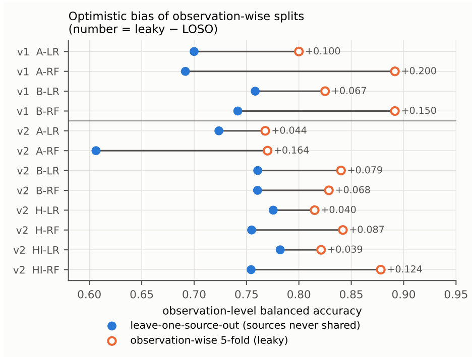
Figure 1.1: Optimism of observation-wise cross-validation. For every representation and model of v1 (8 sources) and v2 (31 sources), observation-level balanced accuracy under leave-one-source-out (filled blue) and under a stratified 5-fold split over observations in which sources appear in both training and test folds (open orange); the number is the difference. The leaky split is optimistic in every case (+0.04 to +0.20), most for models that can memorise intensity (A-RF). Generated for this report from results/metrics_observation_level.csv , results/secondary_observation_split.csv and their results/v2/ counterparts ( report_en/figures/generated/make_figures.py ; values in G4_leakage.csv ).
