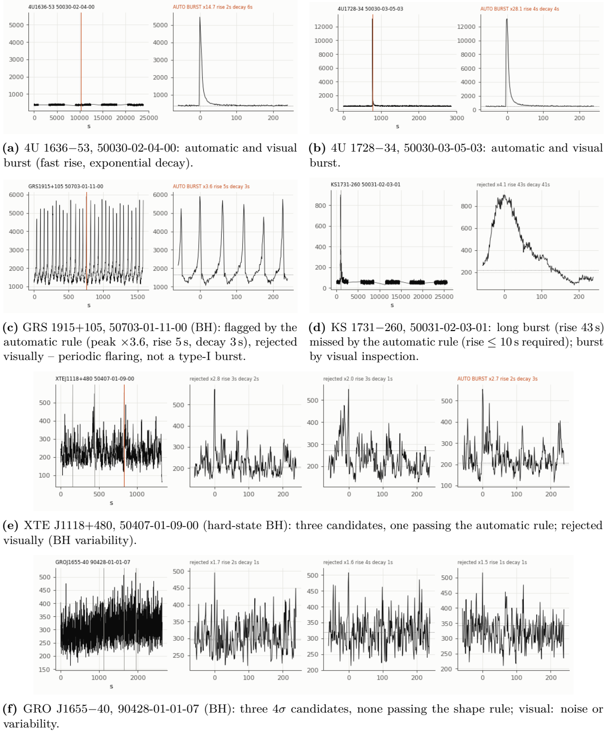
Figure 7.2: Six of the burst-candidate plots, chosen to show each outcome (true positive, BH false positive, missed long burst, rejected candidates). Each plot: left, the whole 1-s Standard-1 light curve of the observation ( \text{counts s}^{-1} summed over the PCUs on; GTI gaps joined by lines; red marks = candidates); then one zoom per candidate with the persistent level (dotted) and the automatic verdict (peak ratio, rise and half-decay times) in its title. Repo: figures/v4/burst_candidates/ (one PNG per observation with candidates), produced by scripts/17_v4_burst_detect.py ; verdicts in results/v4/burst_visual.csv .
