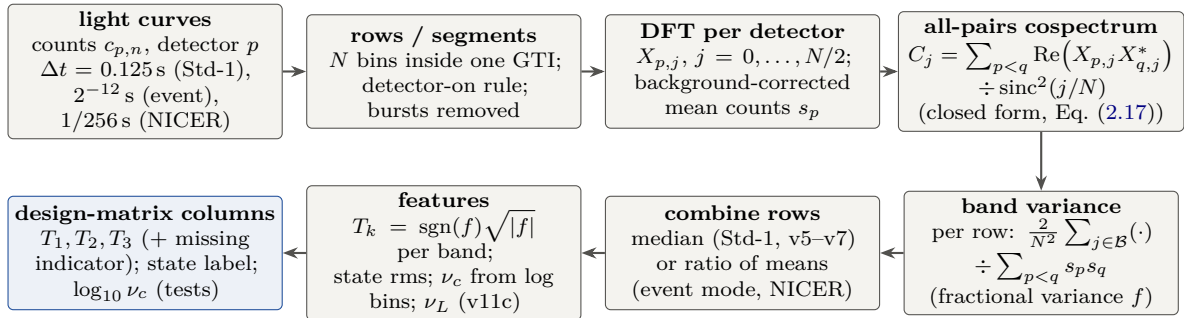
Figure 2.7: Timing-feature pipeline shared by RXTE Standard-1 (v5–v10), RXTE event mode (v8c) and NICER (v9–v13). Differences between the instruments are in the bin width, the segment length, the “detector” (PCU or NICER MPU), whether rows are combined by the median or by the ratio of means, and the frequency bands (Table 2.6). Drawn for this report.
