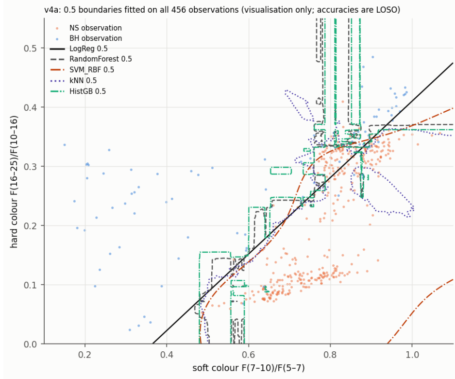
Figure 7.5: 0.5 decision boundaries in the H colour plane (soft colour F(7-10)/F(5-7) , hard colour F(16-25)/F(10-16) , count space) of LR, RF, SVM-RBF, kNN and HistGB fitted on all 456 v2 observations (blue BH, orange NS). Visualisation only; all accuracies in this chapter are LOSO. Repo: figures/v4/v4a_colour_boundaries.png , scripts/16_v4a_algorithms.py .
