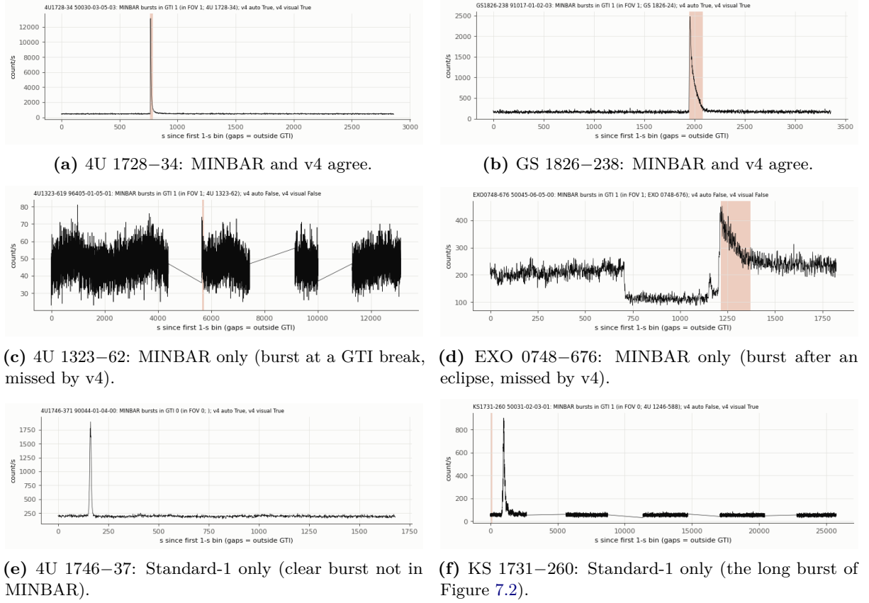
Figure 9.3: MINBAR versus the v4 Standard-1 burst detector: 1-s Standard-1 light curves ( \text{counts s}^{-1} , time since the first bin; gaps are outside the GTIs) with MINBAR burst intervals shaded; the title states the MINBAR match and the v4 automatic and visual verdicts. Repo: figures/v7b1/ (one PNG per agreeing or disagreeing observation), scripts/31_v7b1_minbar.py .
