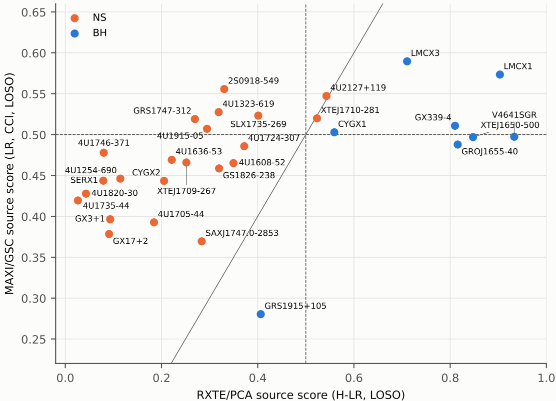
v7c3: 30 sources seen by both instruments (Spearman rho = 0.63, agreement 0.73)
