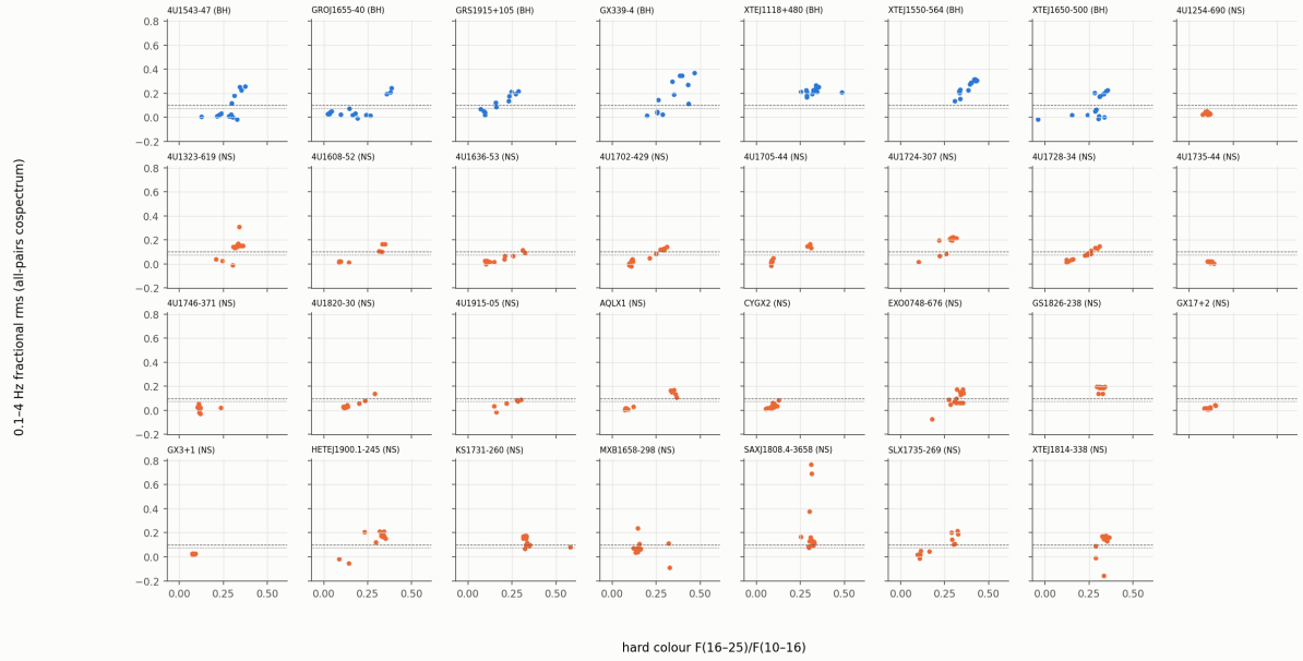
Figure 9.1: The state index (0.1–4 Hz fractional rms, all-pairs cospectrum) against the hard colour for every S1 source (BH blue, NS orange; dashed 0.10 = hard-like threshold, dotted 0.075 = soft-like threshold, RM06 Table 2). XTE J1118+480 and XTE J1550–564 are hard-like throughout; the Z sources Cyg X-2 and GX 17+2 are soft-like; in most sources rms rises with the hard colour. Repo: figures/v7a/v7a_rms_vs_colour_by_source.png , scripts/34_v7a_states.py .
