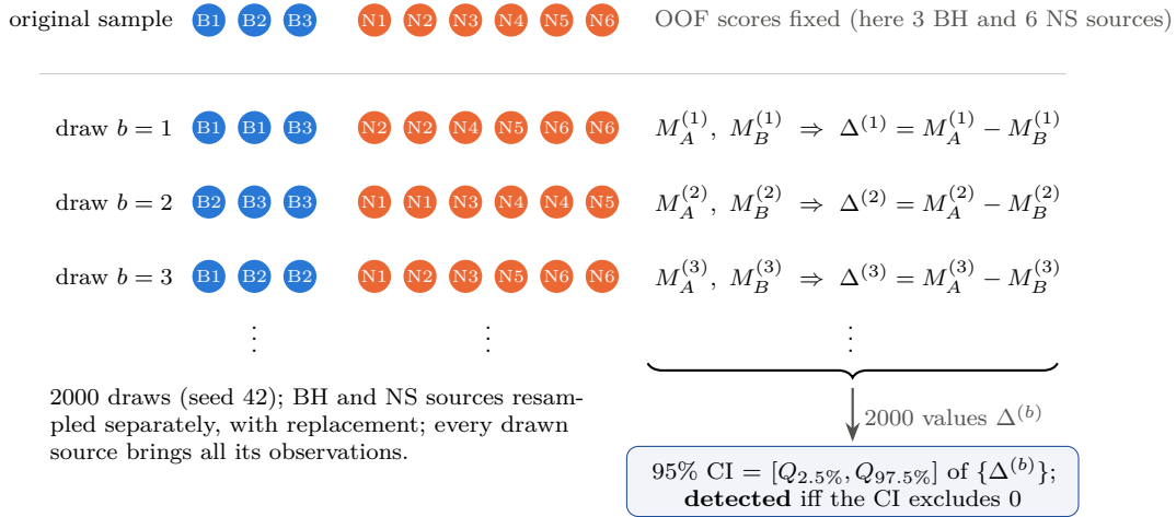
Figure 5.2: Class-stratified source bootstrap with paired differences. Each draw resamples the BH sources and the NS sources separately, with replacement and with all observations of a drawn source; both models are evaluated on the same drawn multiset, so the difference \Delta^{(b)} is paired. No model is refitted. Drawn for this report.
