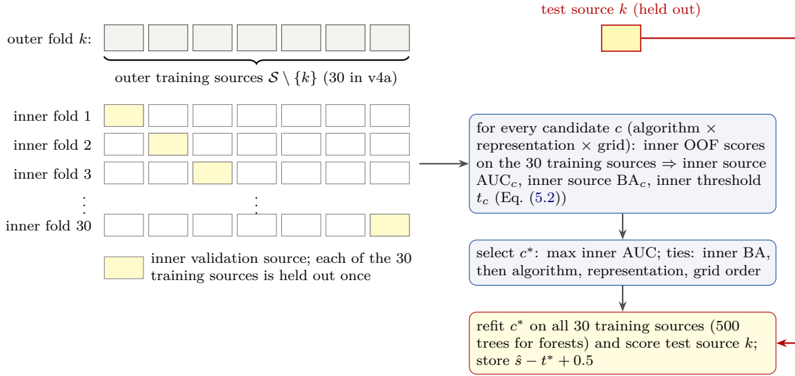
Figure 5.1: Nested LOSO as used in v4a (1d per algorithm and representation; 1e over all 140 configurations). For each outer fold, every candidate configuration is evaluated by an inner LOSO over the outer training sources only; the winner and its inner-optimal threshold are refitted on the outer training sources and applied once to the held-out source. The bias of “choosing the best of many” is therefore included in the outer estimate. Drawn for this report.
