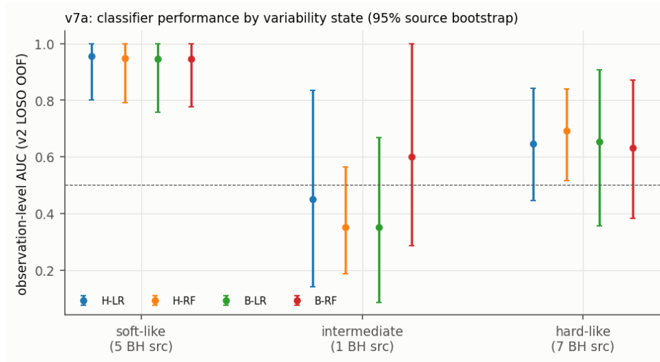
Figure 9.3: Observation-level AUC of the v2 LOSO OOF scores within each variability state (95% source-bootstrap intervals; H-LR, H-RF, B-LR, B-RF). Repo: figures/v7a/v7a_auc_by_state.png , scripts/34_v7a_states.py .
