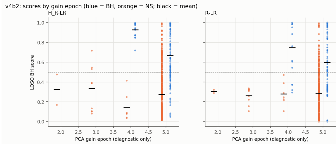
Figure 7.5: LOSO BH scores of the 677 v4b2 observations by PCA gain epoch (diagnostic only; BH blue right of each epoch, NS orange left, black bar = mean). Left: H R -LR; right: R-LR. The epoch-4 BH points are almost all XTE J1859+226; epochs 2–3 contain only a few NS observations of the new sources. Repo: figures/v4b2/v4b2_scores_by_epoch.png , scripts/22_v4b2_analysis.py .
