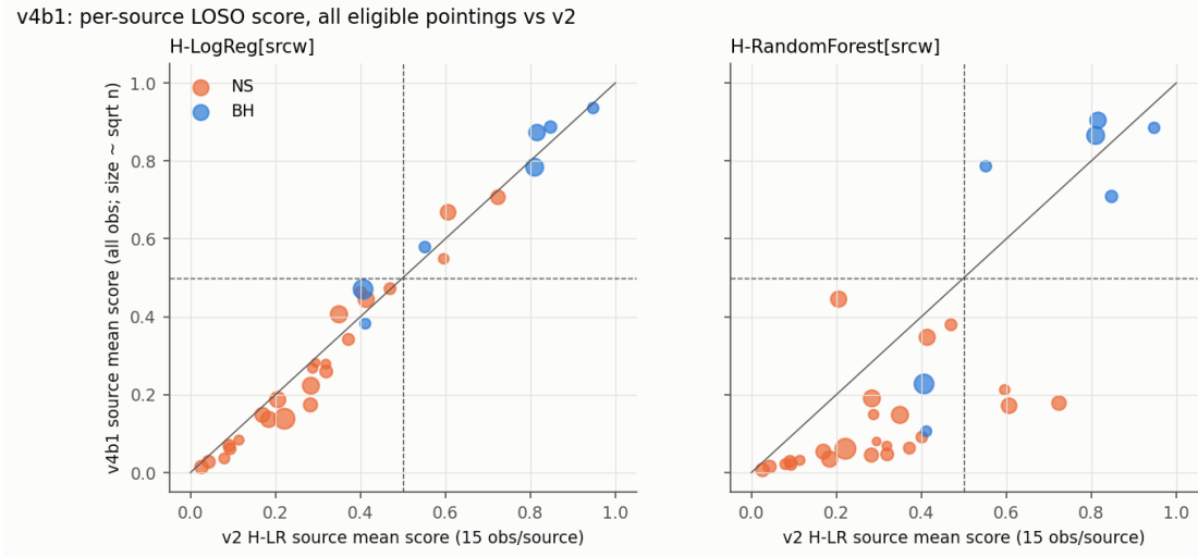
Figure 7.6: Per-source LOSO mean scores with all eligible observations (v4b1, vertical) against the v2 H-LR with 15 observations per source (horizontal); marker size \propto \sqrt{n} , BH blue, NS orange, dashed lines at 0.5. Left: H-LR with source-equal weights – every source stays on the diagonal and in the same quadrant. Right: H-RF with source-equal weights – the forest pushes most NSs to lower scores and moves the NSs that H-LR misclassifies below 0.5, but GRS 1915+105 (large blue circle near 0.23) and XTE J1118+480 stay below 0.5. Repo: figures/v4b1/v4b1_source_scores.png , scripts/25_v4b1_analysis.py .
