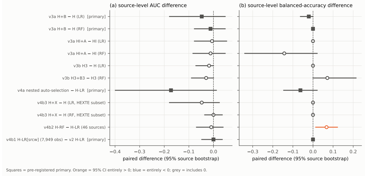
Figure 7.7: Main paired differences of Phases 1–2 against their two-colour baselines with 95% source-bootstrap intervals: (a) source AUC, (b) source balanced accuracy. Rows marked [primary] were the pre-declared primary comparisons of v3a, v4a and v4b1 (the v4b1 main comparison was pre-declared as its main comparison; the pre-registration calls only v4a 1e “primary”). Generated for this report from results/v3/v3a_bootstrap.csv , results/v3/v3b_bootstrap.csv , results/v4/v4a_bootstrap.csv , results/v4b3/v4b3_bootstrap.csv , results/v4b2/v4b2_bootstrap.csv and results/v4b1/v4b1_bootstrap.csv by report_en/figures/generated/make_figures.py ; plotted values in G5_phase12_forest.csv .
