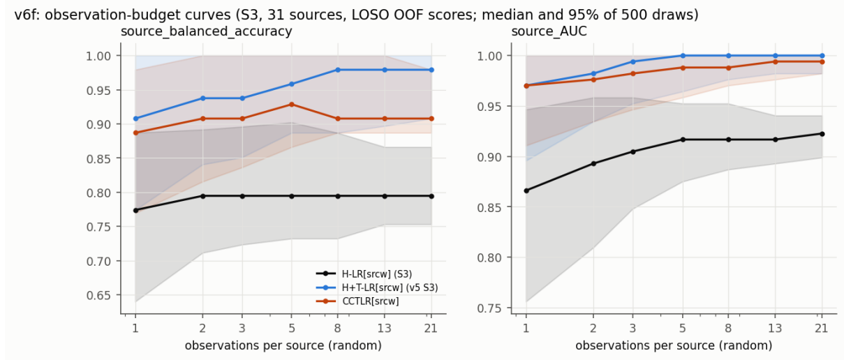
Figure 8.4: Observation-budget curves on S3: source balanced accuracy (left) and source AUC (right) when each source is represented by k randomly drawn observations (LOSO OOF scores of the source-equal-weight models; median and central 95% of 500 draws). Black H-LR, blue H+T-LR, red CCTLR. Repo: figures/v6/v6f_budget_curves.png , scripts/30_v6_analysis.py .
