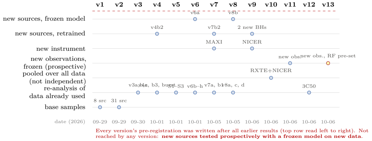
Figure 1.2: What each version adds in terms of independence from data already seen. Rows are ordered from most independent (top) to least; dots mark the sub-analyses of each version. External sources (v6a, v8b) were scored by frozen RXTE models, but few BHs were available (4–7). The NICER versions brought a new instrument and two BHs never used before; v10 pooled everything; v11 and v13 used never-read observations of the same sources with frozen pipelines, v13 with the Random Forest chosen before download (highlighted). Drawn for this report from the pre-registrations and reports/decision_log.md .
