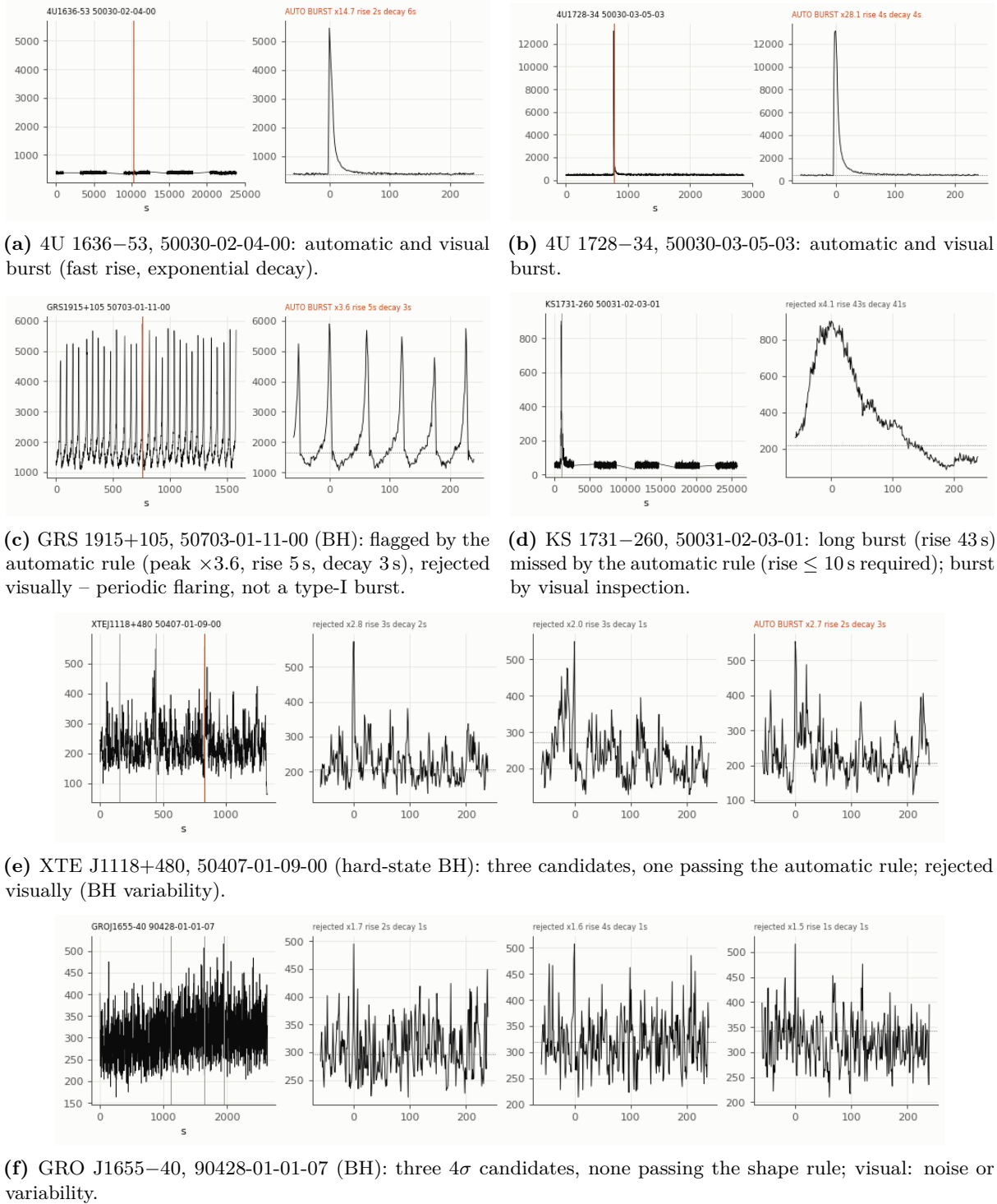
Figure 7.1: Six of the burst-candidate plots, chosen to show each outcome (true positive, BH false positive, missed long burst, rejected candidates). Each plot: left, the whole 1-s Standard-1 light curve of the observation ( \text{counts s}^{-1} summed over the PCUs on; GTI gaps joined by lines; red marks = candidates); then one zoom per candidate with the persistent level (dotted) and the automatic verdict (peak ratio, rise and half-decay times) in its title. Repo: figures/v4/burst_candidates/ (one PNG per observation with candidates), produced by scripts/17_v4_burst_detect.py ; verdicts in results/v4/burst_visual.csv .
