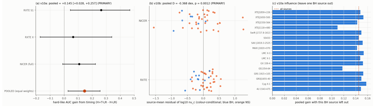
Figure 10.3: v10 pooled tests: (a) hard-like timing gain per component and pooled (red); (b) source-mean residuals of \log_{10} \nu_c at fixed colour per instrument (BH blue, NS orange); (c) pooled gain with each BH source left out (dashed: all sources). Repo: figures/v10/v10_pooled.png , scripts/54_v10_pooled.py .
