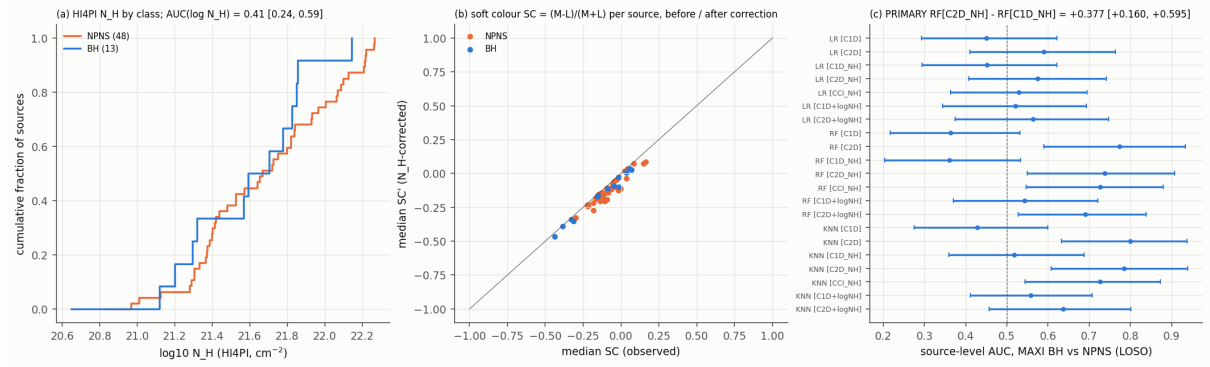
Figure 9.6: v8d: (a) cumulative HI4PI \log N_H of the 13 BHs and 48 NPNS (AUC of \log N_H alone 0.41); (b) per-source median soft colour SC before and after the correction; (c) source AUC of all model/feature combinations (95% source-bootstrap intervals). Repo: figures/v8d/v8d_nh_control.png , scripts/45_v8d_nh.py .
