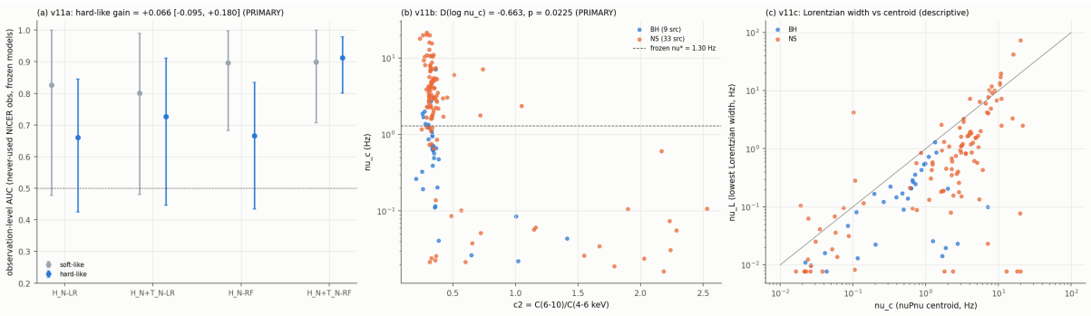
Figure 11.1: v11 on new observations: (a) observation-level AUC by state of the frozen models; (b) \nu_c against c_2 for the new hard-like observations (BH blue, 9 sources; NS orange, 33) with the frozen \nu^* = 1.30 \text{ Hz} ; note the very hard ( c_2 > 0.5 ), very low- \nu_c points discussed in the text; (c) lowest Lorentzian width \nu_L against \nu_c (v11c). Repo: figures/v11/v11_prospective.png , scripts/57_v11_analysis.py .
