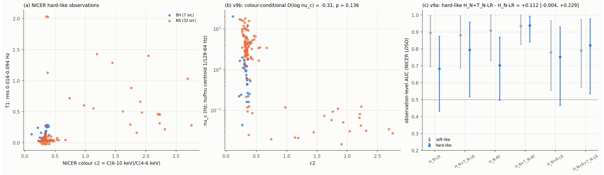
Figure 10.1: NICER hard-like observations (BH blue, 7 sources; NS orange, 32 sources): (a) T1 rms against the colour c_2 = C(6-10)/C(4-6) ; (b) \nu_c against c_2 – at c_2 \approx 0.2-0.4 the BHs lie at lower \nu_c , and the very hard NS observations ( c_2 > 0.7 ) have very low \nu_c ; (c) observation-level AUC by state for the v9a models. Repo: figures/v9/v9_nicer.png , scripts/49_v9_analysis.py .
