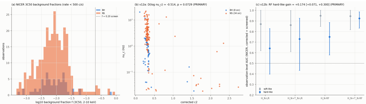
Figure 11.2: v12: (a) 3C50 background fractions of the faint ( < 500 \text{ cs}^{-1} ) observations with the f = 0.20 screen; (b) \nu_c against the corrected c_2 (8 BH, 34 NS sources); (c) AUC by state after correction and screening. Repo: figures/v12/v12_background.png , scripts/59_v12_analysis.py .
