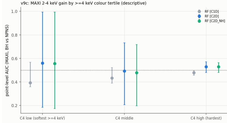
Figure 9.7: v9c (pre-declared, descriptive): point-level AUC of RF on C1D, C2D and C2D NH within tertiles of the \geq 4 keV colour C4 (95% source-bootstrap intervals). The point-level metric is dominated by the sources with most points, which is why all values are near 0.5; the source-level version is in Table 9.21. Repo: figures/v9/v9c_maxi_c4_strata.png , scripts/50_v9c_maxi_strata.py .
