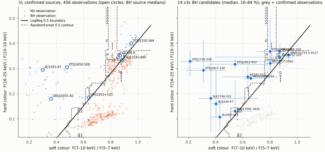
Figure 6.10: The two count-space colours of H: soft F(7–10)/F(5–7) (x) and hard F(16–25)/F(10–16) (y). Left: 456 observations of the 31 confirmed sources (orange NS, blue BH; open circles = BH source medians), the LR 0.5 boundary (solid) and the RF 0.5 contour (dashed), both fitted on all sources for illustration only. Right: the 14 v3c candidates (median and 16–84% range) on the confirmed observations (grey). Look at the upper-right end of the NS track: hard BHs and hard NSs overlap there, which is where every spectral model errs and where Phases 3–6 look for timing information. Repo: figures/final/colour_colour_decision_boundary.png ; script scripts/15_colour_colour.py .
