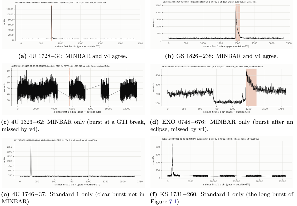
Figure 9.2: MINBAR versus the v4 Standard-1 burst detector: 1-s Standard-1 light curves ( \text{counts s}^{-1} , time since the first bin; gaps are outside the GTIs) with MINBAR burst intervals shaded; the title states the MINBAR match and the v4 automatic and visual verdicts. Repo: figures/v7b1/ (one PNG per agreeing or disagreeing observation), scripts/31_v7b1_minbar.py .
