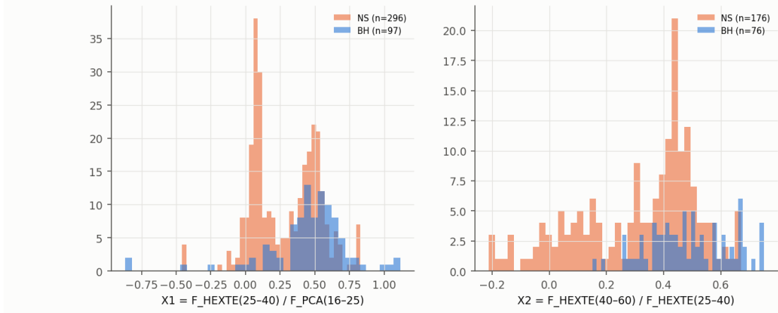
Figure 7.2: HEXTE cluster-B colours (Eq. (7.1)) of the v2 observations with valid values, BH blue, NS orange. Left: X_1 (393 observations: 97 BH, 296 NS); right: X_2 (252 observations: 76 BH, 176 NS). The NS X_1 distribution is bimodal (soft states near 0, hard states near 0.5); the BHs lie mostly in the hard NS mode, and the X_2 distributions overlap. Repo: figures/v4b3/v4b3_hexte_colours.png , scripts/19_v4b3_hexte.py ; values in data/v4b3/processed/hexte_features.csv .
