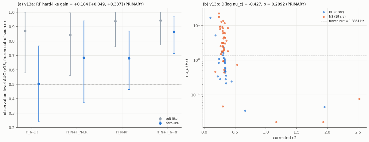
Figure 11.3: v13 on a third set of new observations with the frozen v12 pipeline: (a) AUC by state of the frozen out-of-source models; (b) \nu_c against the corrected c_2 with \nu^* = 1.3361 Hz – at c_2 \approx 0.3 the BHs lie mostly below the NSs. Repo: figures/v13/v13_prospective.png , scripts/63_v13_analysis.py .
