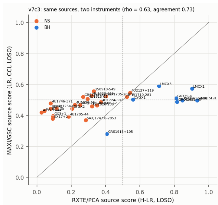
Figure 9.5: RXTE/PCA H-LR source score (horizontal) against MAXI/GSC LR (CCI) source score (vertical) for the 30 common sources (BH blue, NS orange; dashed lines at 0.5). Repo: figures/v7c/v7c3_rxte_vs_maxi.png , scripts/39_v7c2_analysis.py .
