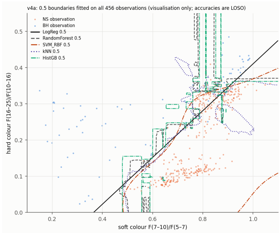
Figure 7.4: 0.5 decision boundaries in the H colour plane (soft colour F(7-10)/F(5-7) , hard colour F(16-25)/F(10-16) , count space) of LR, RF, SVM-RBF, kNN and HistGB fitted on all 456 v2 observations (blue BH, orange NS). Visualisation only; all accuracies in this chapter are LOSO. Repo: figures/v4/v4a_colour_boundaries.png , scripts/16_v4a_algorithms.py .
