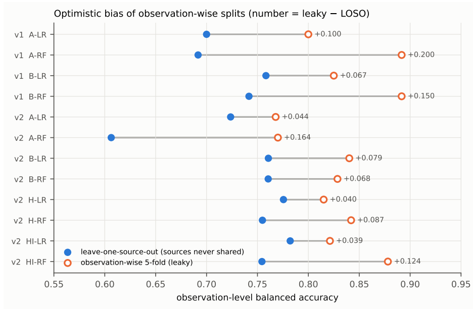
Figure 1.1: Optimism of observation-wise cross-validation. For every representation and model of v1 (8 sources) and v2 (31 sources), observation-level balanced accuracy under leave-one-source-out (filled blue) and under a stratified 5-fold split over observations in which sources appear in both training and test folds (open orange); the number is the difference. The leaky split is optimistic in every case (+0.04 to +0.20), most for models that can memorise intensity (A-RF). Generated for this report from results/metrics_observation_level.csv , results/secondary_observation_split.csv and their results/v2/ counterparts ( report_en/figures/generated/make_figures.py ; values in G4_leakage.csv ).
