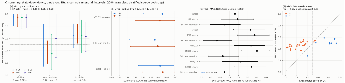
Figure 9.8: v7 summary: (a) AUC by variability state for four models; (b) source AUC of H-LR and H-RF with 31 sources, with 34 sources evaluated on the 31, and on all 34; (c) MAXI source AUC of all models and feature sets (dashed: RXTE v2 H-LR); (d) RXTE vs MAXI source scores of the 30 common sources. Repo: figures/v7/v7_summary.png , scripts/40_v7_summary_figure.py .
