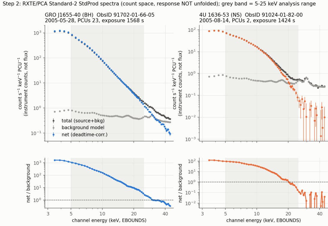
Figure 2.1: Data-flow validation on one BH (GRO J1655–40, ObsID 91702-01-66-05) and one NS (4U 1636–53, ObsID 91024-01-82-00). Top: total (dark grey), background model (light grey) and deadtime-corrected net (colour) count rates per keV per PCU against channel energy (EBOUNDS), log-log; the grey band is the 5–25 keV analysis range. Bottom: net/background ratio. The point is that the net spectrum is background-dominated only above \sim 30 keV for these bright sources, and that everything is in instrument count space (no response unfolding). Repo: figures/step2_two_sources.png , script scripts/05_two_source_check.py .
