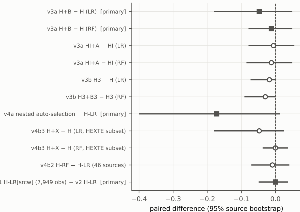
(a) source-level AUC difference
