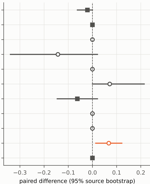
(b) source-level balanced-accuracy difference
