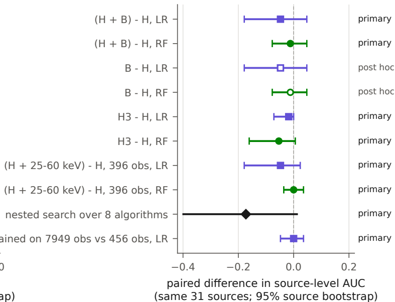
(a) RXTE/PCA development sample, LOSO
