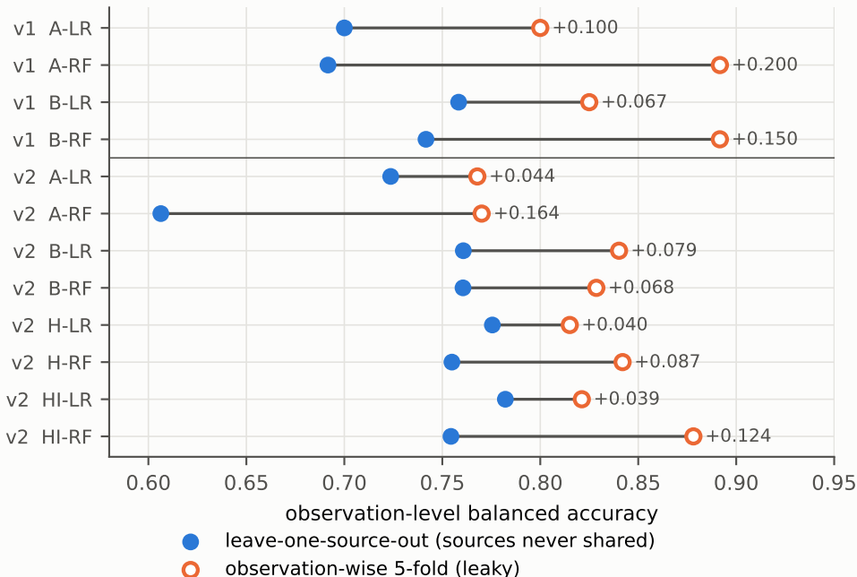
Optimistic bias of observation-wise splits (number = leaky – LOSO)
