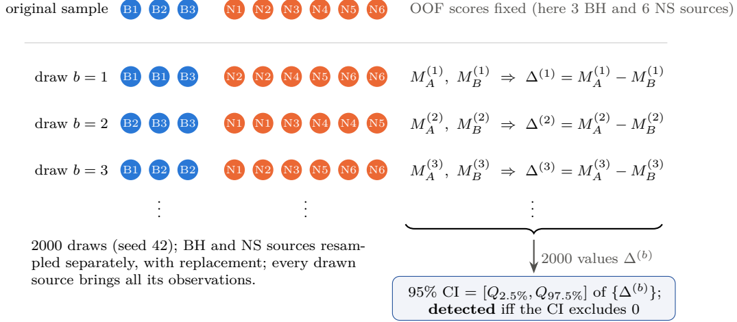
Figure 5.2: Class-stratified source bootstrap with paired differences. Each draw resamples the BH sources and the NS sources separately, with replacement and with all observations of a drawn source; both models are evaluated on the same drawn multiset, so the difference \Delta^{(b)} is paired. No model is refitted. Drawn for this report.
