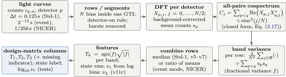
Figure 2.4: Timing-feature pipeline shared by RXTE Standard-1 (v5–v10), RXTE event mode (v8c) and NICER (v9–v13). Differences between the instruments are in the bin width, the segment length, the “detector” (PCU or NICER MPU), whether rows are combined by the median or by the ratio of means, and the frequency bands (Table 2.6). Drawn for this report.
