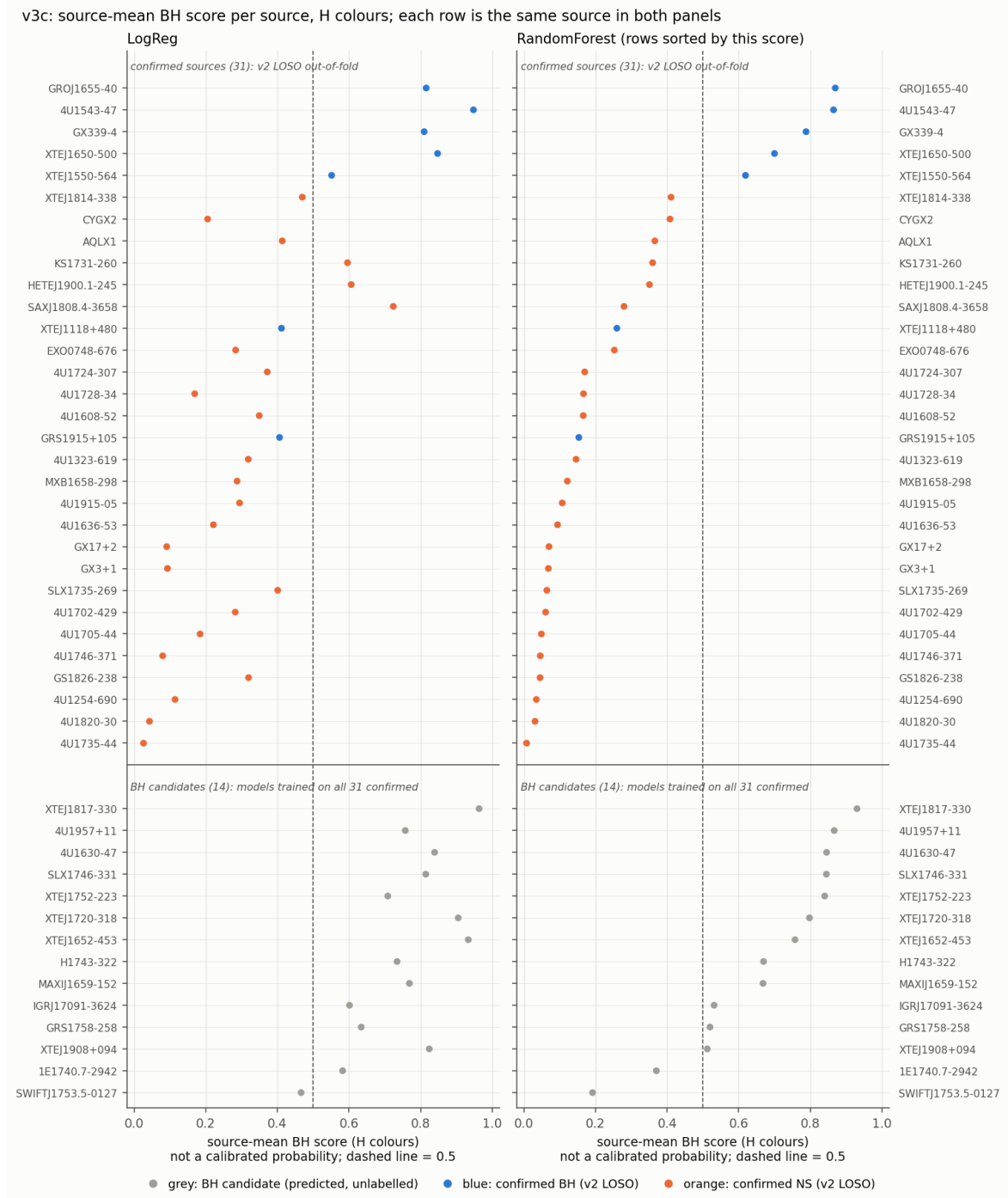
Figure 6.9: v3c with H: LOSO source means of the 31 confirmed sources (blue BH, orange NS, top block) and source-mean BH scores of the 14 candidates (grey, predicted, bottom block), LR left, RF right; each row is the same source in both panels, sorted within each block by the RF score; dashed = 0.5. Most candidates sit with the confirmed BHs; Swift J1753.5–0127 sits with the NSs (0.47 LR, 0.19 RF), and 1E 1740.7–2942 is also below 0.5 for RF (0.37; results/v3/v3c_candidate_source_summary.csv ). Repo: figures/v3/v3c_candidate_scores.png , drawn from the saved predictions by scripts/v3c_plot.py ( scripts/14_v3c_candidates.py --plot-only ); this version replaces an earlier one whose LR panel had mismatched source labels.
