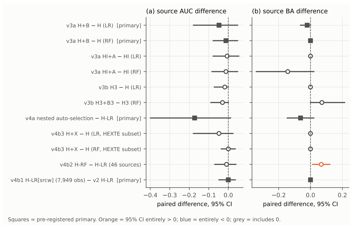
Figure 7.7: Main paired differences of Phases 1–2 against their two-colour baselines with 95% source-bootstrap intervals: (a) source AUC, (b) source balanced accuracy. Rows marked [primary] were the pre-declared primary comparisons of v3a, v4a and v4b1 (the v4b1 main comparison was pre-declared as its main comparison; the pre-registration calls only v4a 1e “primary”). Generated for this report from results/v3/v3a_bootstrap.csv , results/v3/v3b_bootstrap.csv , results/v4/v4a_bootstrap.csv , results/v4b3/v4b3_bootstrap.csv , results/v4b2/v4b2_bootstrap.csv and results/v4b1/v4b1_bootstrap.csv by report_en/figures/generated/make_figures.py ; plotted values in G5_phase12_forest.csv .
