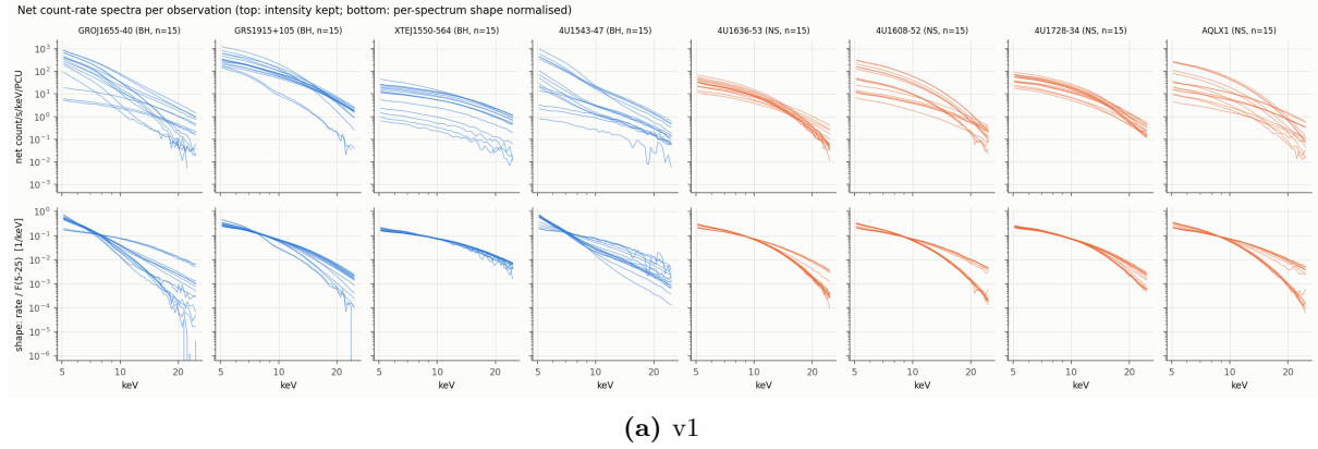
Figure 6.2: Net count-rate spectra of every accepted observation, one panel pair per source (upper: count rate per keV per PCU, log-log, non-positive bins omitted; lower: per-spectrum shape normalised to the 5–25 keV rate). The spread within a source (state changes) is comparable to the spread between sources, which is why a single observation is a hard input. Repo: figures/step3_spectra_by_source.png , figures/v2/step3_spectra_by_source.png ; script scripts/06_dataset_checks.py . Panel (b), v2, is in the continuation of this figure.
