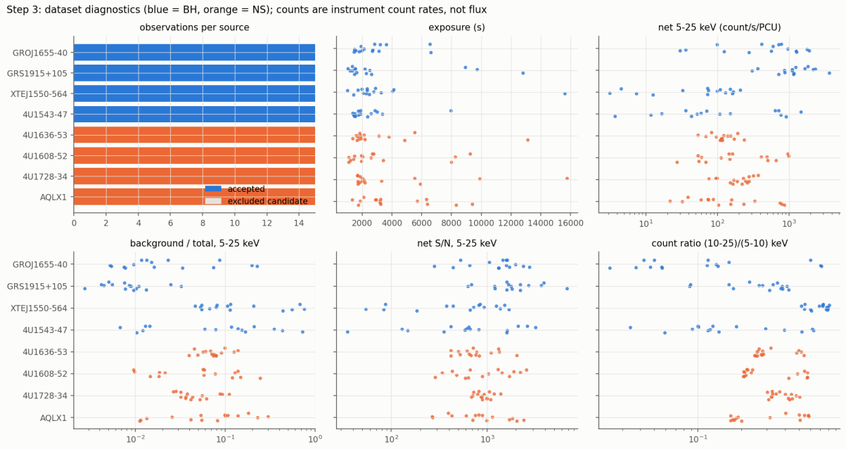
(a) v1, 8 sources
