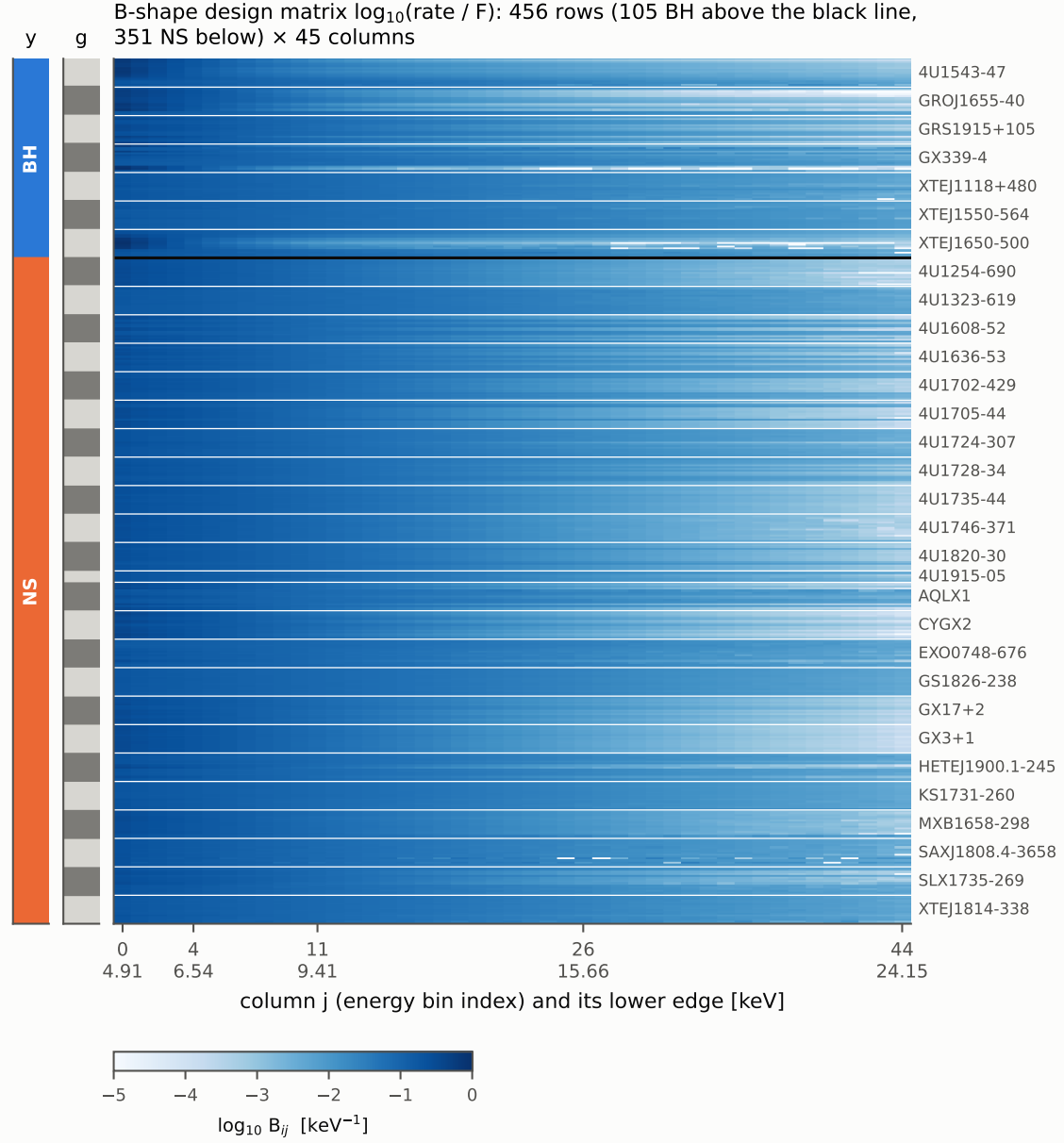
Figure 3.1: The real v2 design matrix for representation B: 456 rows (observations) \times 45 columns (energy bins), colour = \log_{10} B_{ij} (sequential scale, darker = larger). Rows are grouped by source (right labels; alternating grey in strip g ), BH sources first (strip y : blue = 1) and NS below the black line (orange = 0). The steep fall of the shape with energy dominates every row; differences between sources are subtle and mostly in the high-energy columns, consistent with the finding that two colours capture the usable information. Generated for this report from data/v2/processed/features.npz .
