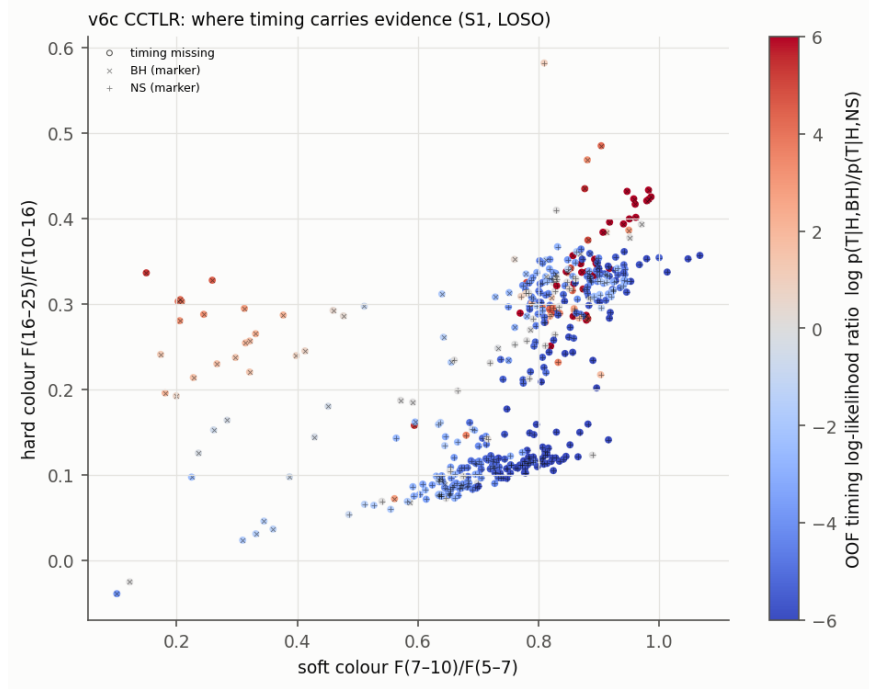
Figure 8.3: Where the timing features carry evidence: each S1 observation in the colour plane, coloured by its out-of-fold CCTL timing log-likelihood ratio \Lambda = \log p(\mathbf{T} \mid \mathbf{h}, \text{BH}) / p(\mathbf{T} \mid \mathbf{h}, \text{NS}) (red BH-like, blue NS-like, clipped at \pm 6 ); \times = BH, + = NS markers, grey open circles = timing missing ( \Lambda = 0 ). The hard-state corner (hard colour \gtrsim 0.35 ) and the soft BH region at low soft colour are red; the NS banana branch at hard colour \approx 0.1 is blue. Repo: figures/v6/v6c_timing_evidence_map.png , scripts/30_v6_analysis.py .
