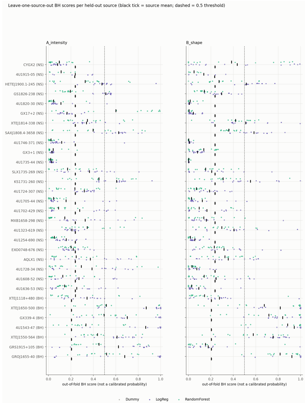
Figure 6.6: v2: out-of-fold BH score of every observation of each held-out source (left: A, right: B; grey Dummy, purple LR, green RF), black tick = source mean, dashed = 0.5. The BH sources (bottom seven) are spread over the whole score range; XTE J1118+480 and GRS 1915+105 are below 0.5 for B. Repo: figures/v2/step4_loso_scores.png ; script scripts/07_train_eval.py (XRB_VERSION=v2).
