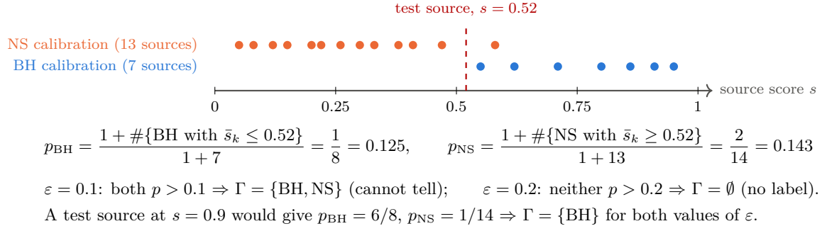
Figure 5.3: Illustration (made-up calibration scores) of the class-conditional conformal p -values of Eq. (5.9). A test source is compared with the calibration sources of each class separately; a label enters the prediction set if the test source is not too atypical for that class. Drawn for this report.
