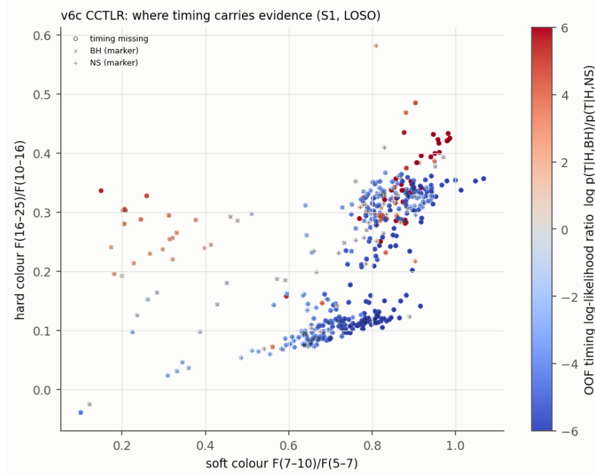
Figure 8.3: Where the timing features carry evidence: each S1 observation in the colour plane, coloured by its out-of-fold CCTLR timing log-likelihood ratio \Lambda = \log p(\mathbf{T} | \mathbf{h}, \text{BH}) / p(\mathbf{T} | \mathbf{h}, \text{NS}) (red BH-like, blue NS-like, clipped at \pm 6 ); \times = BH, + = NS markers, grey open circles = timing missing ( \Lambda = 0 ). The hard-state corner (hard colour \gtrsim 0.35 ) and the soft BH region at low soft colour are red; the NS banana branch at hard colour \approx 0.1 is blue. Repo: figures/v6/v6c_timing_evidence_map.png , scripts/30_v6_analysis.py .
