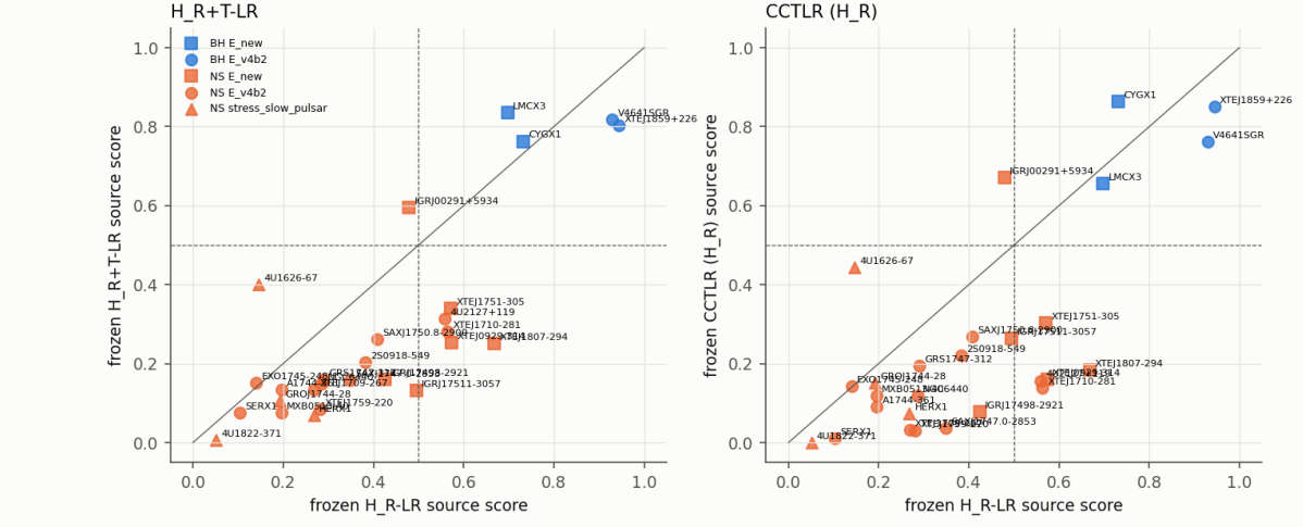
v6a: external sources never used in training (models frozen on the 31 v2 sources); ^ = slow-pulsar stress set
