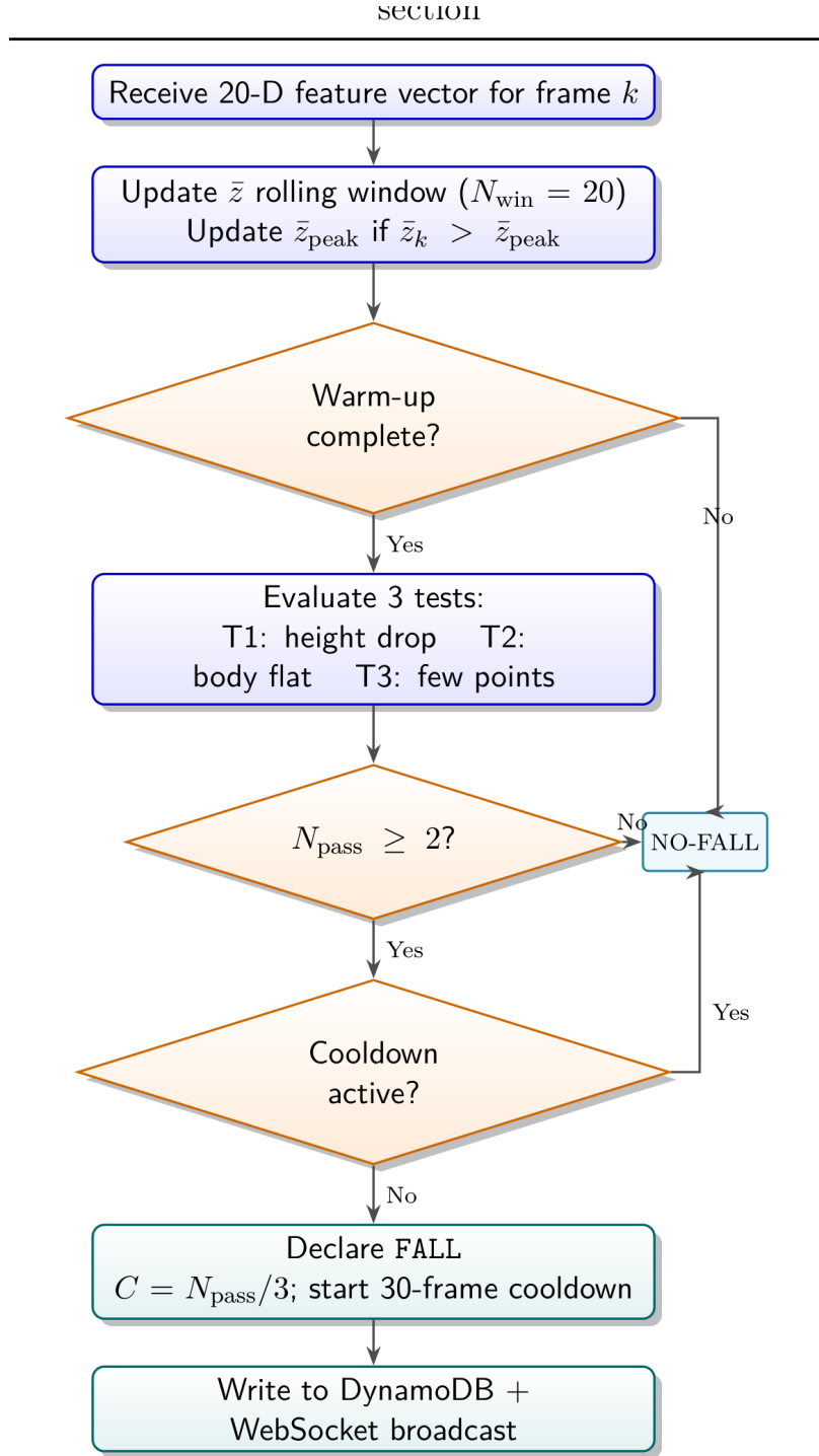
Figure 5.1: StreamingFallDetector per-frame decision flow. All frames k are processed sequentially.
