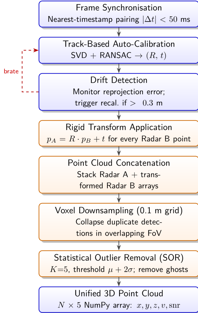
dual-radar fusion pipeline with auto-recalibration
