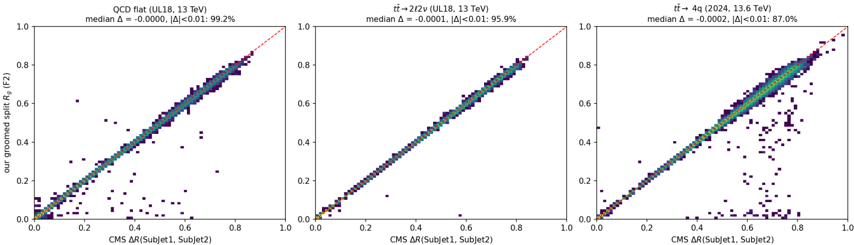
R_g exact match: our soft-drop split angle vs CMS's stored subjet pair — jet-by-jet
