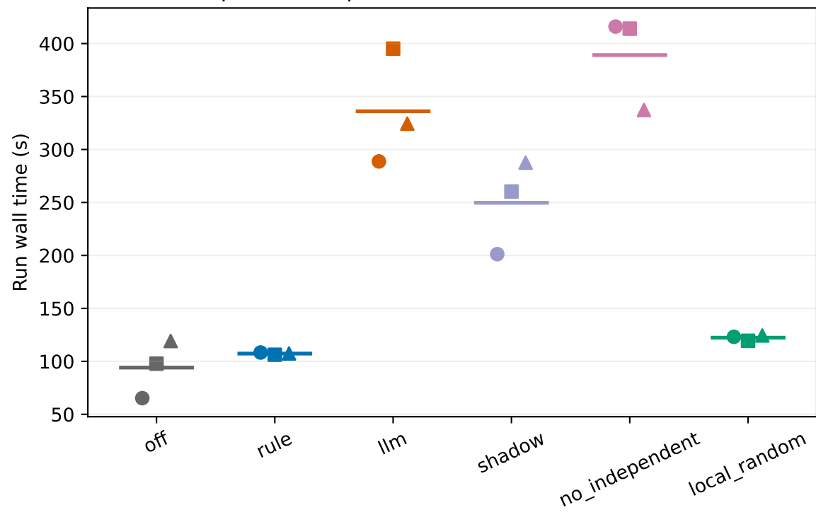
Main32: points = repeats; line = mean of available values
