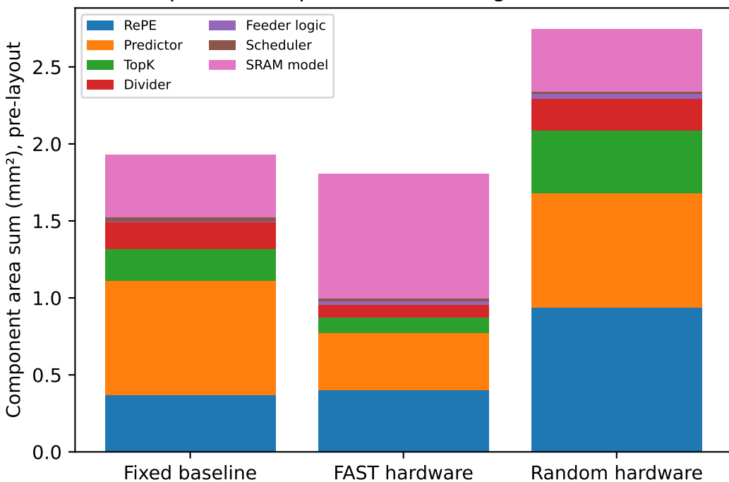
Separate components; not integrated die area
