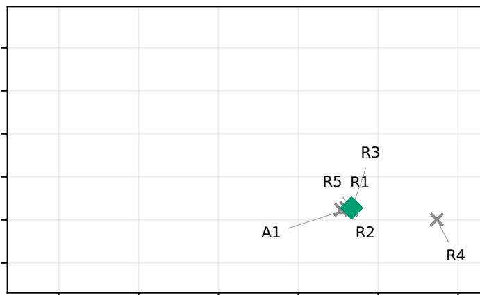
Global Top-K
