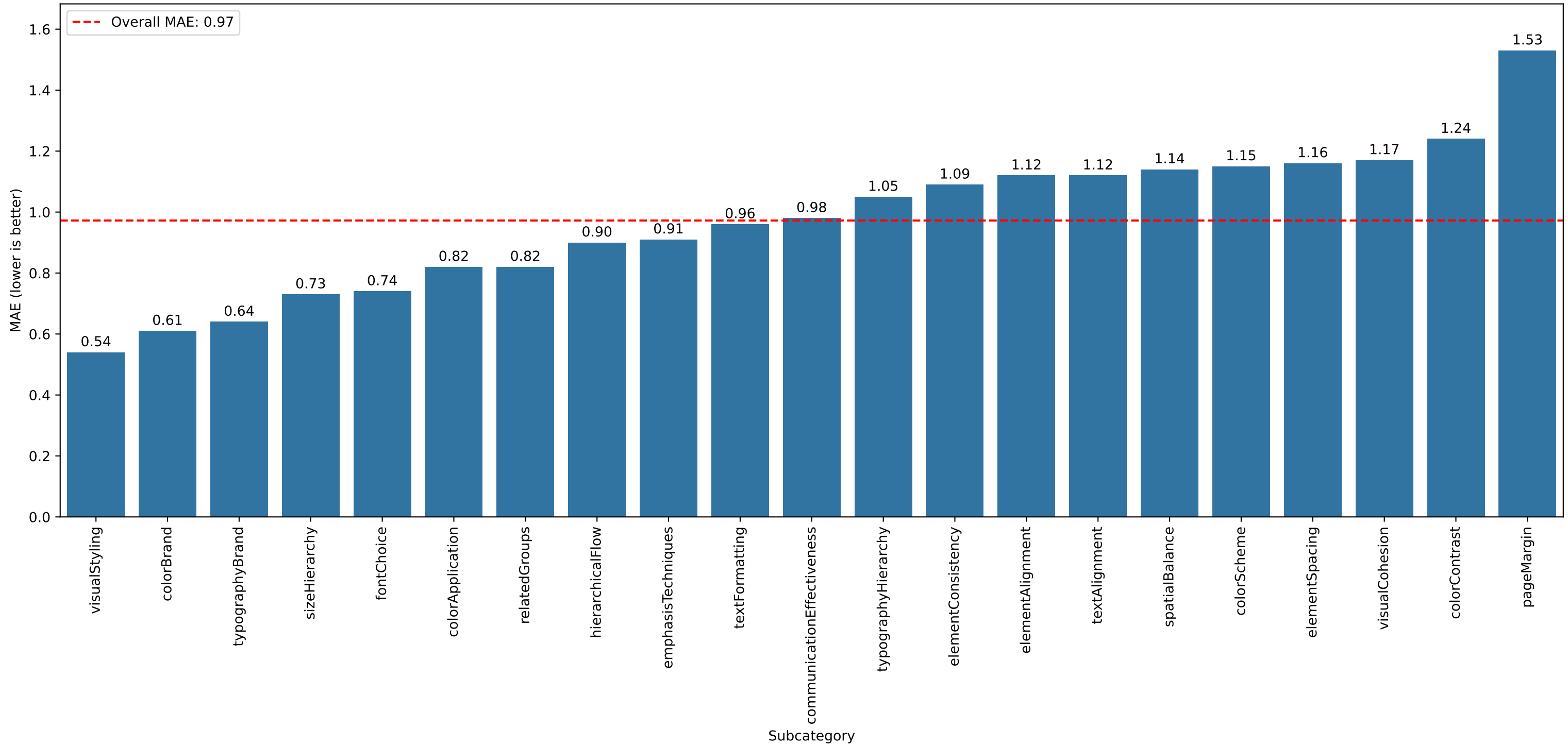
Mean Absolute Error by Subcategory: gemma-3-12b-it-unsloth-bnb-4bit
